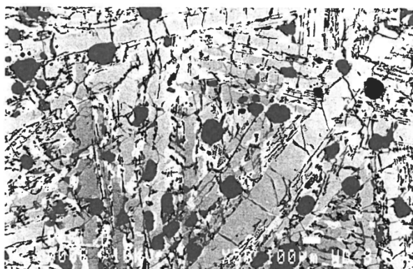
Fig. 27: Sample of a 58% ferro-silicon treated at 600°C for 12 h. HT-FeSi 2 is grey, LT-FeSi 2 is white and Si-precipitates are black (Bjorndal, 1990)
