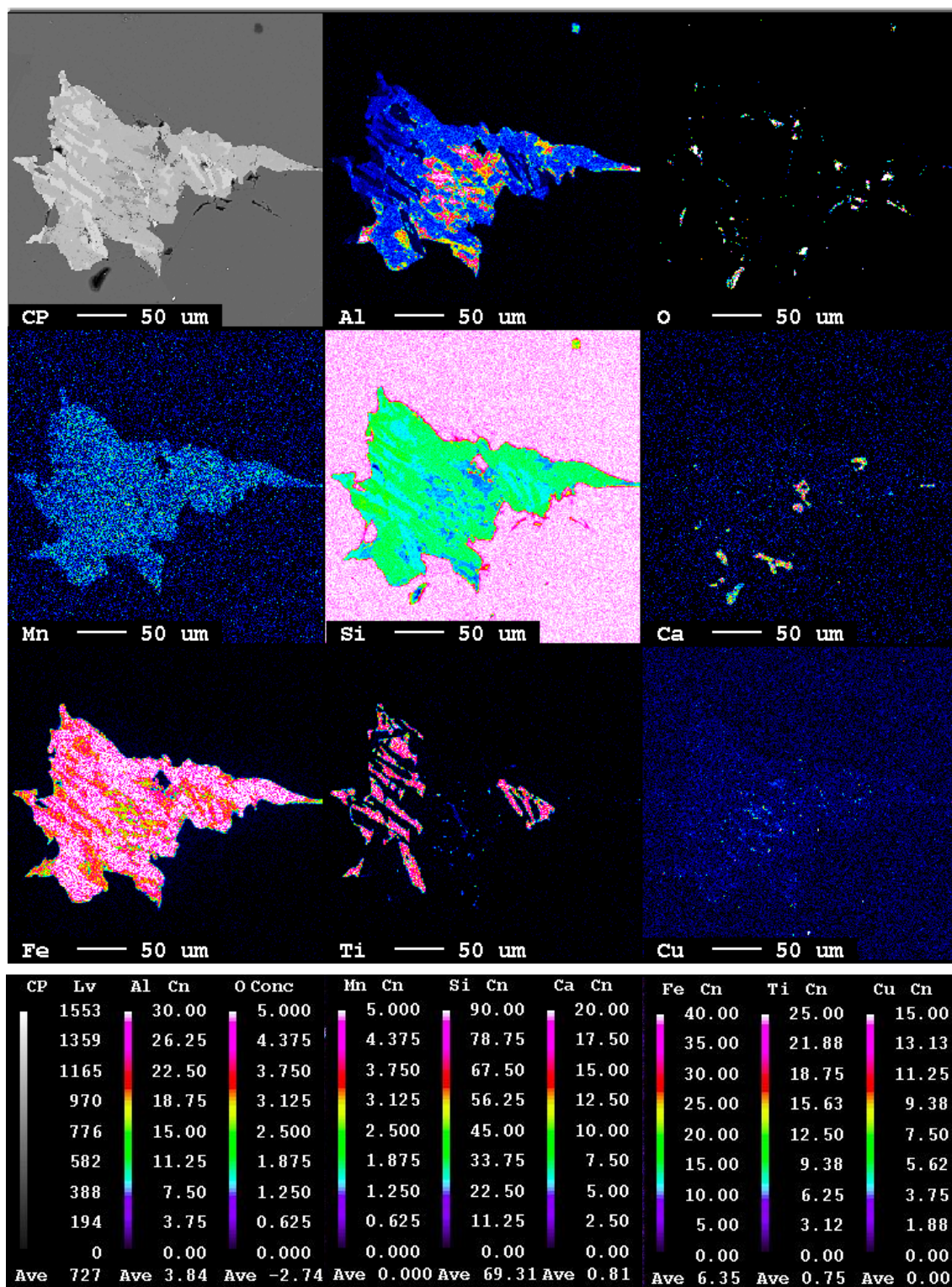
Fig. 69: Mapping of an intermetallic particle from the sample annealed at 1200°C
