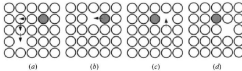
Fig. 7: Vacancy mechanism for substitutional diffusion
