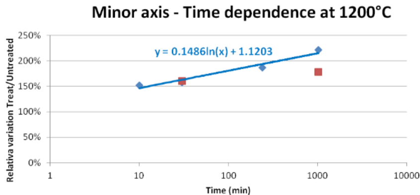
Fig. 61: Time dependence of relative variation of minor axis at 1200°C
