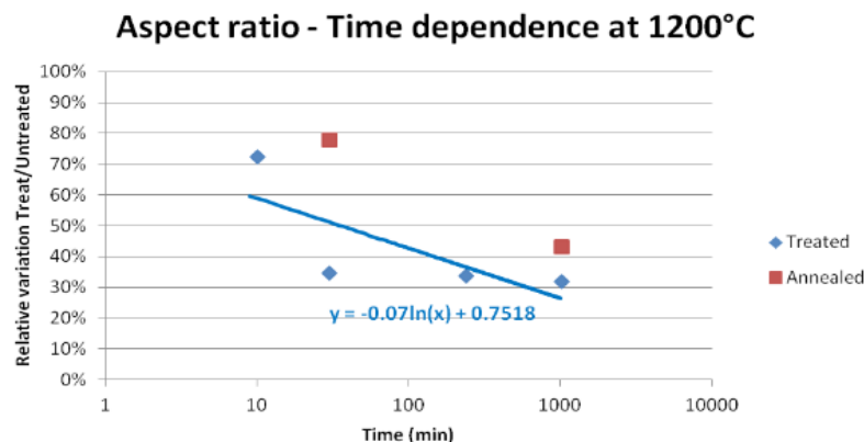
Fig. 41: Time dependence of relative variation of aspect ratio at 1200°C
