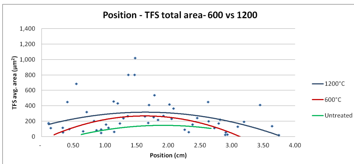
Fig. 80: Relation between position and sum of TFS particles area. Focus on similarity between 600°C ad untreated (a) and comparison with the annealed sample (b)
