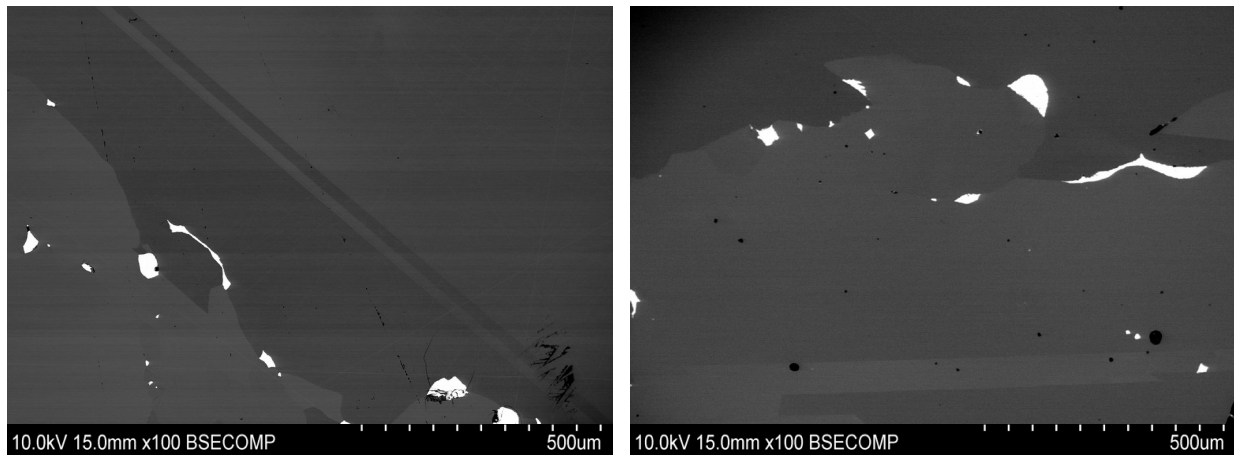
Fig. 36: Remolten treated sample (left) and heat treated sample microstructure (right). The pictures are taken respectively from the bottom and from the solidification front meeting point, which are the zones where the highest changes in microstructure occur compared to the respective reference
