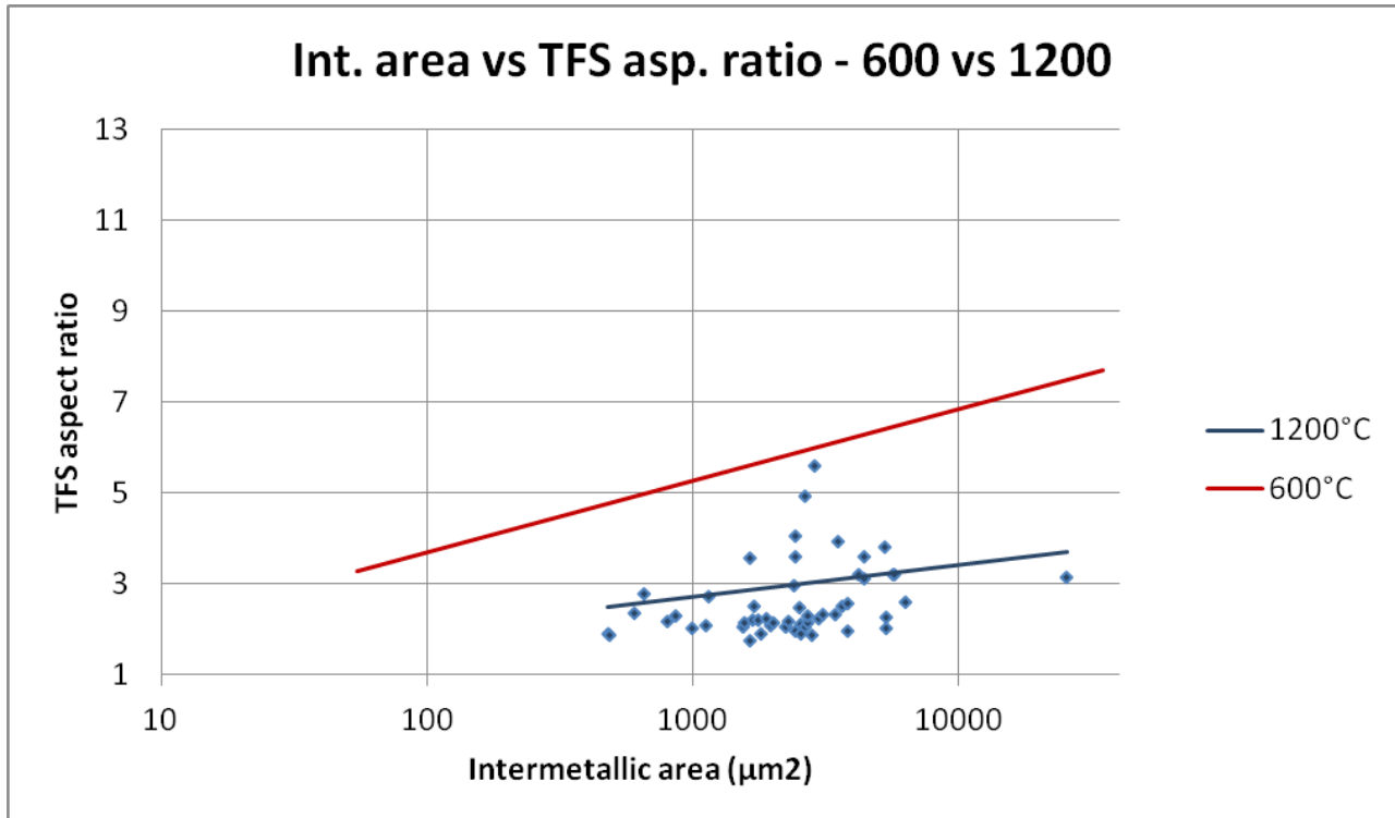
Fig. 81: Relation between hosting intermetallic area and average TFS particle aspect ratio. Focus on similarity between 600°C ad untreated (a) and comparison with the annealed sample (b)
