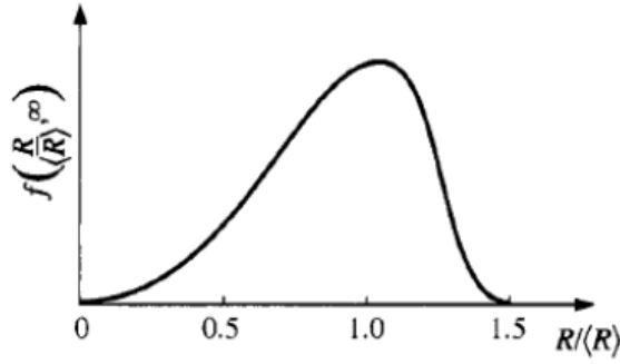
Fig. 18: Final steady-state normalized PSD for diffusion-limited coarsening
