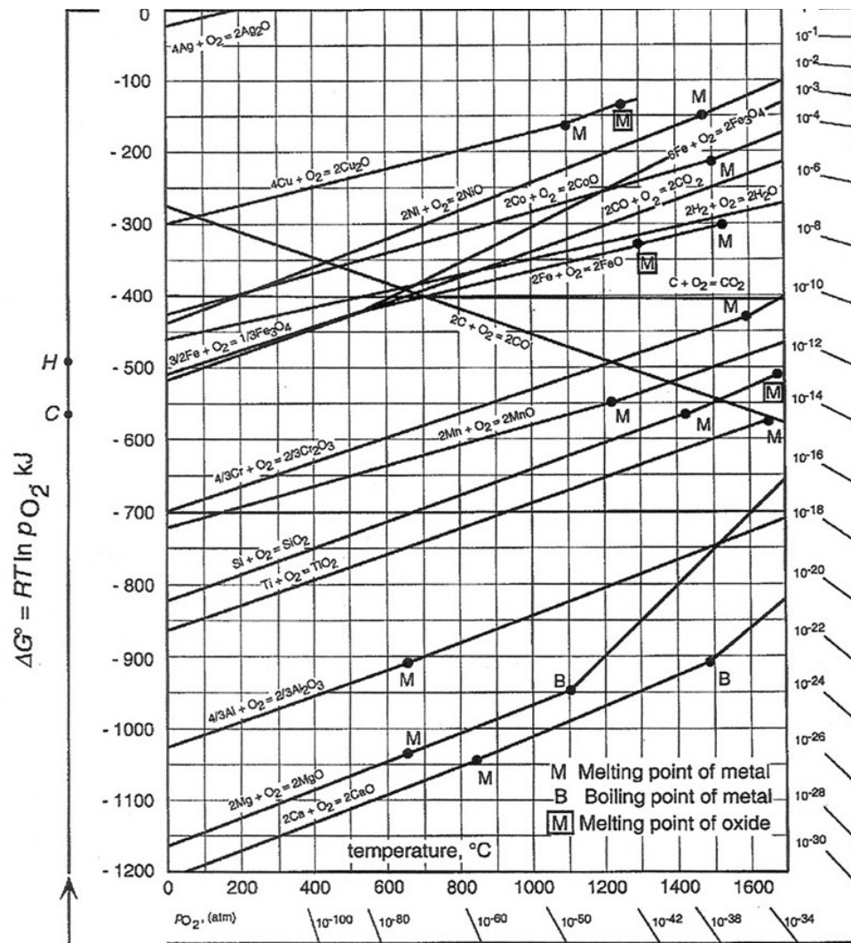
Fig. 3: Ellingham diagram for different oxides (Gaskell, 2010)
