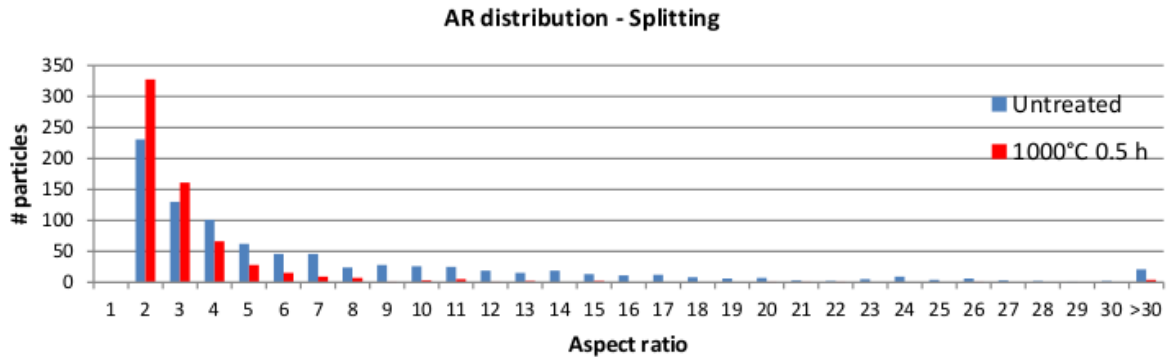
Fig. 42: Distribution of AR values in a sample treated for short times, which shows splitting (compared to the related untreated surface)
