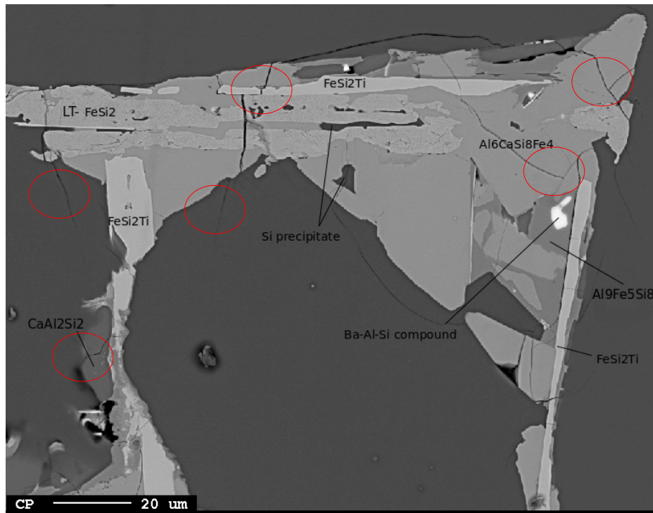
Fig. 77: Cracks in intermetallic going through silicon, \text{FeSi}_2 , Al-Fe-Si phases and \text{Al}_6\text{CaFe}_4\text{Si}_8 , but in most cases not through \text{TiFeSi}_2 . Picture from sample treated at 600^\circ\text{C}
