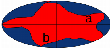
Fig. 39: Definition of aspect ratio: a and b are respectively the major and the minor axis of the ellipse (blue) circumscribed to a particle (red). Therefore AR=b/a
