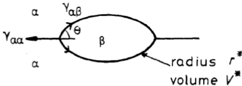
Fig. 20: Thermodynamic model of precipitation of particles at the grain boundary. r^* and V^* are the critical nucleus radius and volume
