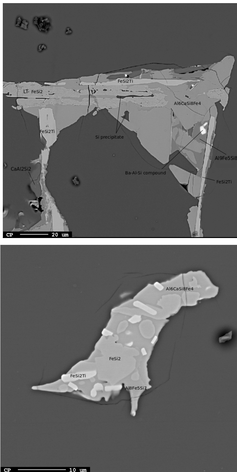
Fig. 66: Two particles coming respectively from the solidification fronts meeting point (A) and from the bottom (B) of the treated sample at 600°C
