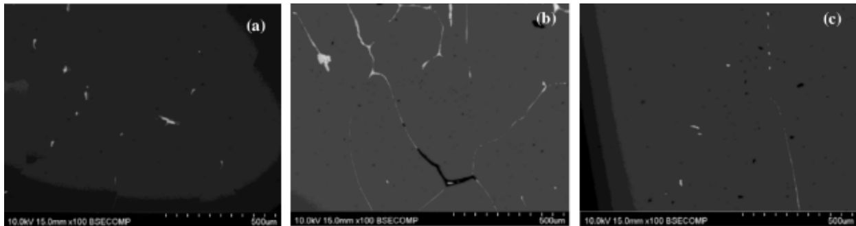
Fig. 34: Untreated sample microstructures at bottom (a), center (b) and top (c) of the cast
