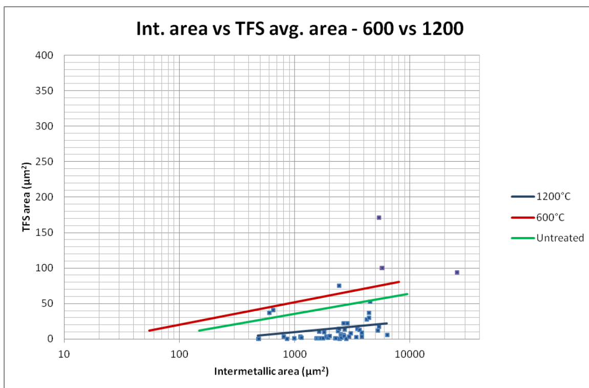
Fig. 82: Relation between hosting intermetallic area and average TFS particle area. Focus on similarity between 600°C ad untreated (a) and comparison with the annealed sample (b)
