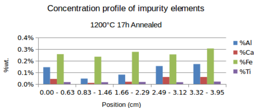
Fig. 71: XRF analysis as a function of position for the annealed sample at 1200°C. The position 0.00 corresponds to the cast bottom., and 3.95 to the interface between slag and silicon
