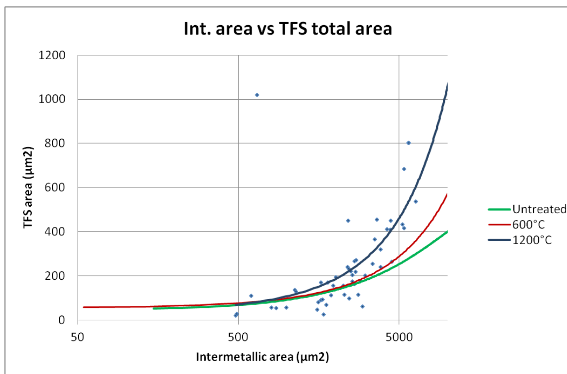
Fig. 79: Relation between hosting intermetallic area sum of TFS particles area. Focus on similarity between 600°C ad untreated (a) and comparison with the annealed sample (b)
