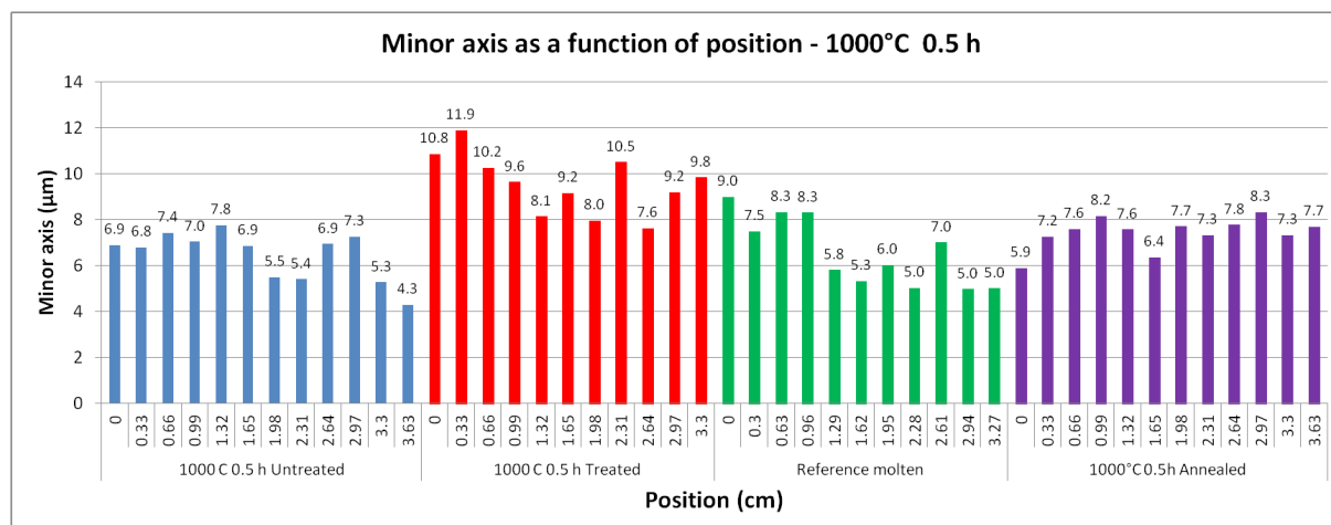
Fig. 62: Minor axis as a function of position in samples showing splitting, compared to their relative references
