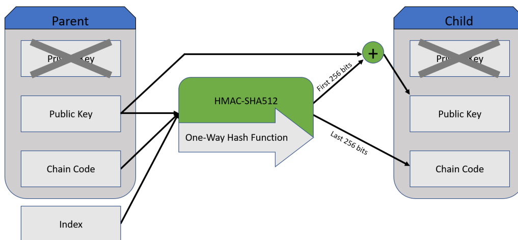
FIGURE 3.4: Public Derivation
