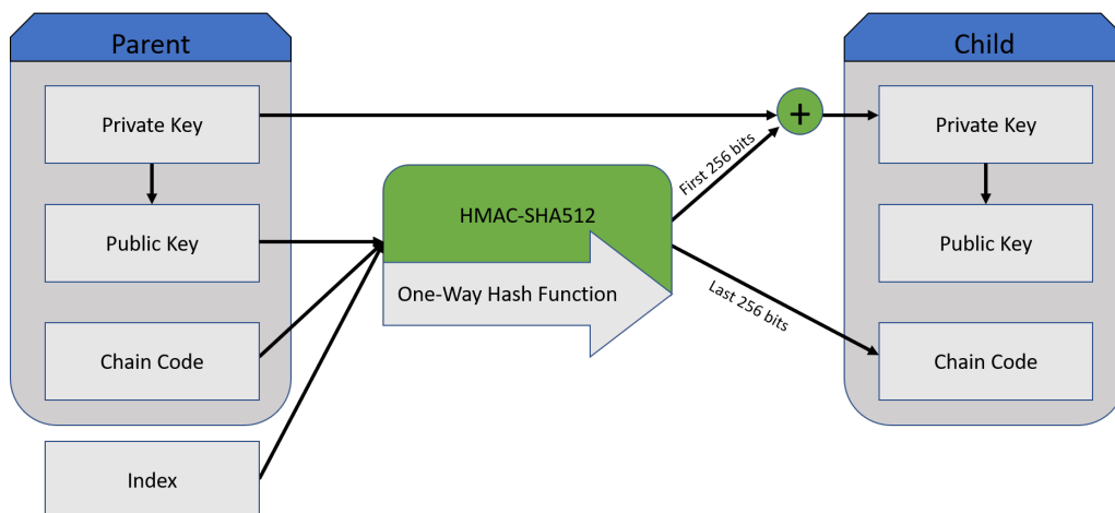
FIGURE 3.2: Normal Derivation
