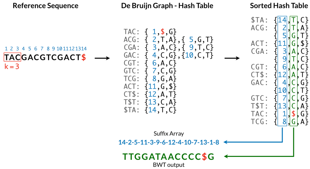
Figure 5.4: Optimized BWT and suffix array computation via de Bruijn graph
