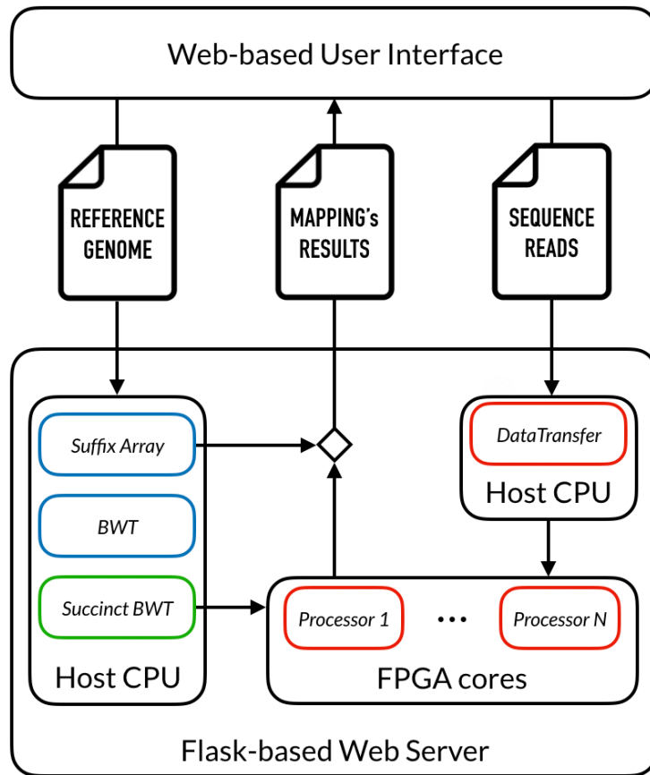
Figure 5.1: Outline of the proposed sequence mapper
