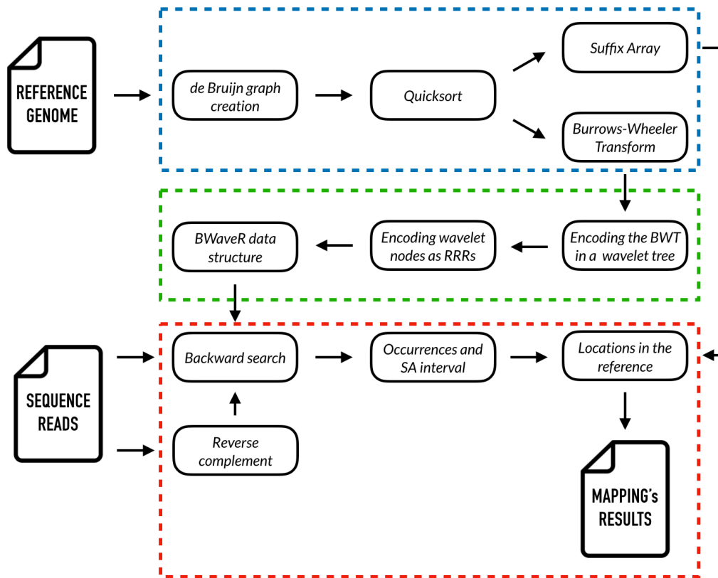
Figure 5.2: BWaveR sequence mapper: overall work-flow
