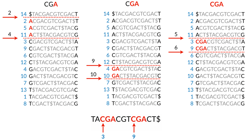
Figure 3.2: The backward pattern matching procedure
