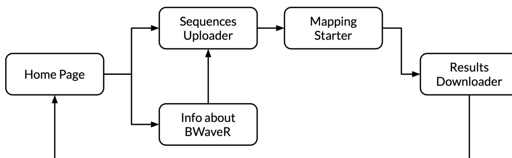
Figure 5.9: Overview of the BWaveR web application
