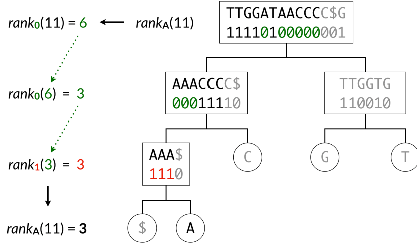
Figure 3.4: A rank query on the wavelet tree
