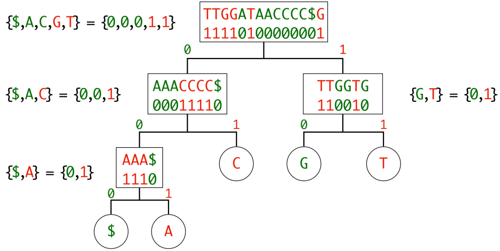
Figure 3.3: Wavelet tree of the sequence TTGGATAACCCC\$G
