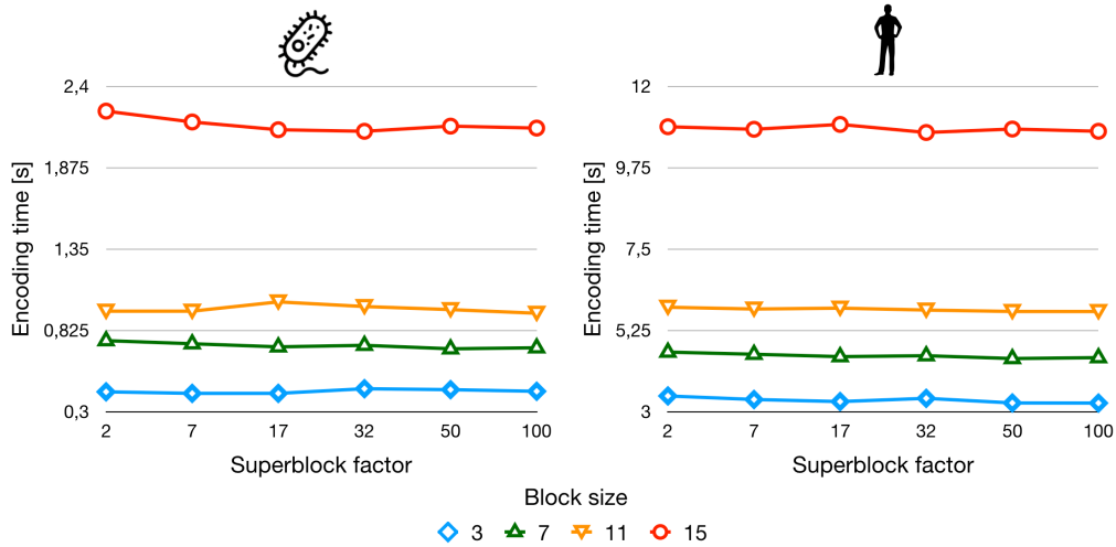
Figure 6.3: Succinct encoding time for E.Coli (left) and Human Chr.21 (right)
