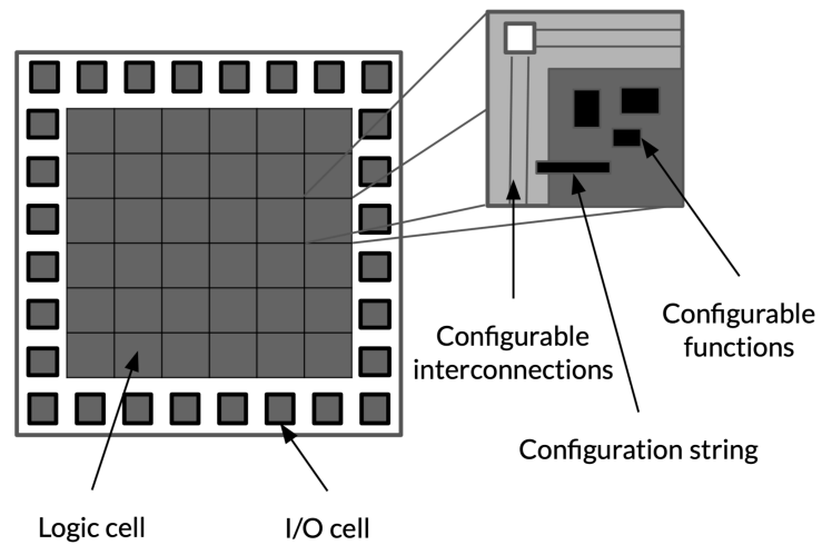
Figure 3.5: FPGA overview
