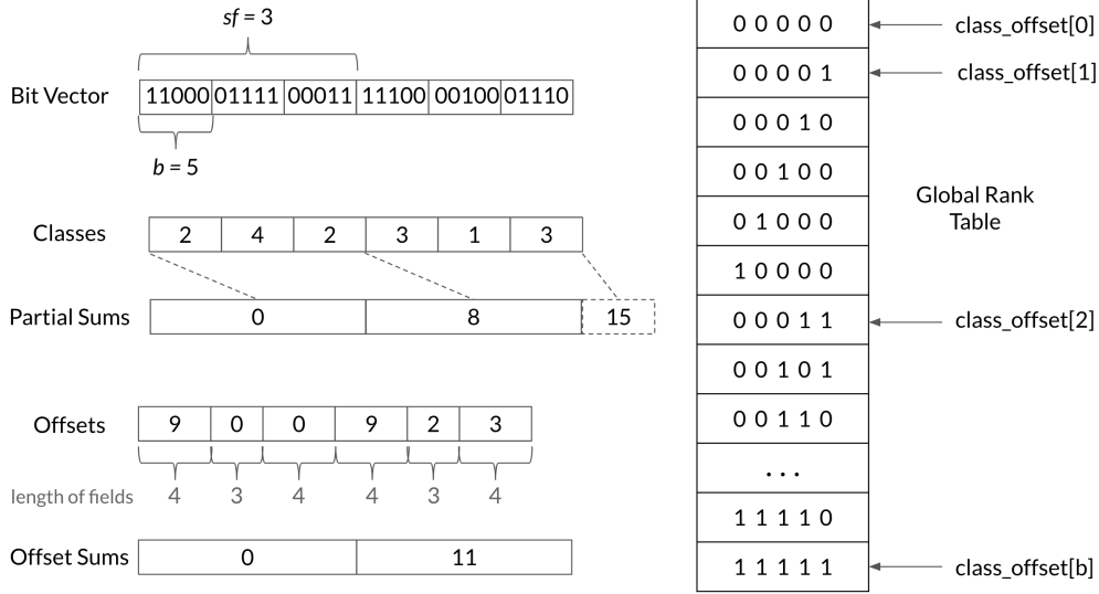
Figure 5.6: Overview of the implemented RRR sequence
