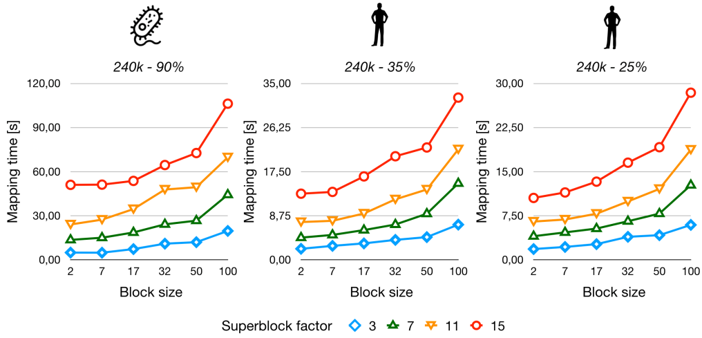
Figure 6.5: Reads mapping time comparison
