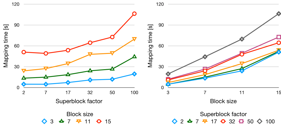
Figure 6.4: Reads mapping time for E.Coli
