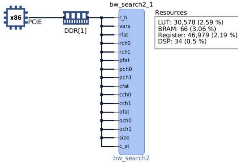
Figure 5.7: Schematic of the hardware design
