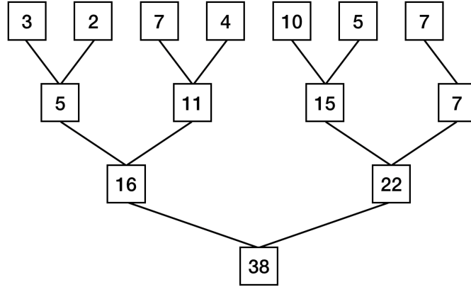
Figure 5.8: Example of reduction: sum of array elements
