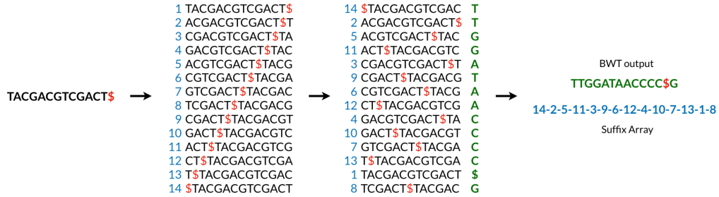
Figure 3.1: Burrows-Wheeler Transform and Suffix Array construction
