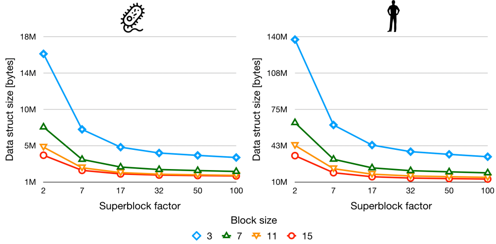
Figure 6.2: Data structure's size for E.Coli (left) and Human Chr.21 (right)
