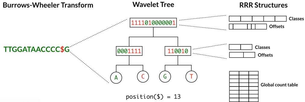
Figure 5.5: Overview of the BWaveR data structure
