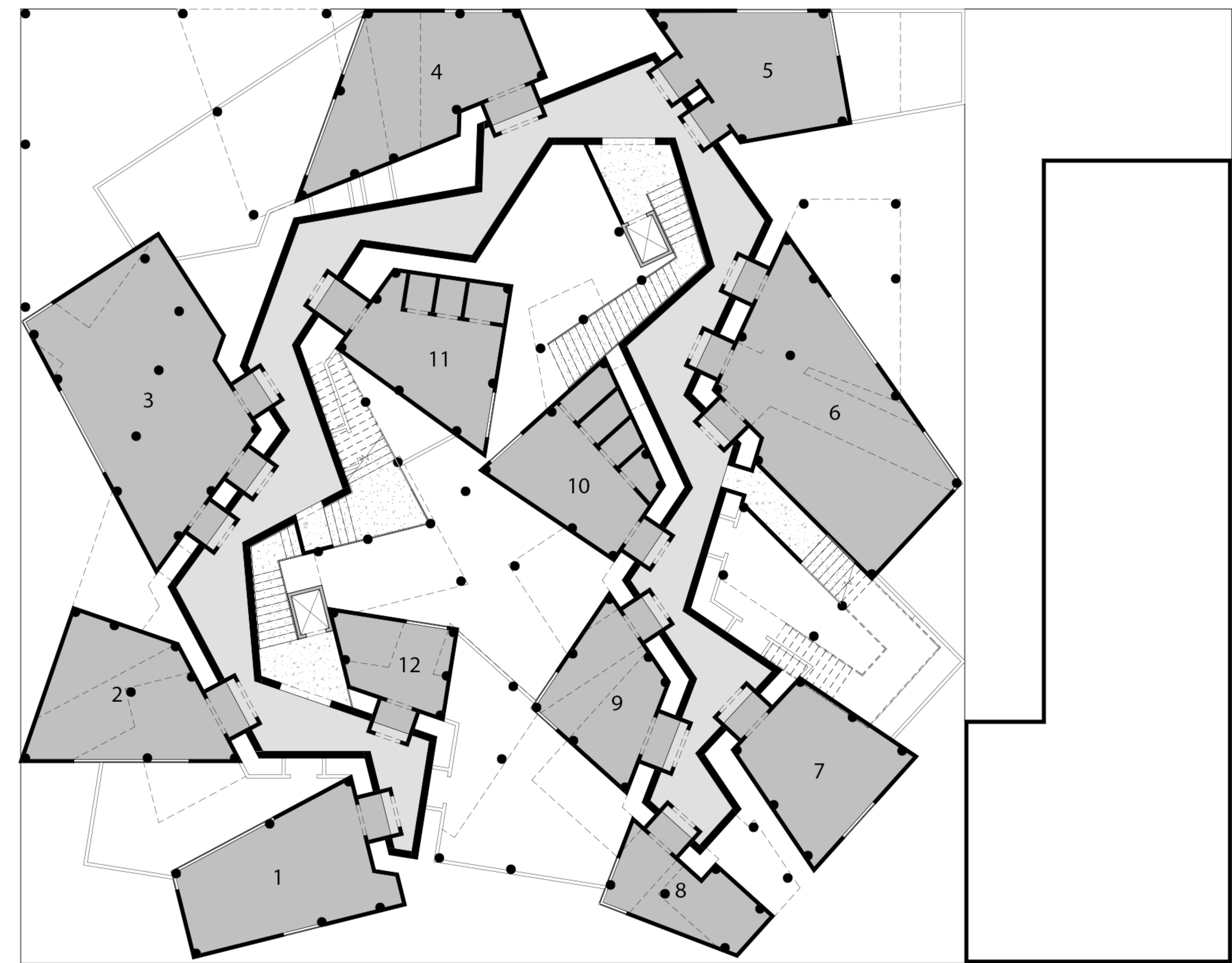
First Floor Plan 1:100
