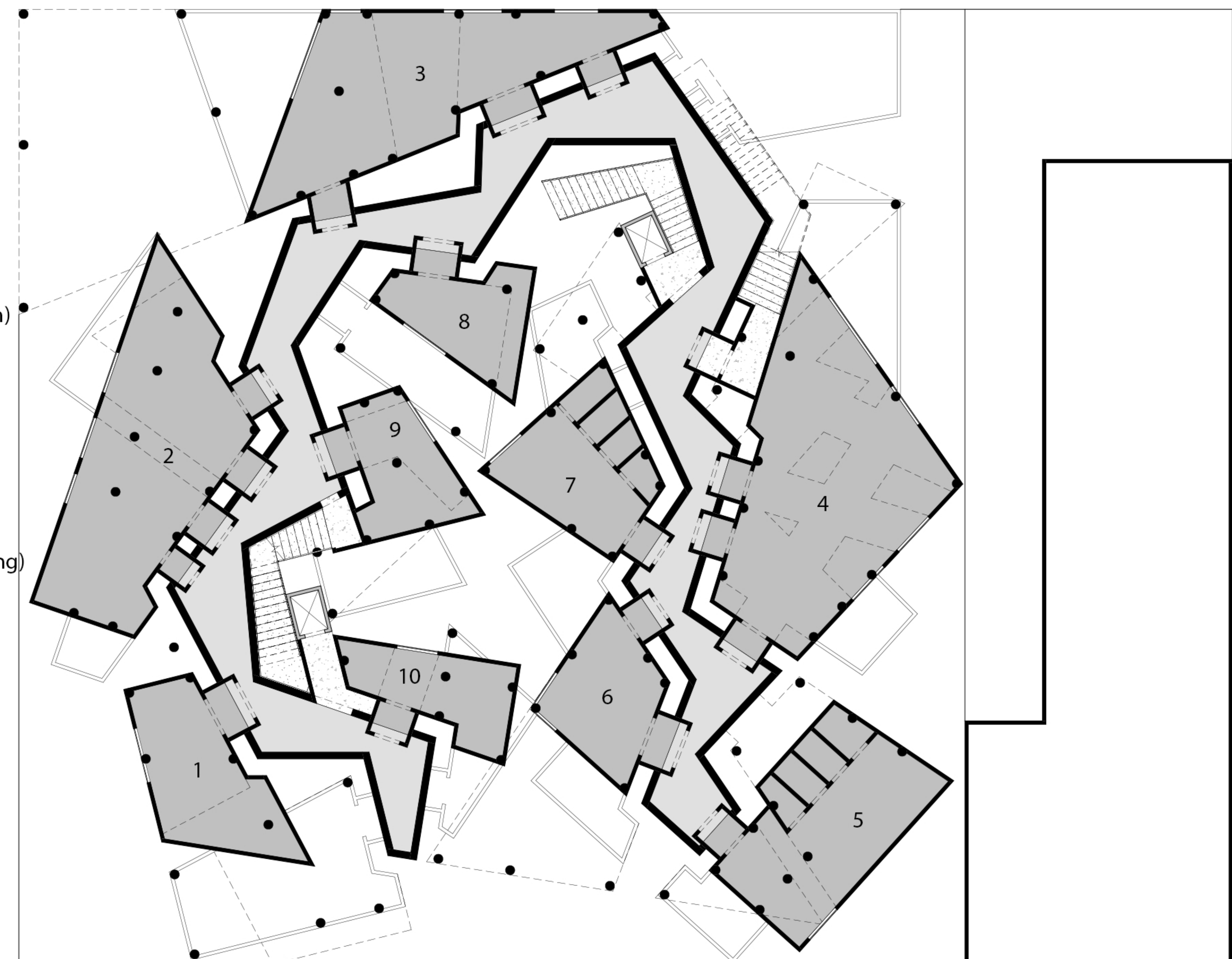
Third Floor Plan 1:100
