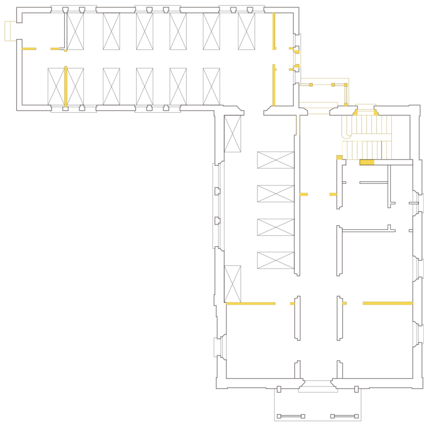
ORIGINAL GROUND FLOOR PLAN 1:200
