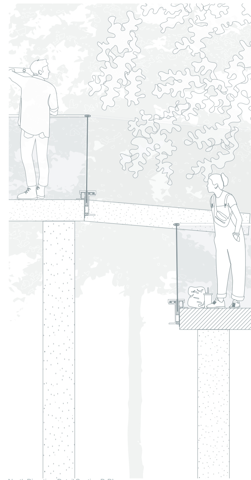
North Direction: Detail Section D-D'
