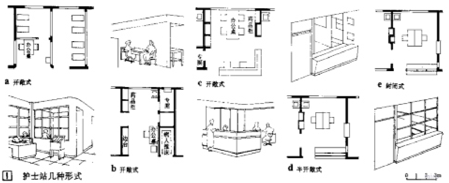
Nurse station
