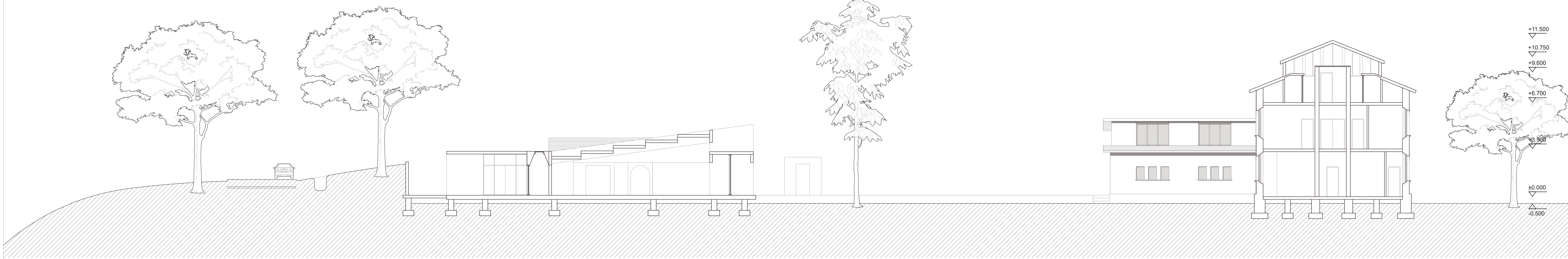
SECTION B-B 1:100
