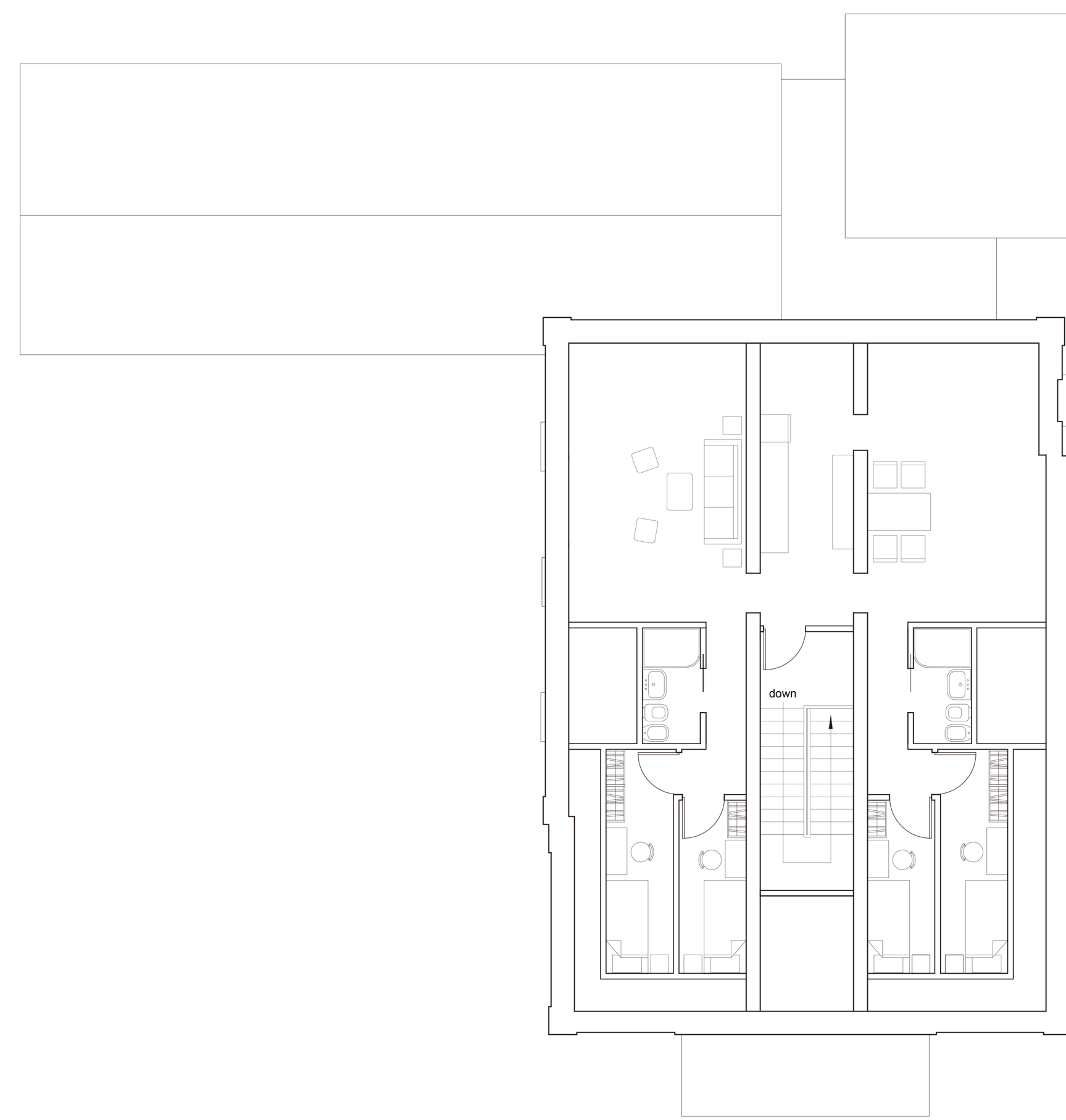
SECOND FLOOR PLAN 1:100
