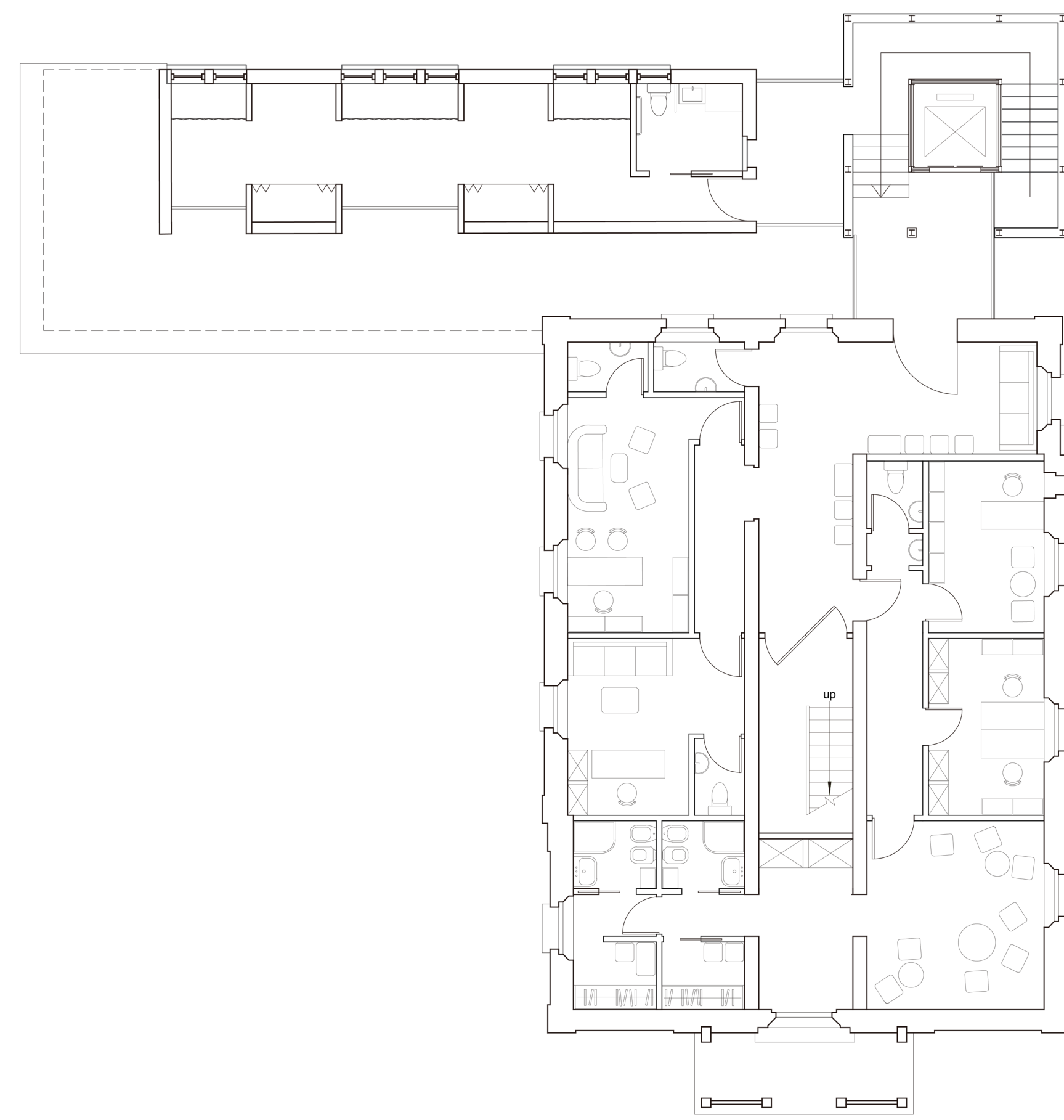
FIRST FLOOR PLAN 1:100
