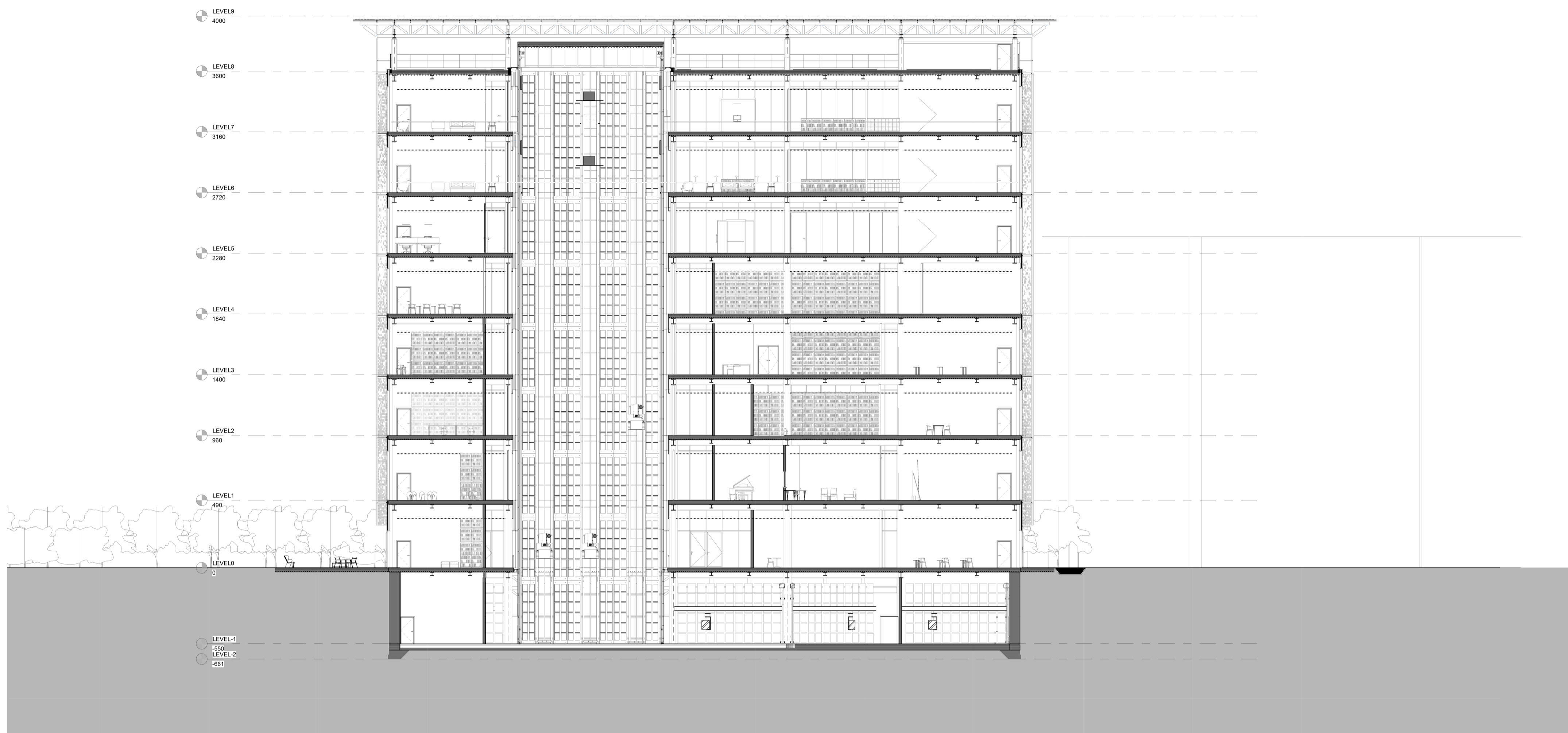
TRANSVERSE SECTION - through the Tower of Books
