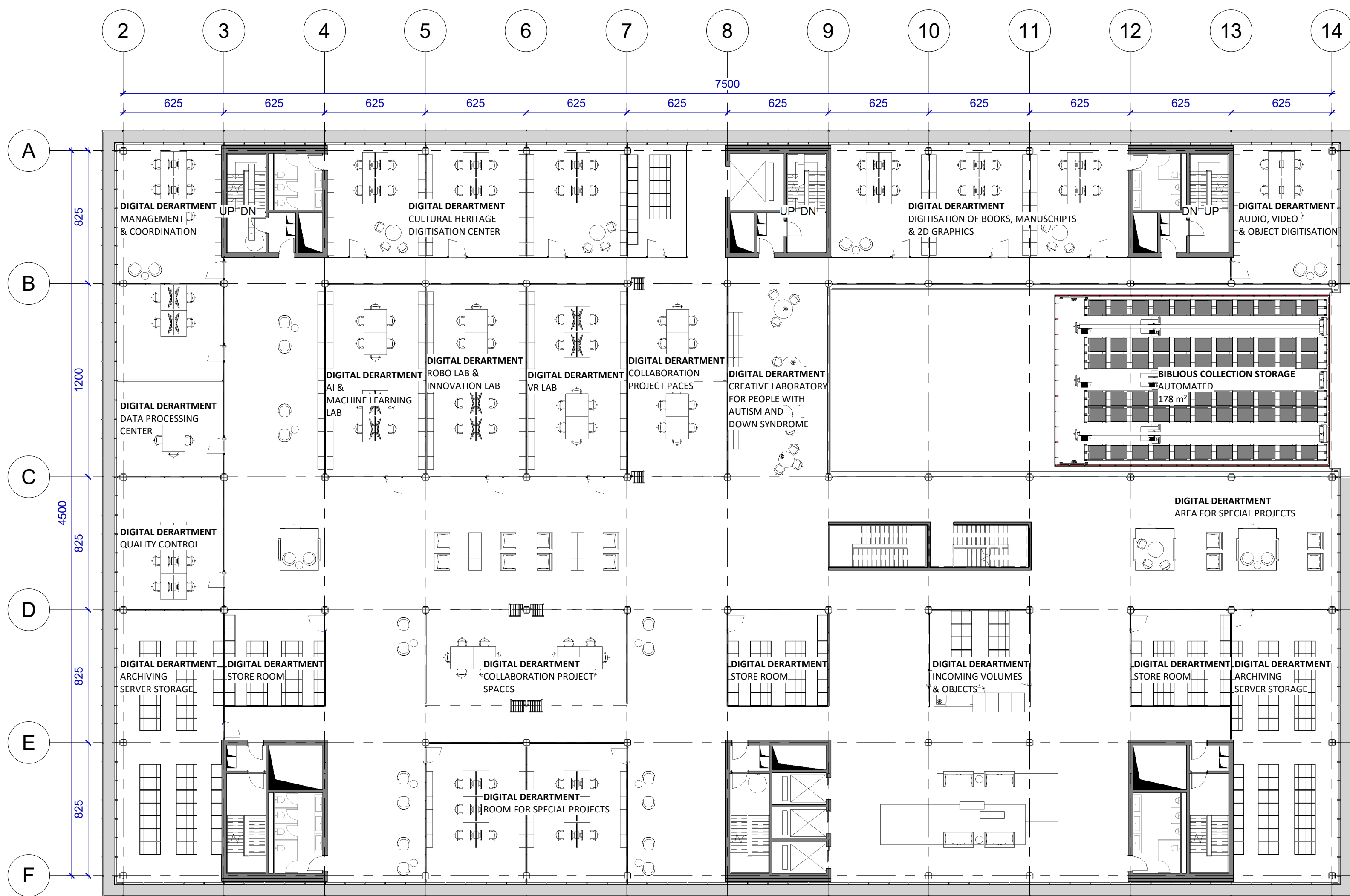
LEVEL 5 FLOOR PLAN
