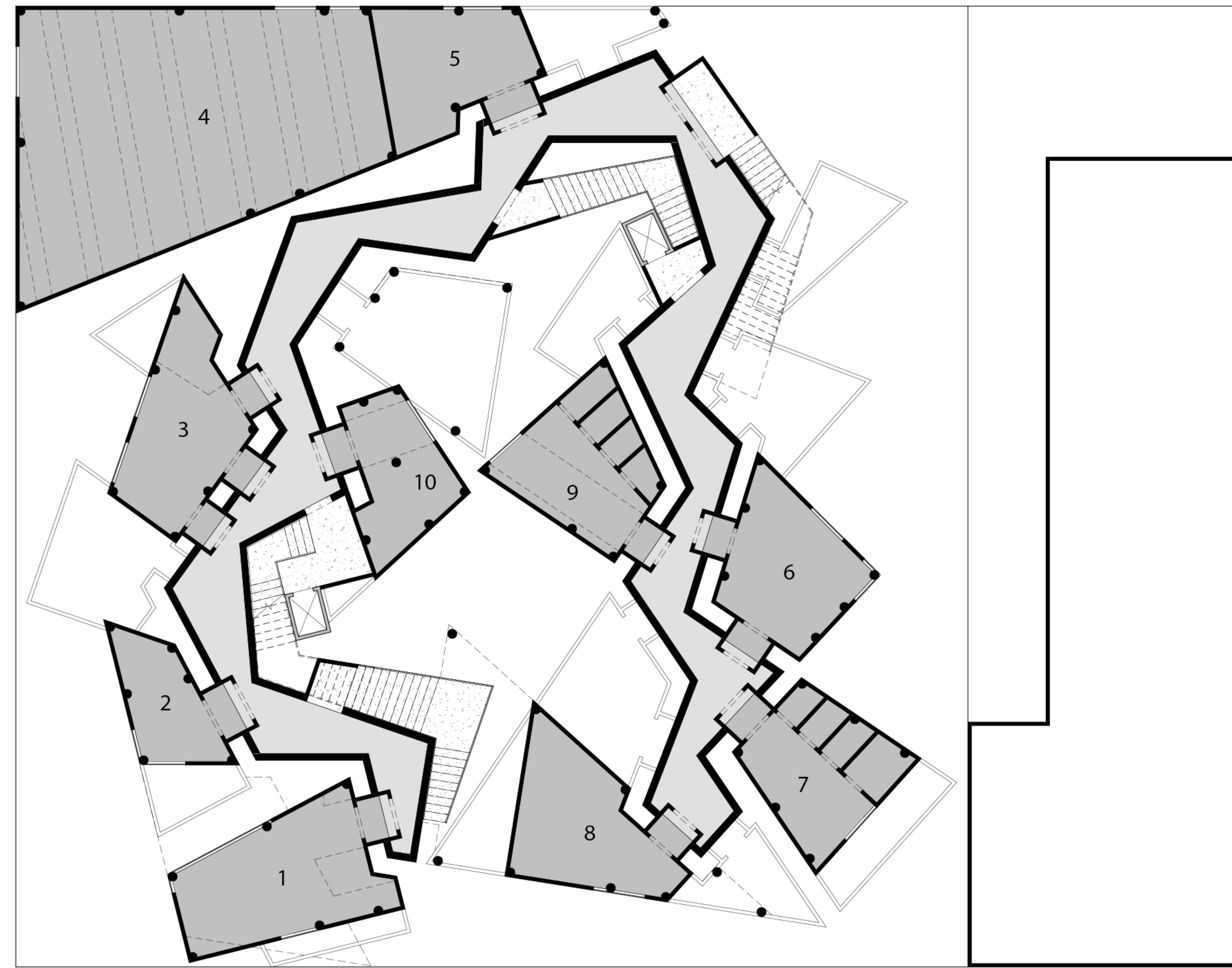
Fifth Floor Plan 1:100
