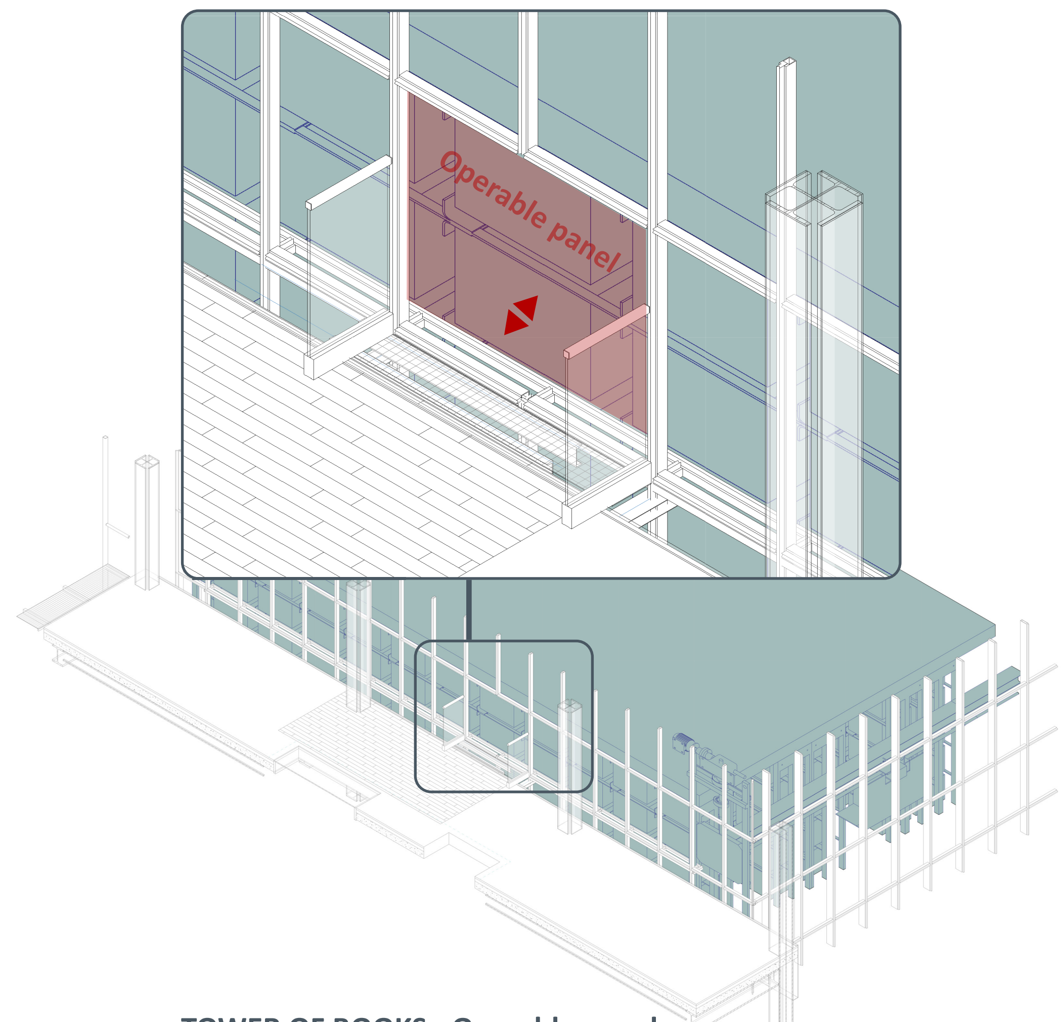
TOWER OF BOOKS - Operable panels for book retrieval by librarian (Level 7)
