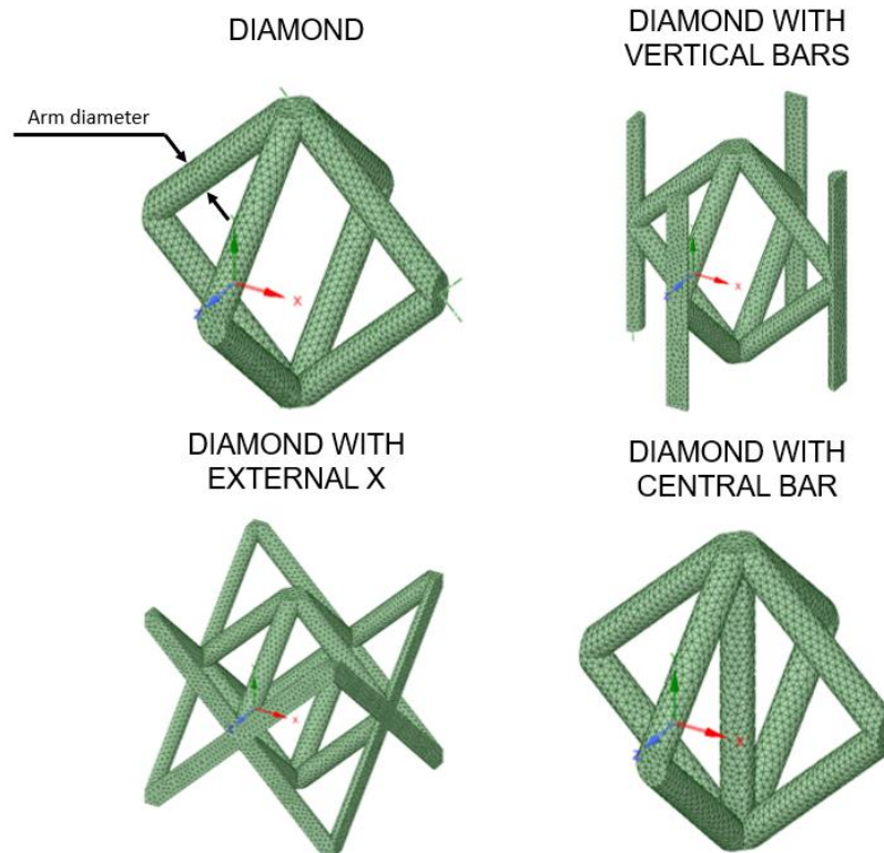
Figure 42. Different types of lattice elements used in this project work. These were the only selected because they attend the 45° overhang constraint. Names were given by the author.
