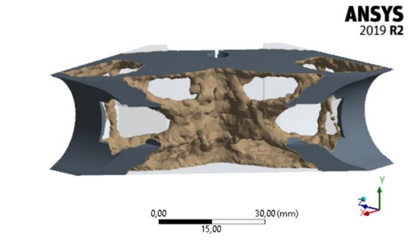
Figure 79. TO results for 15% of the original mass and maximum possible first natural frequency.
