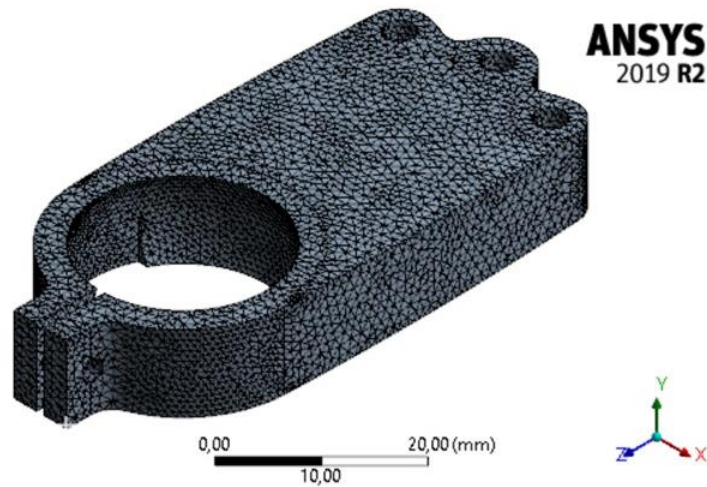
Figure 33. Surface mesh of the single pendulum model, with tetragonal elements.
