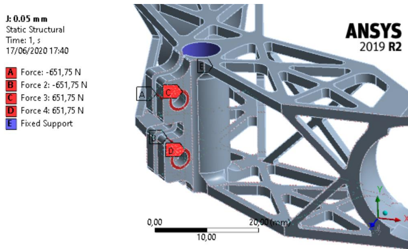
Figure 90. ANSYS model to find the stress at the part when the bolts are tightened.
