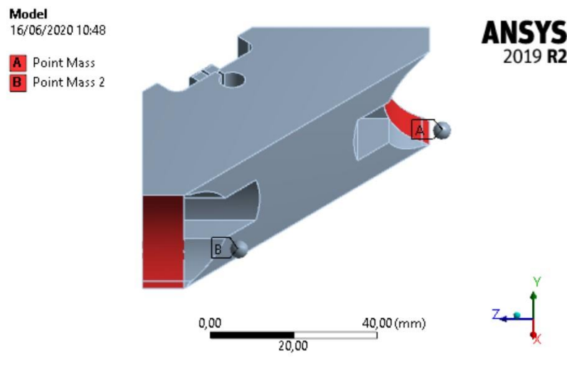
Figure 74. Two "point mass" are present (spheres A and B) and are connected to the surfaces where the pendulum tips has contact with the optimizable region (red surfaces).
