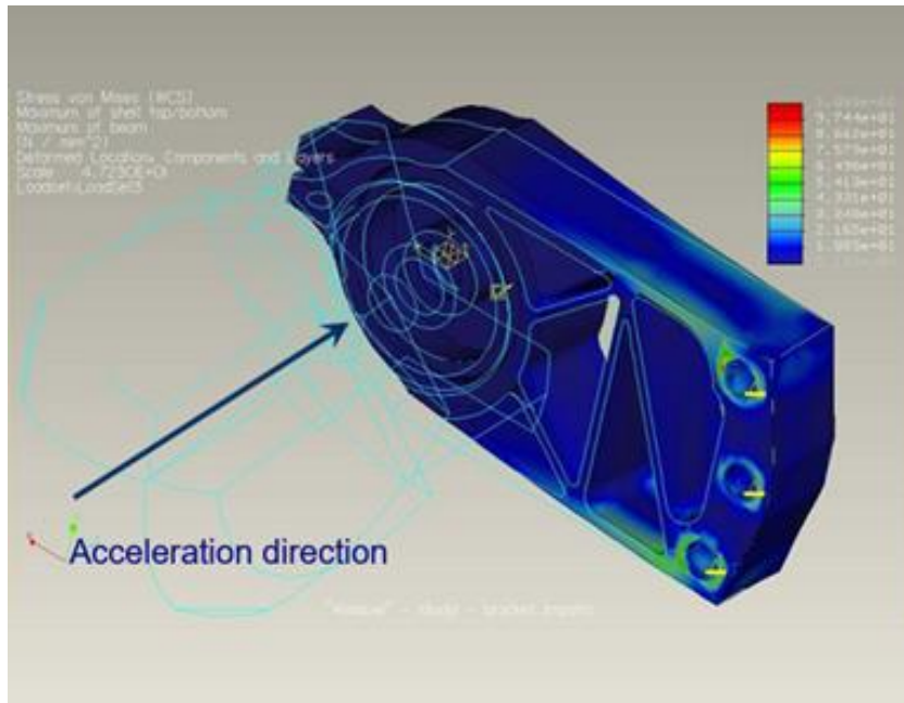
Figure 7. Pendulum arm analysis, acceleration in the Y axis, maximum stress of 108 MPa.
