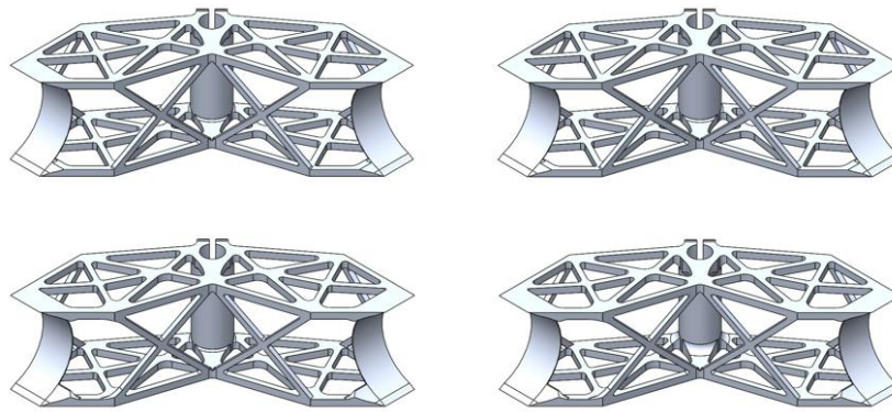
Figure 83. Iterative optimization of the initial shape. 9) Top-left; 10) Top-right; 11) Bottom-left; 12) Bottom-right.
