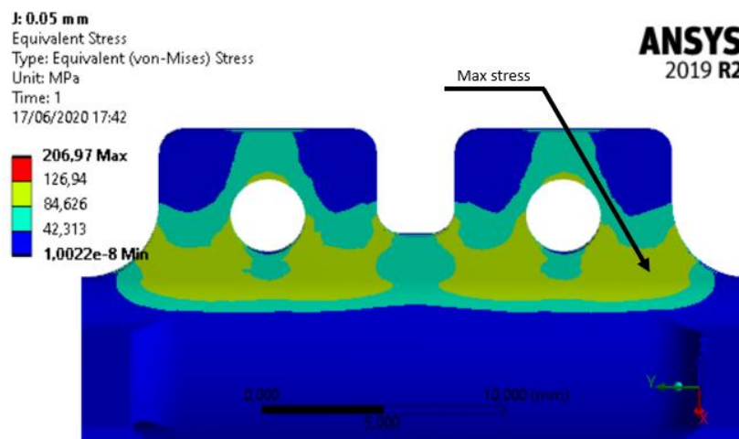
Figure 92. Stress plot at the bolt fixations when the bolt forces are applied.
