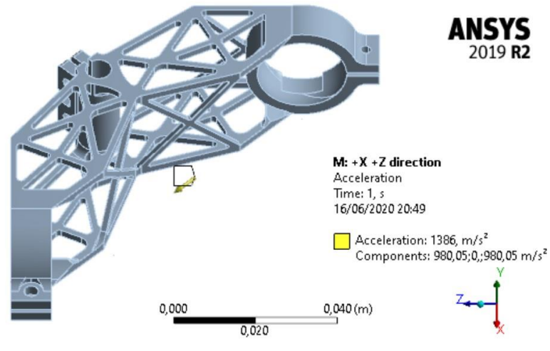
Figure 86. Acceleration direction (+X +Z) that yields the highest stress on the part.
