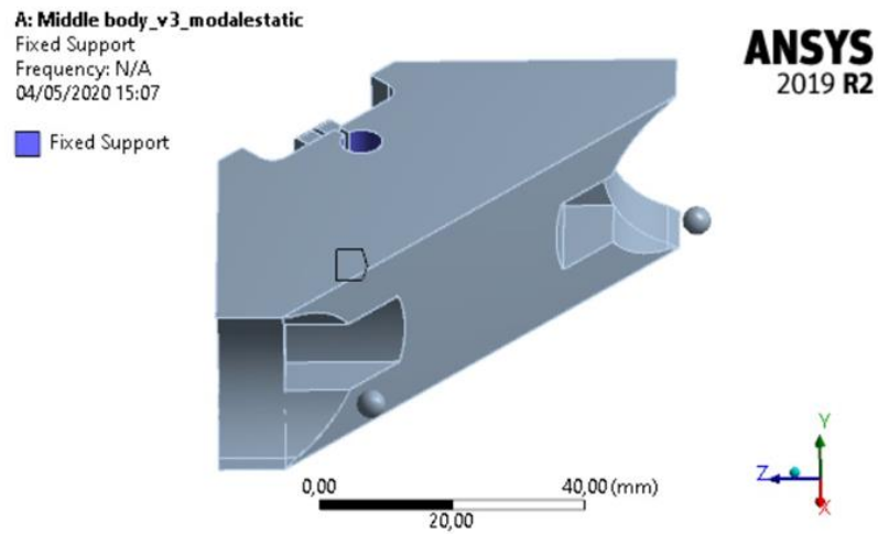
Figure 73. Fixed support boundary condition (region in blue).
