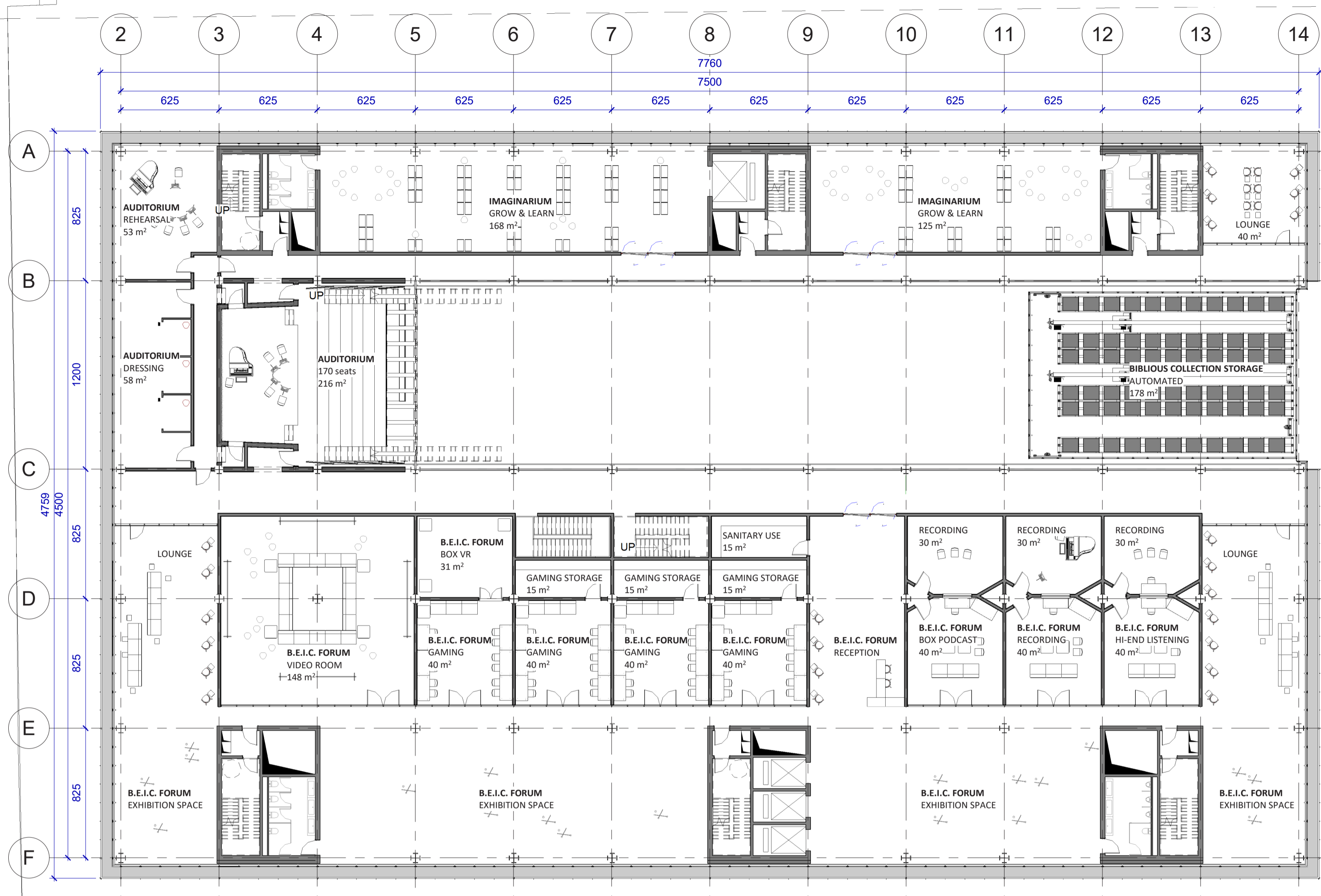
LEVEL 1 FLOOR PLAN
