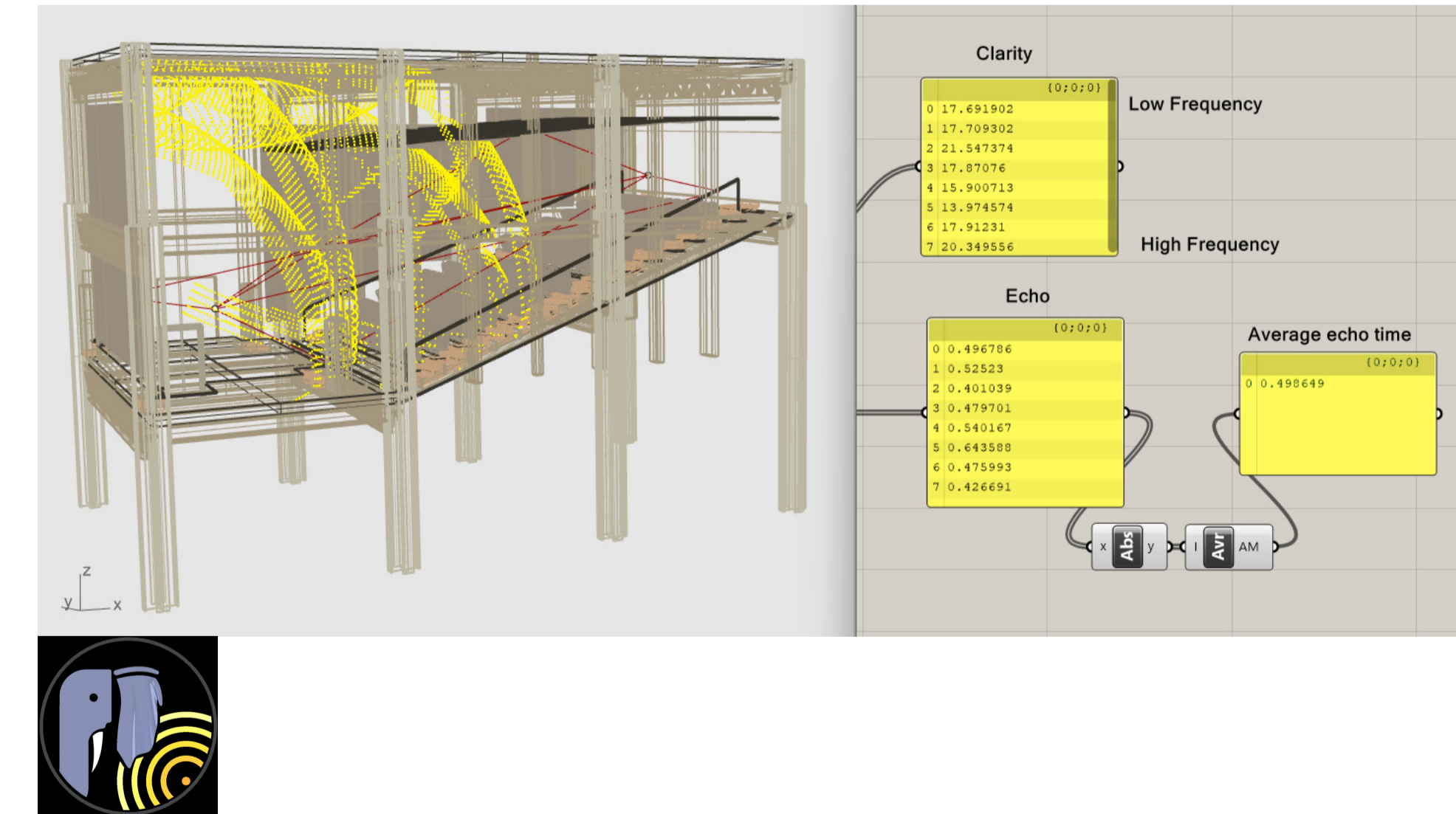
PACHYDERM ACOUSTICAL SIMULATION
