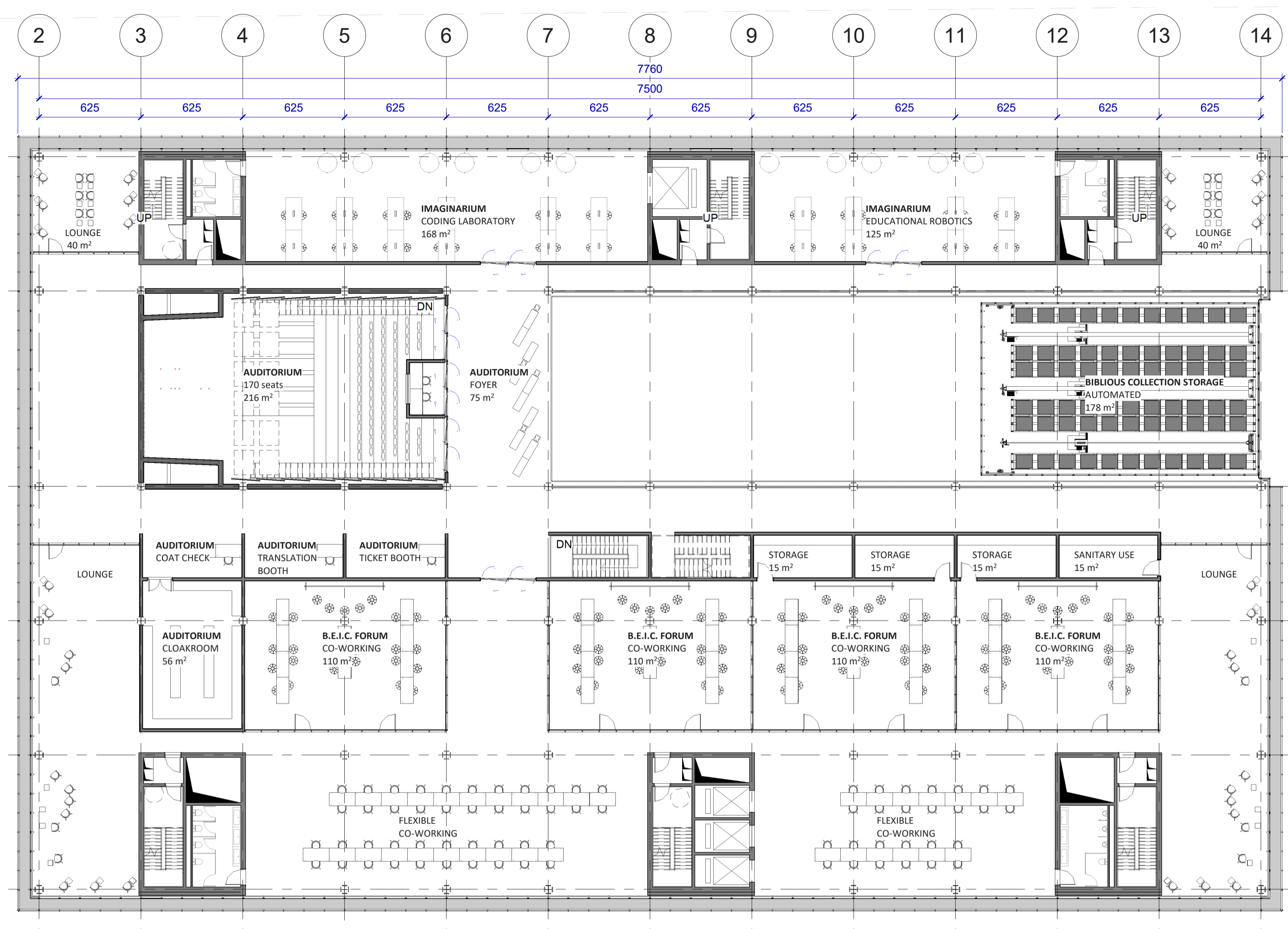
LEVEL 2 FLOOR PLAN
