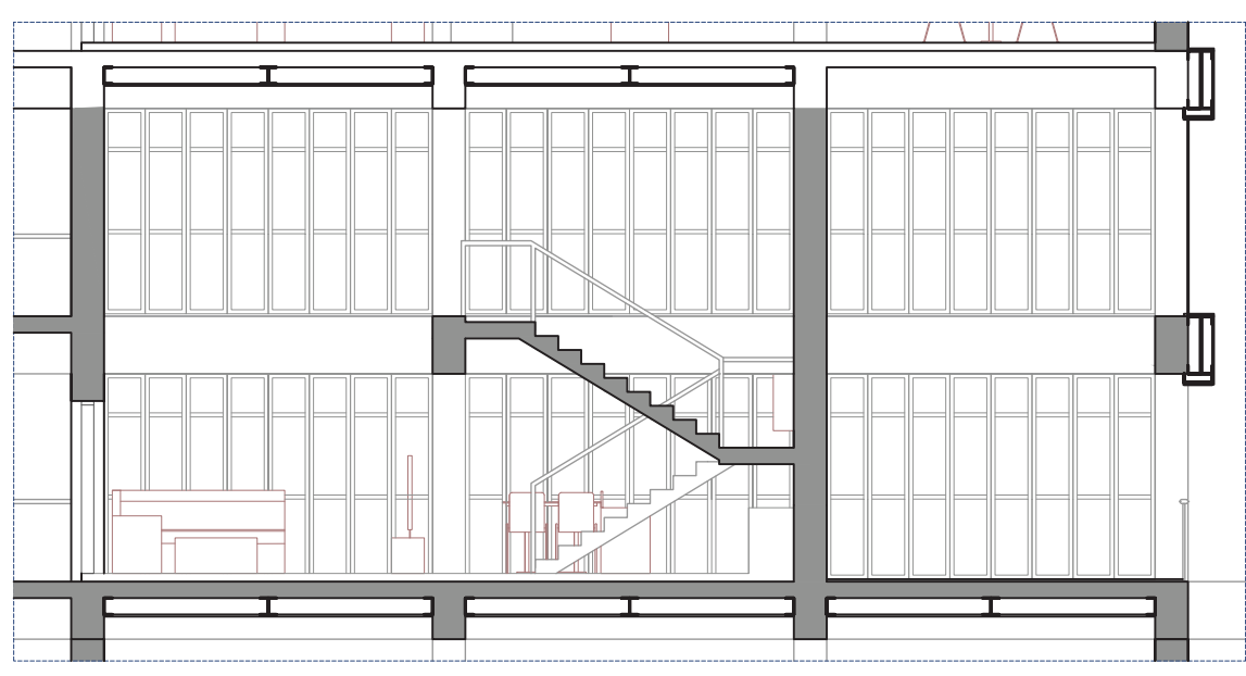
Duplex unit type 1, M=1:100
