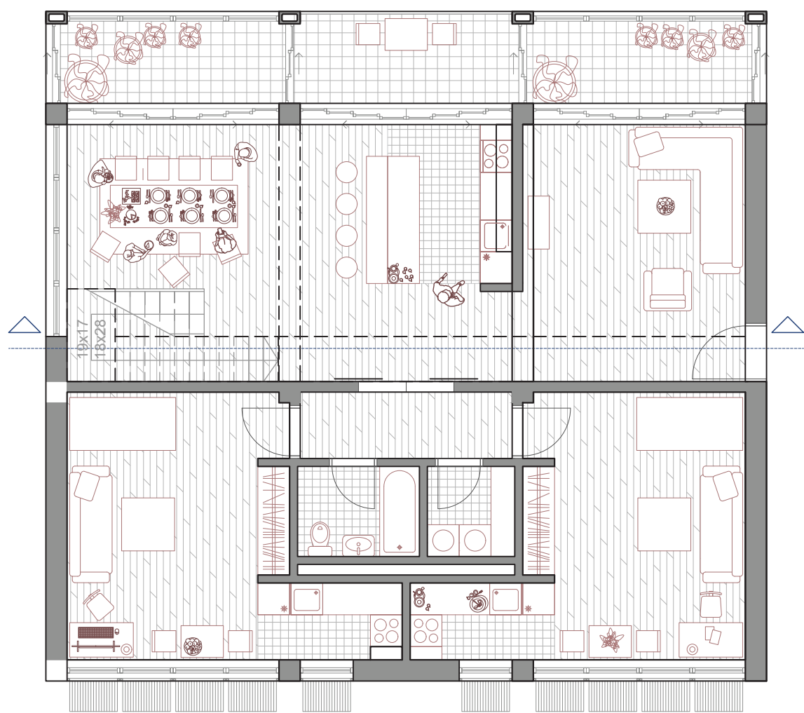
Duplex unit type 1, M=1:100
