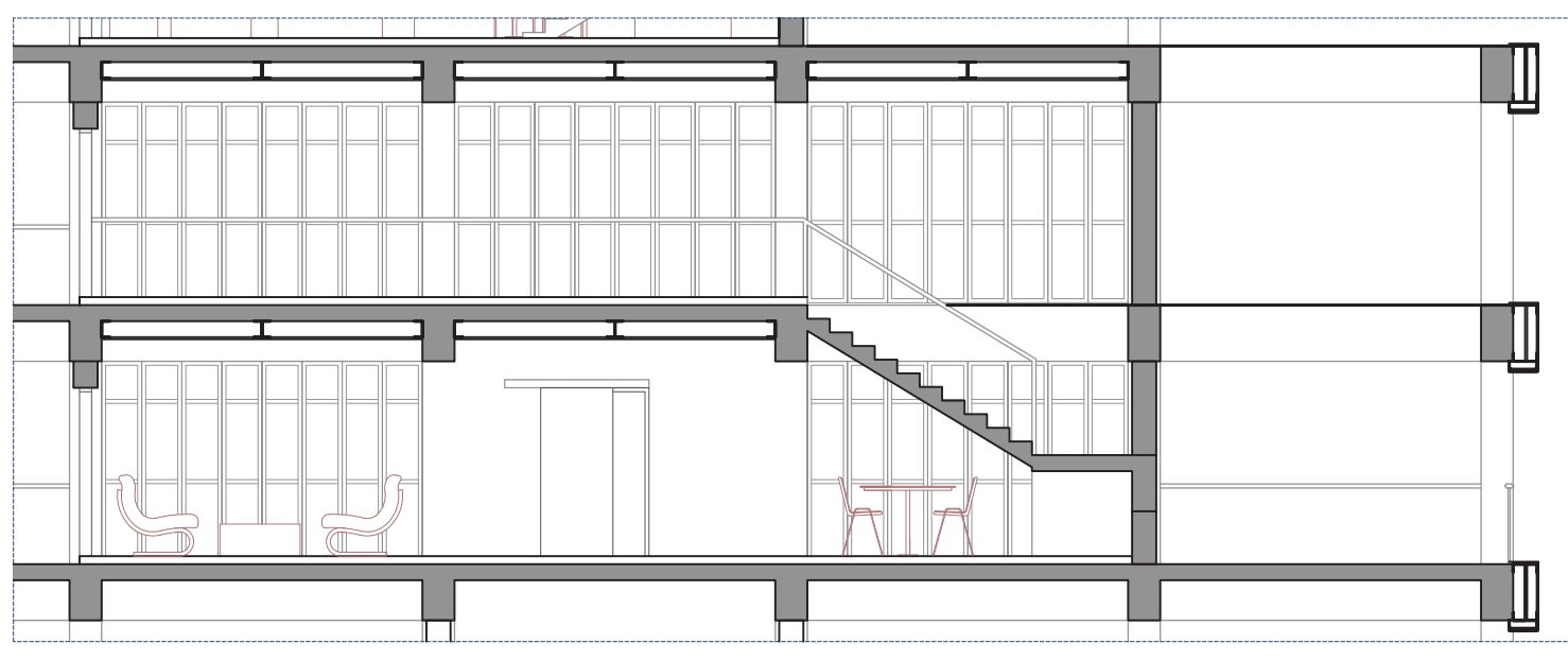
Duplex unit type 2, M=1:100
