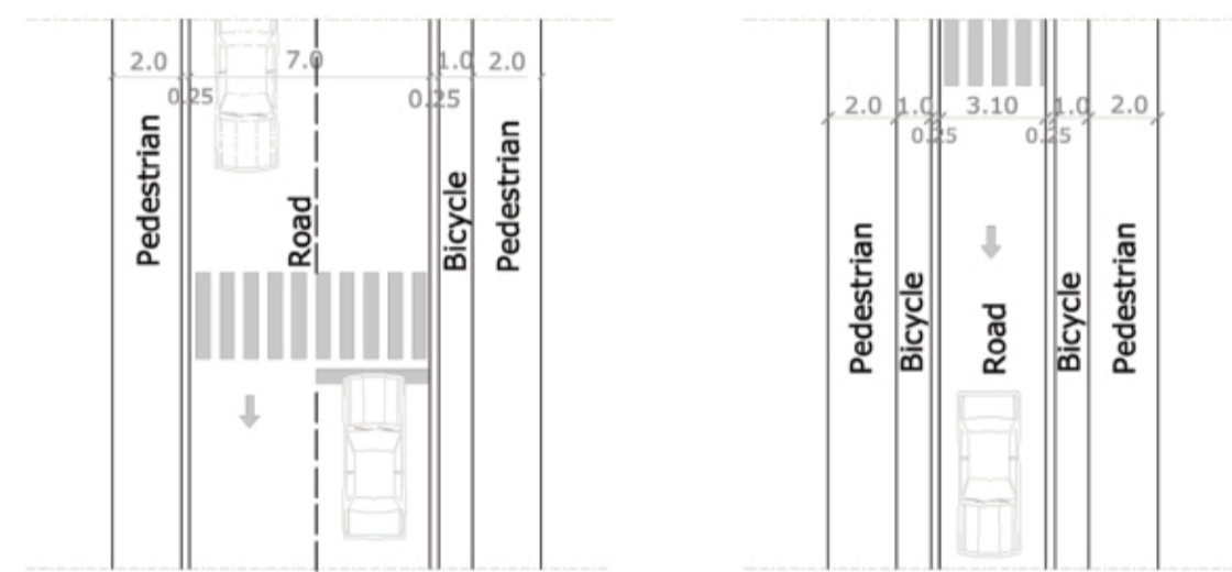
TYPE 3-secondary street, 2 lanes TYPE 4-one-way street
