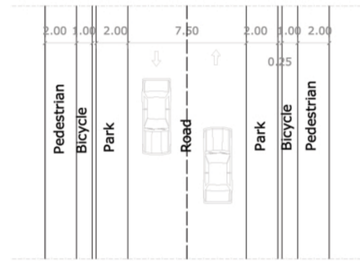
TYPE 2-street with public transportation, 2 directions
