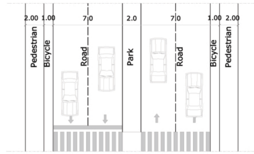
TYPE 1-4 lane street, 2 directions
