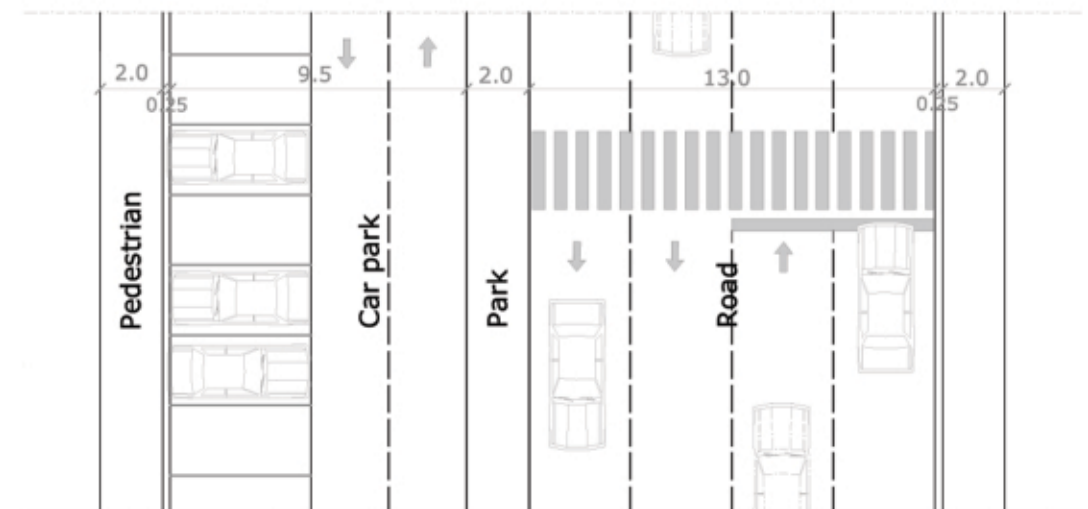
TYPE 6-street with public transportation, 2 directions, 4 lanes
