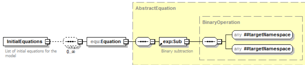
Figure 4.22: Initial Equations
