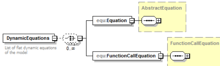
Figure 4.24: DynamicEquations element
