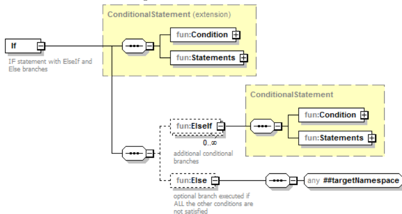
Figure 4.16: If statement
