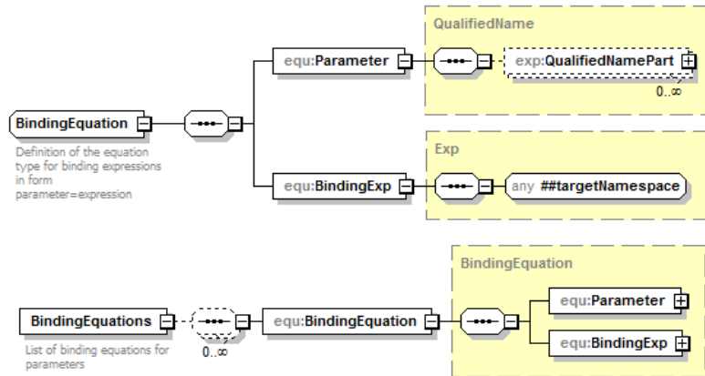
Figure 4.20: Binding Equations
