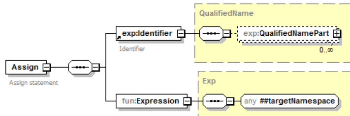
Figure 4.15: Assign element
