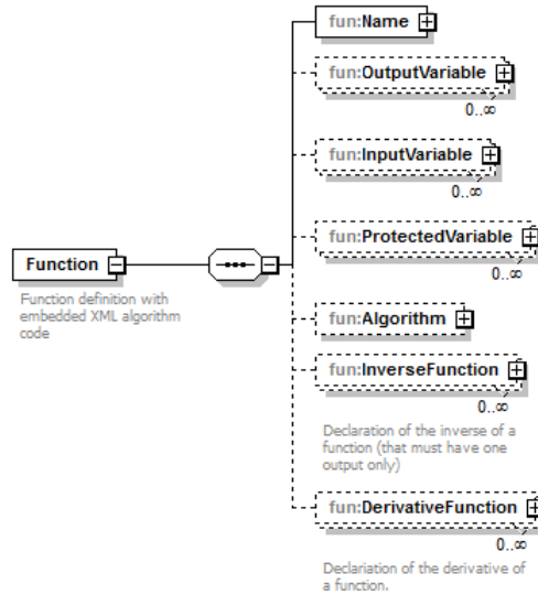
Figure 4.13: Function definition
