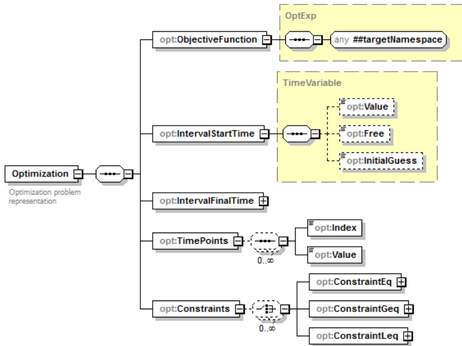
Figure 4.26: Optimization problem extension
