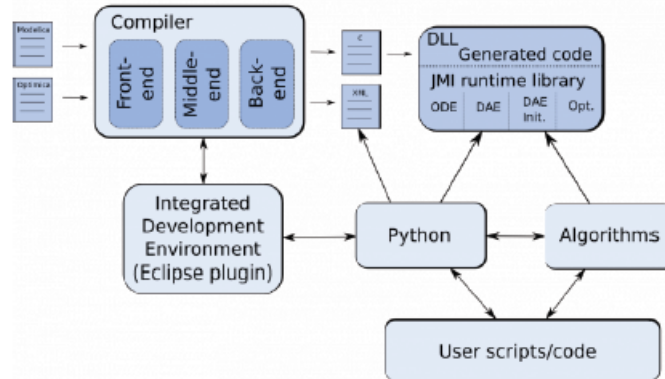
Figure 6.1: JModelica.org architecture
