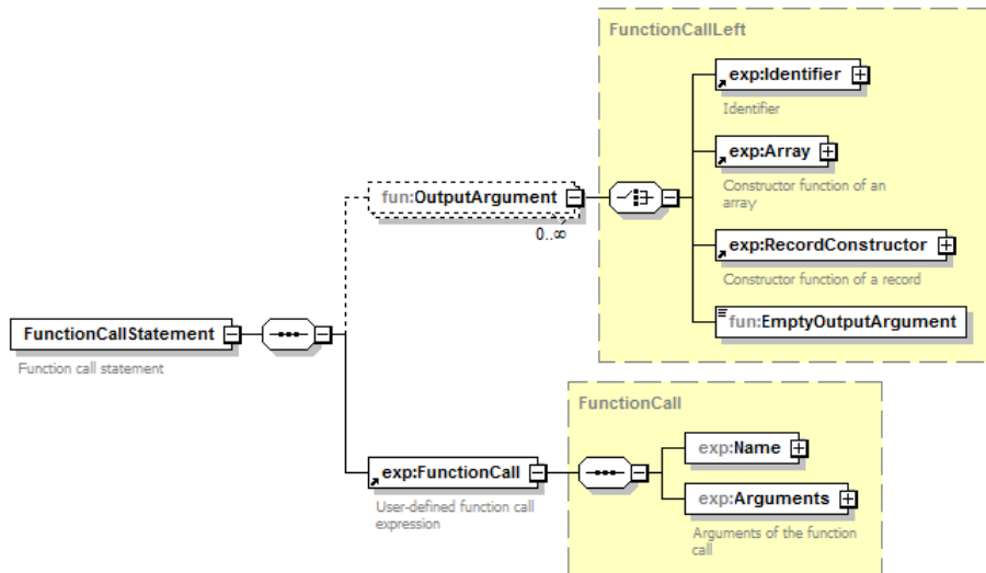
Figure 4.18: FunctionCallStatement definition
