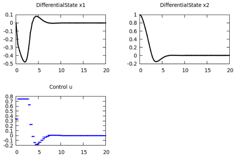
Figure 6.2: Results returned by ACADO
