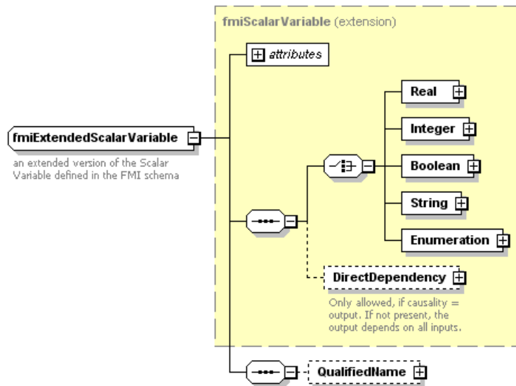
Figure 4.6: fmiExtendedScalarVariable
