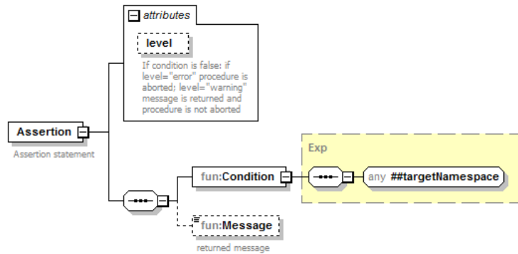
Figure 4.19: Assertion element
