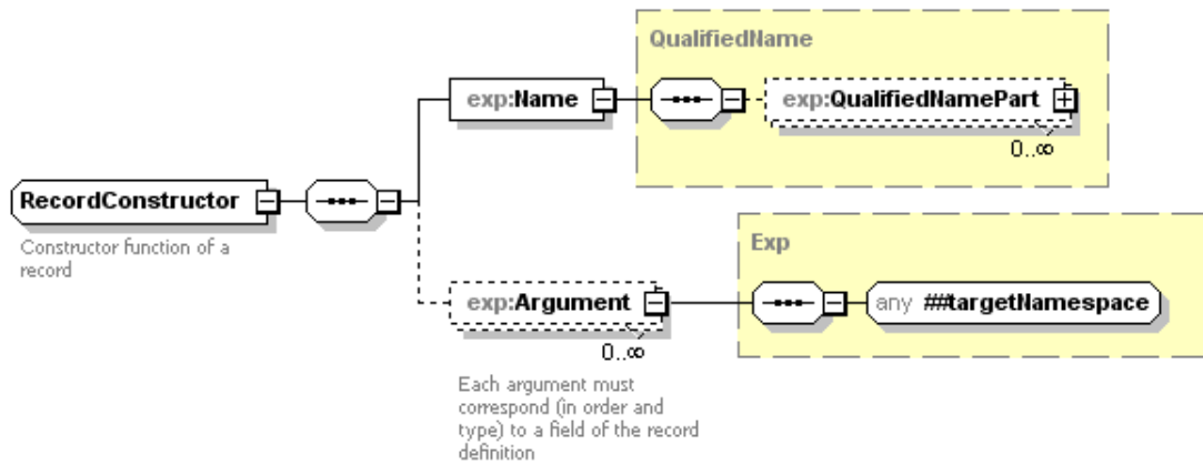
Figure 4.10: RecordConstructor definition
