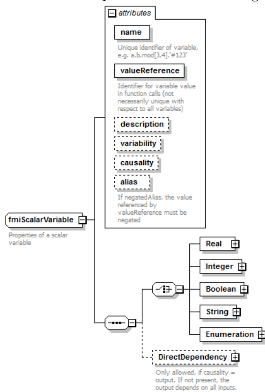
Figure 4.3: Scalar Variables representation in the original FMI schema
