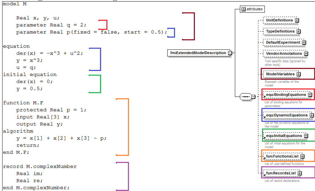
Figure 5.1: Matching a Modelica model with the XML schema
