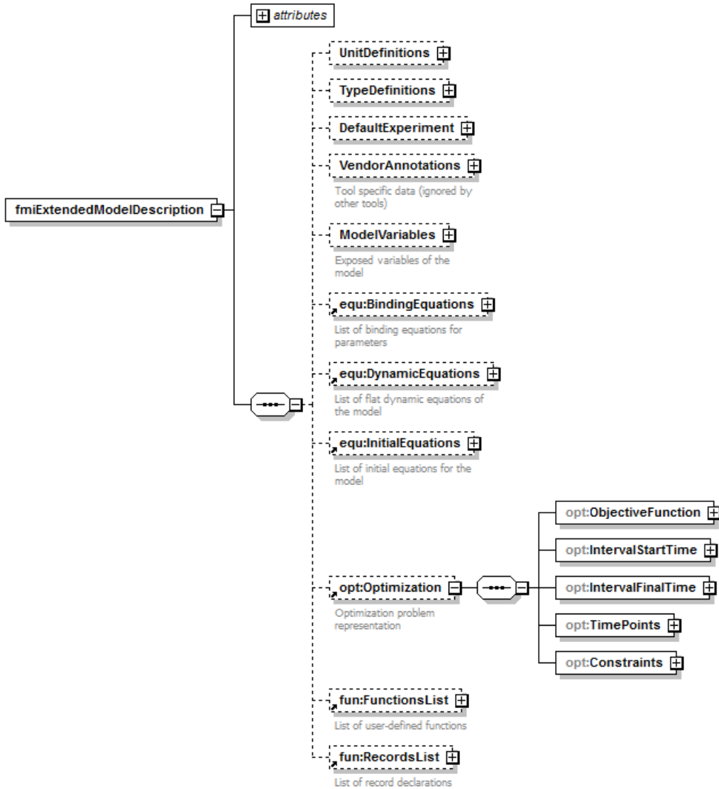
Figure 4.27: Overall of the schema extended by the optimization module
