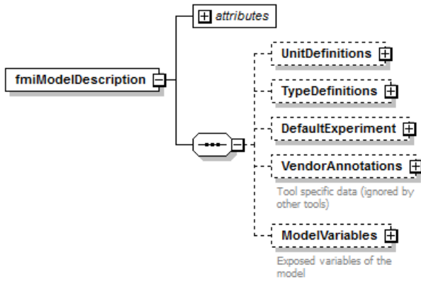
Figure 4.2: Overall of the original FMI schema
