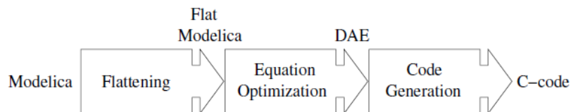
Figure 3.1: Modelica translation process
