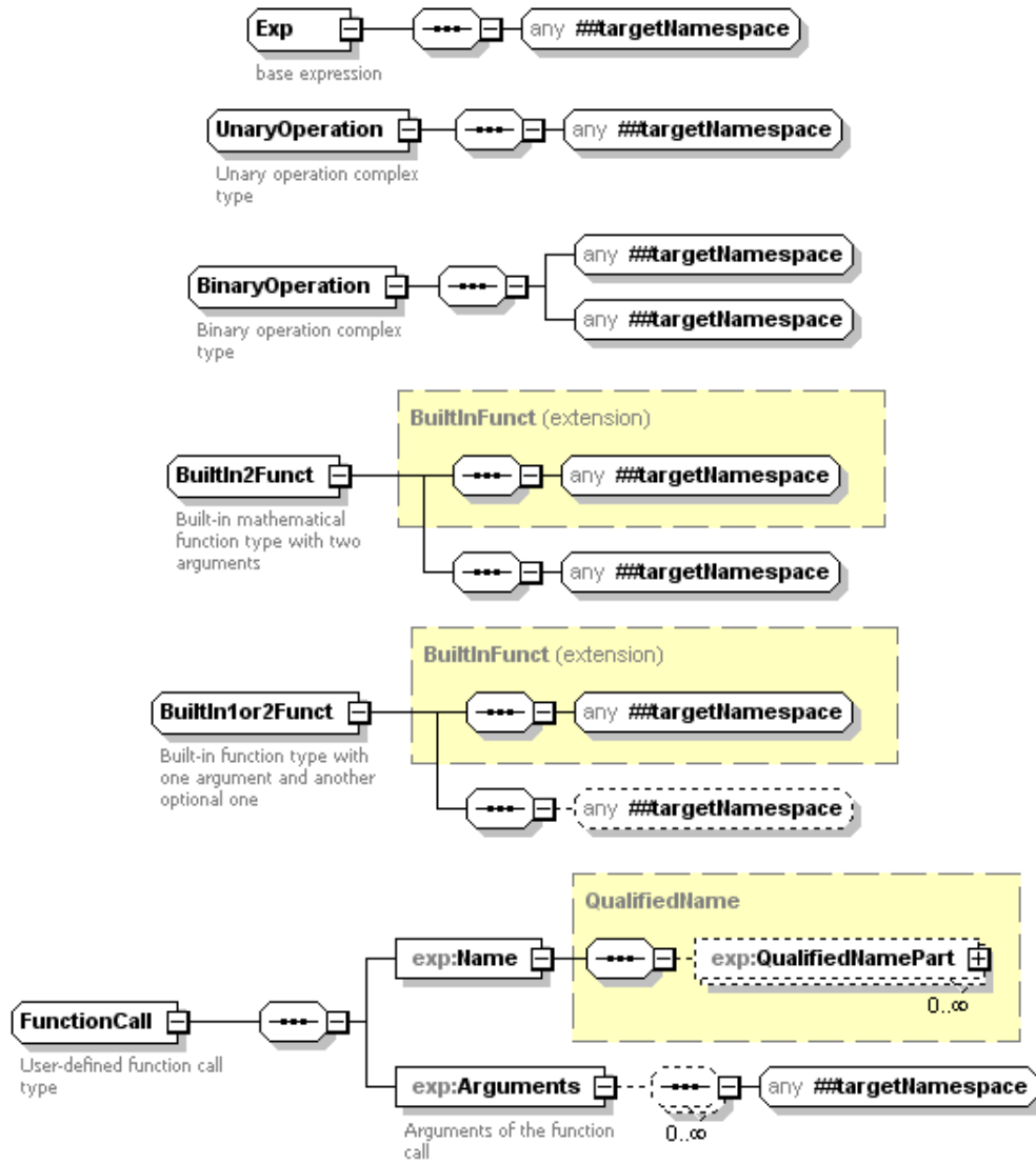
Figure 4.7: Expression complex types
