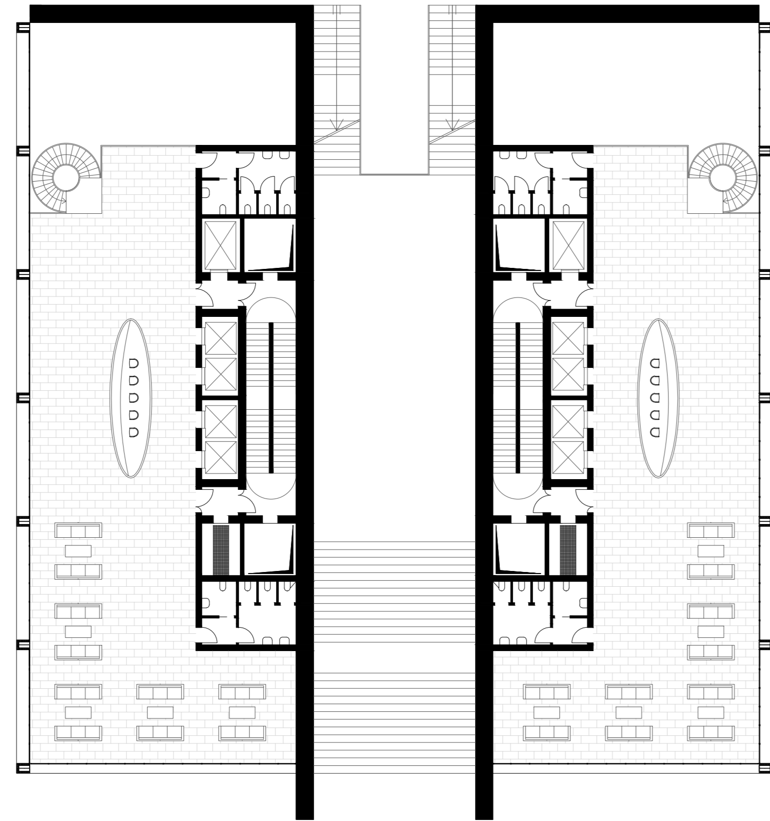
PIANO +7.00
