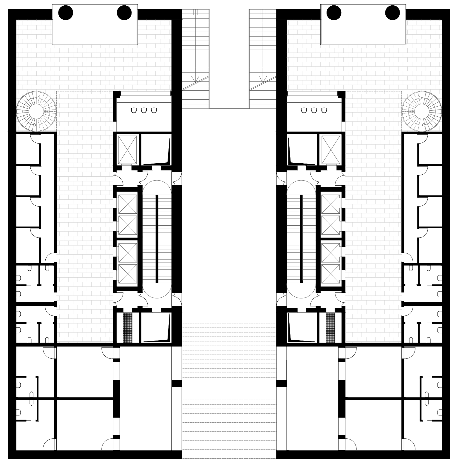
PIANO TERRA
