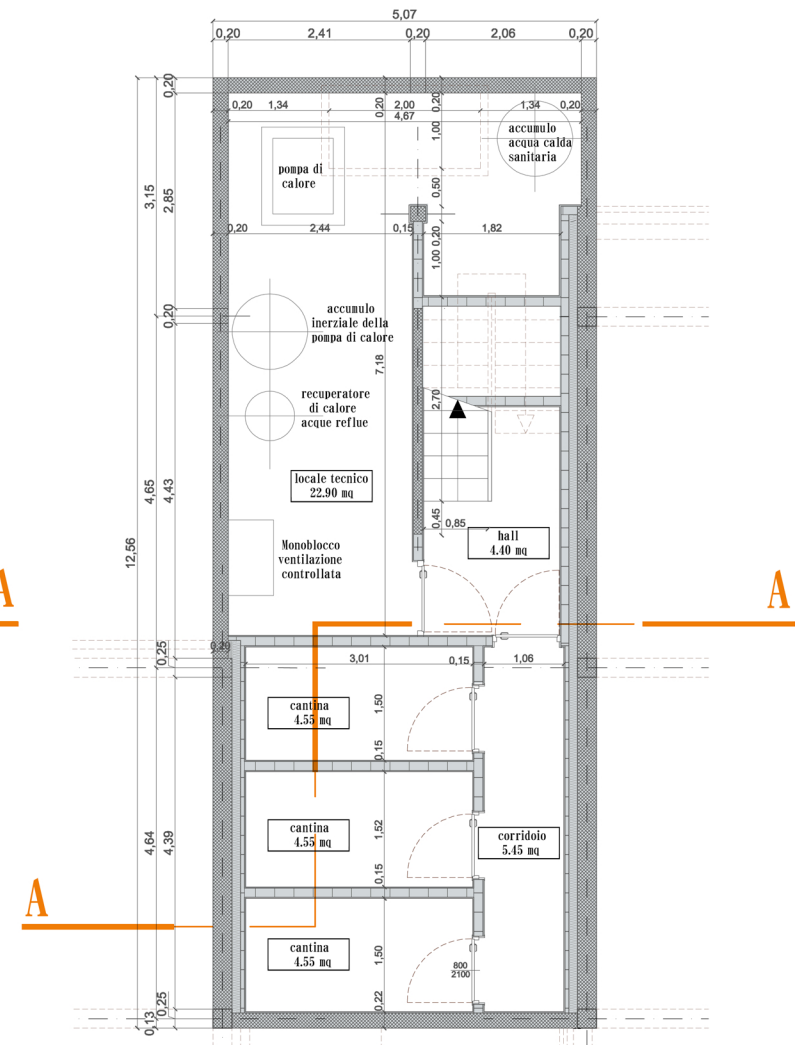
PIANO INTERRATO 1/50
