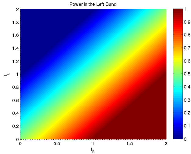
Figure 7.30: Best response for a user increasing the interference in the two bands.
