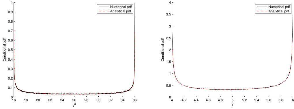
Figure 7.12: Conditional pdf of y^2 (left) and y (right) when x_1 = 5 and d = 1 .
