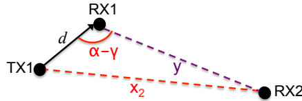
Figure 7.15: Triangle used to characterize x_2 .
