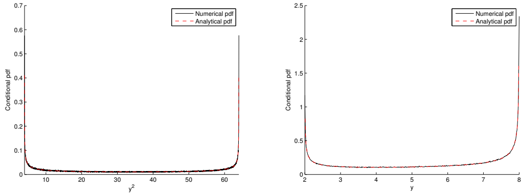
Figure 7.13: Conditional pdf of y^2 (left) and y (right) when x_1 = 5 and d = 3 .
