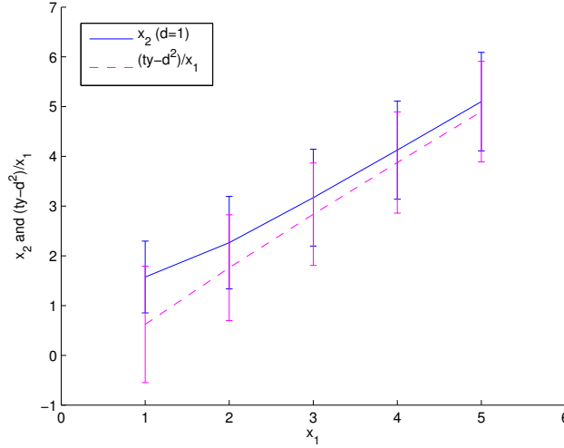
Figure 7.25: Comparison between the average value of x_2 when d = 1 with the average value of the bound (ty - d^2)/x_1 .
