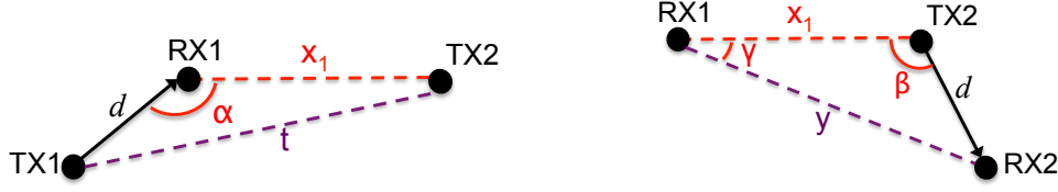
Figure 7.11: Triangles derived from the considered topology.
