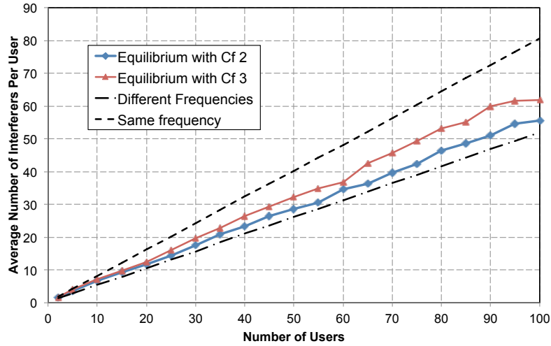
Figure 4.4: Average number of interferers per user.
