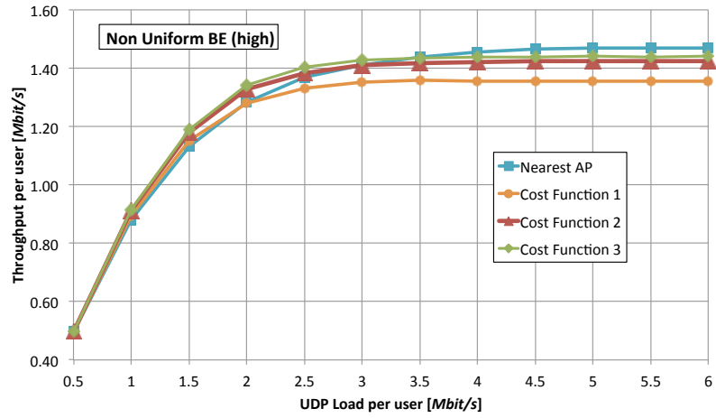
Figure 2.9: Average throughput (BE) per user (located in high density zones) non-uniform topologies.
