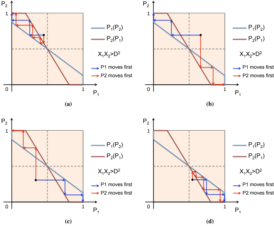
Figure 6.18: Best response dynamics from different starting points.
