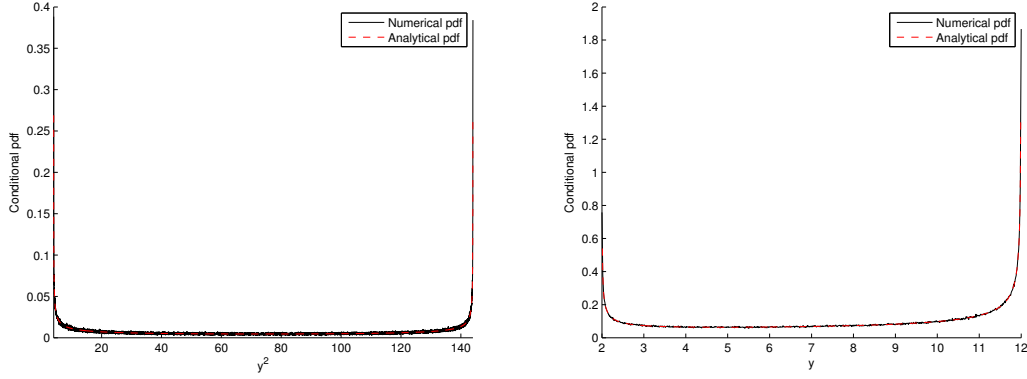
Figure 7.14: Conditional pdf of y^2 (left) and y (right) x_1 = 5 and d = 7 .
