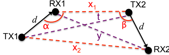
Figure 7.7: Scenario considered for the evaluation of the coupling probability.
