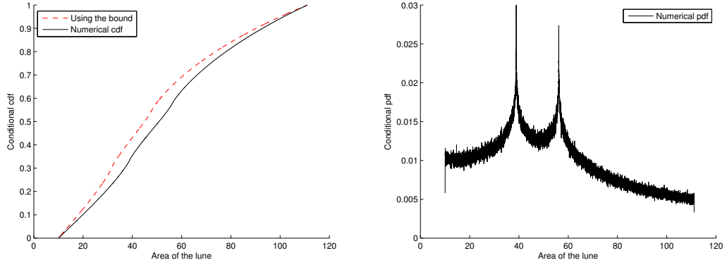
Figure 7.23: Cdf and pdf for the area of the lune when x_1 = 5 and d = 1 .
