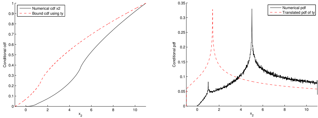
Figure 7.21: Conditional cdf (left) and pdf (right) of x_2 by simulation when x_1 = 5 and d = 3 .
