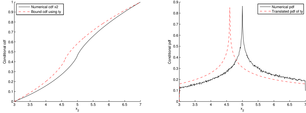
Figure 7.20: Conditional cdf (left) and pdf (right) of x_2 by simulation when x_1 = 5 and d = 1 .
