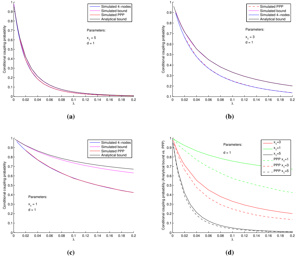
Figure 7.24: Conditional coupling probability when d = 1 varying x_1 .
