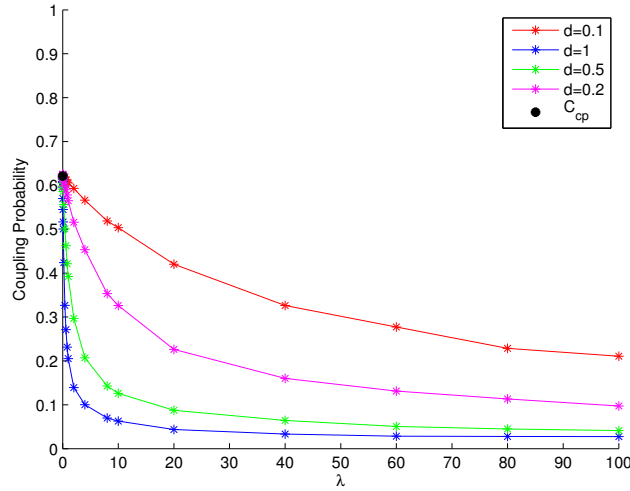
Figure 7.26: Simulated coupling probability for different values of d .
