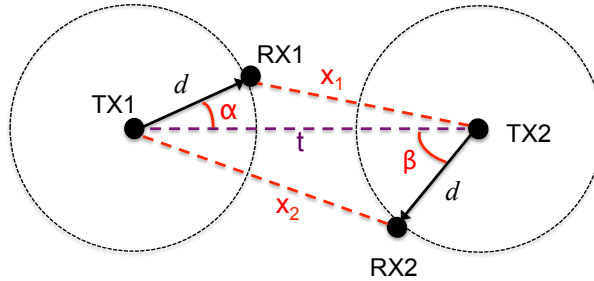
Figure 6.20: 2–player topology.
