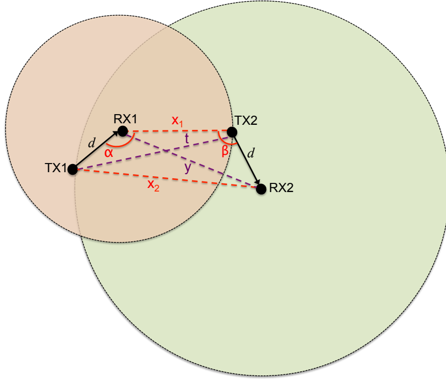
Figure 7.10: The coupling probability is proportional to the area of the non-overlapping green lune.
