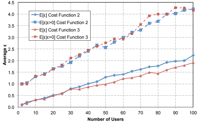
Figure 4.2: Average minimum value of \epsilon .
