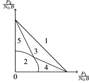
Figure 6.5: Optimal solution for the 2-user asymmetric flat case [4].
