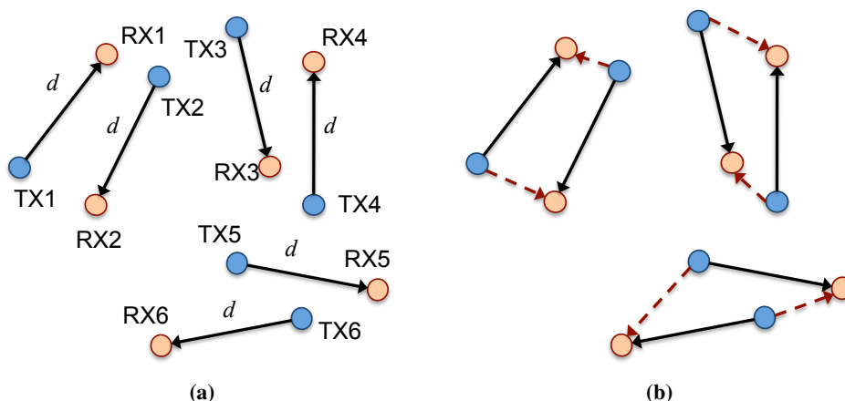
Figure 7.5: Example of a 6-player game (a) with the associated directed influence graph (b).
