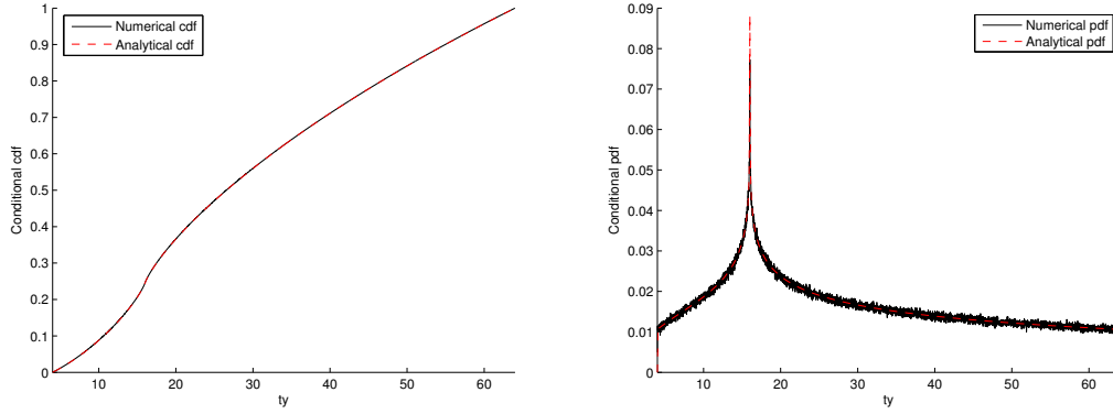
Figure 7.18: Conditional cdf (left) and pdf (right) of ty by simulation and with numerical evaluation of the integral when x_1 = 5 and d = 3 .
