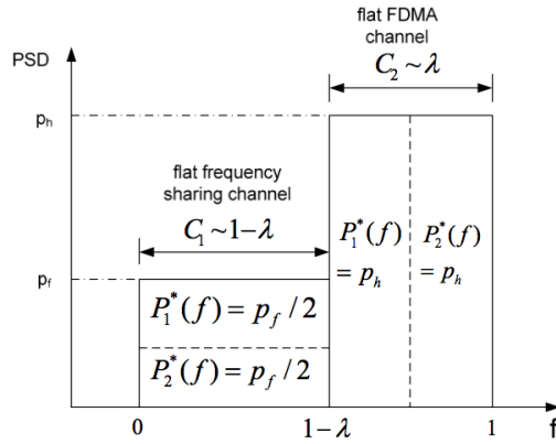
Figure 6.4: Mixed scheme to achieve the optimal solution when p_f < p < p_h [2].
