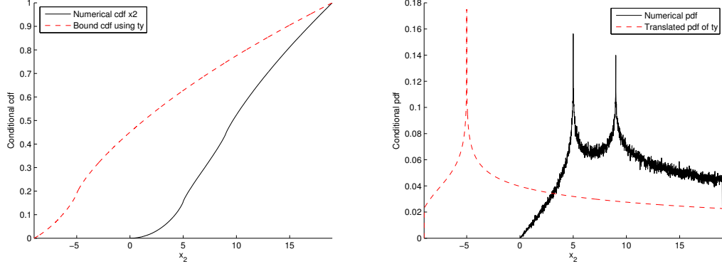
Figure 7.22: Conditional cdf (left) and pdf (right) of x_2 by simulation when x_1 = 5 and d = 7 .
