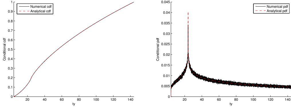
Figure 7.19: Conditional cdf (left) and pdf (right) of ty by simulation and with numerical evaluation of the integral when x_1 = 5 and d = 7 .
