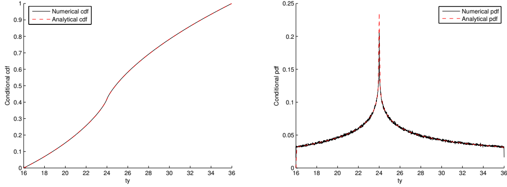
Figure 7.17: Conditional cdf (left) and pdf (right) of ty by simulation and with numerical evaluation of the integral when x_1 = 5 and d = 1 .
