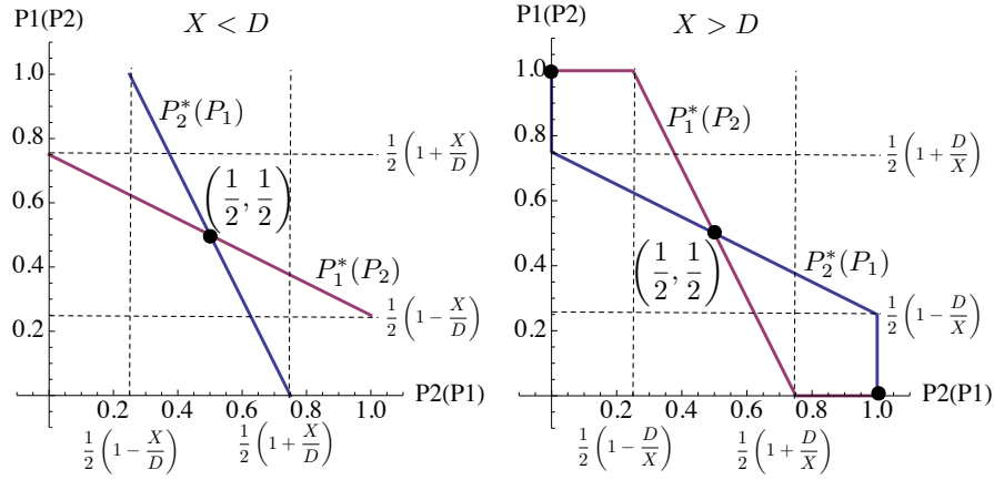
Figure 6.13: The intersection of the best response functions P_1^*(P_2), P_2^*(P_1) give the Nash equilibria. The set of equilibria depends upon X \lesseqgtr D .
