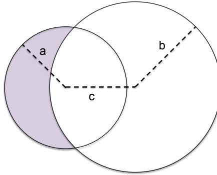
Figure 7.8: The colored area is the lune given by two circles of radius a and b , with b > a , whose centers are separated by c .
