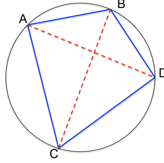
Figure 7.16: Ptolemy's theorem provides a relation among edges and diagonals in a cyclic quadrilateral.
