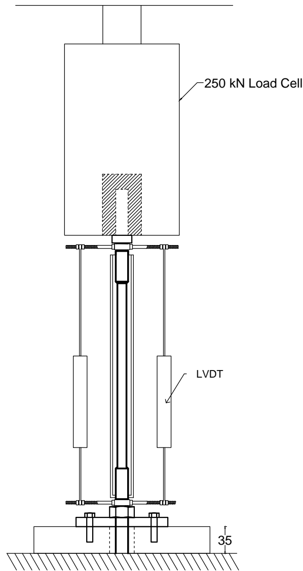
Tav. 1: Test Set up and Details of External Dissipator Devices Prepared
