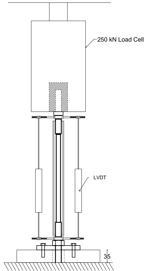
Tav. 2: Test Set up and Details of External Dissipator Devices to be Tested
