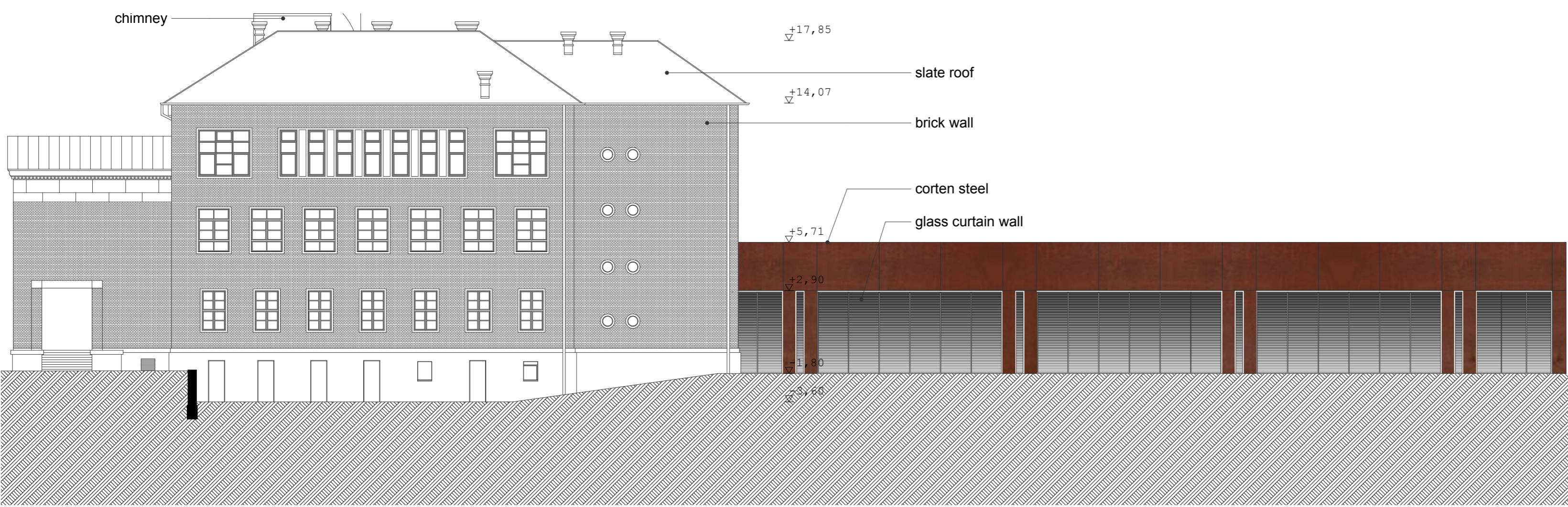
north facade
