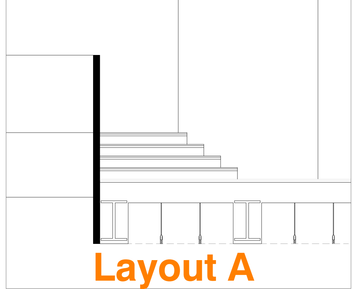
Layout A 1:20
