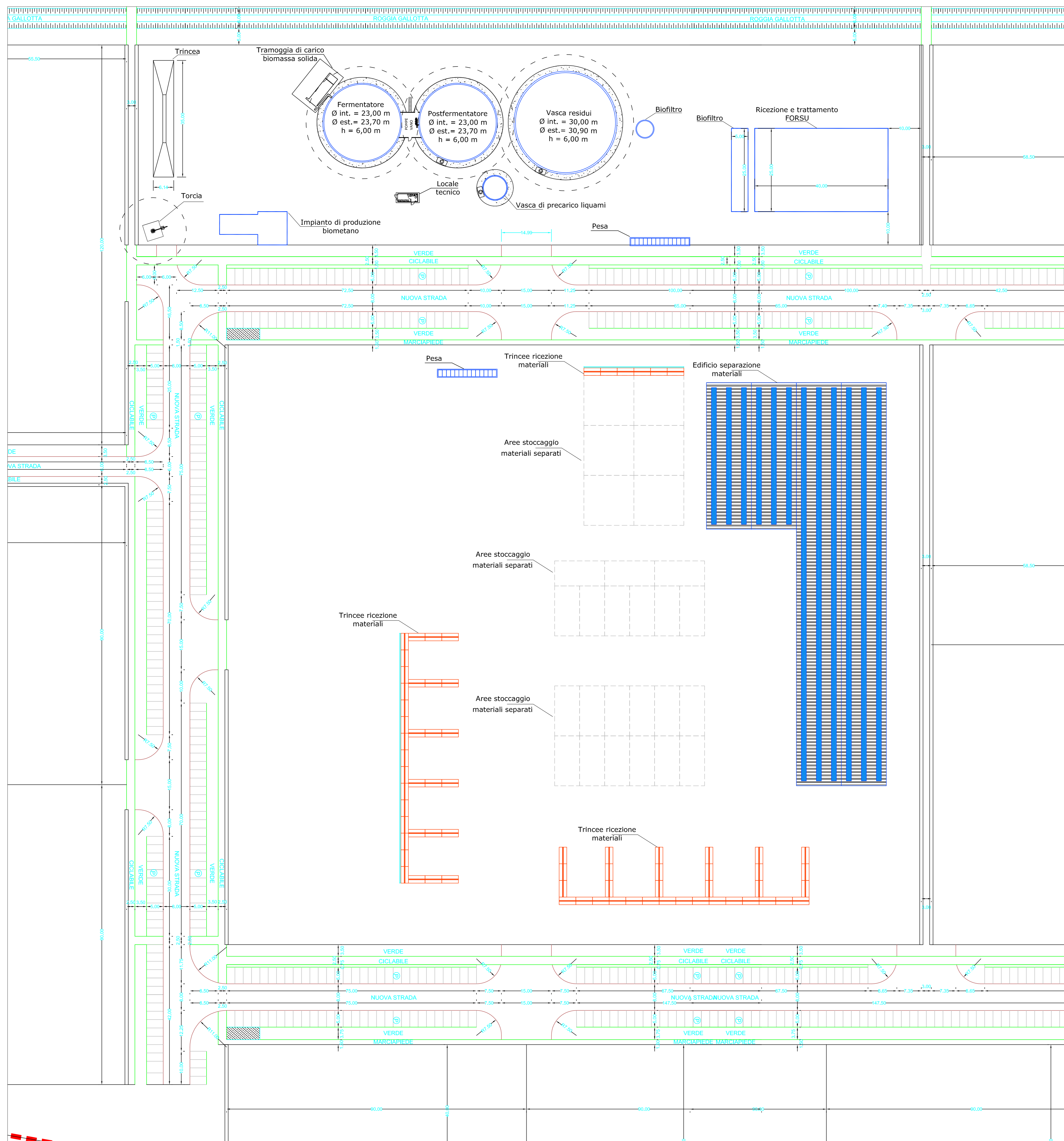
Layout-scala 1:500
