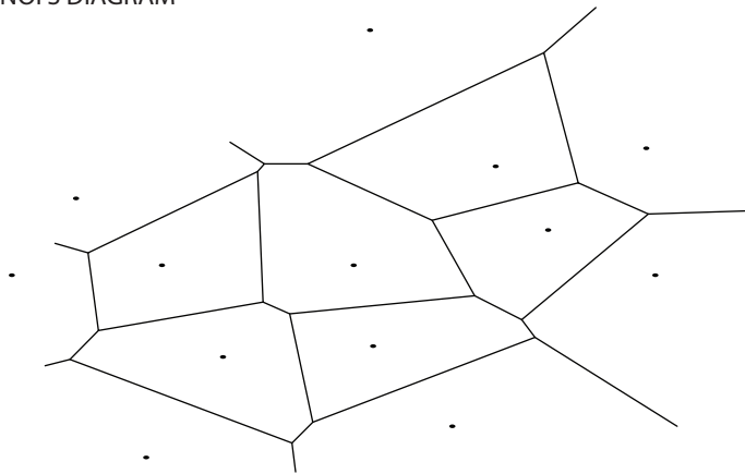
VORONOI'S DIAGRAM
