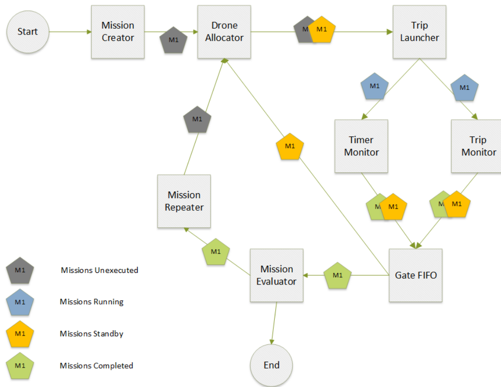
Figure 6.4: Pluto graph for the Alfa Crop Monitoring and Pollination application
