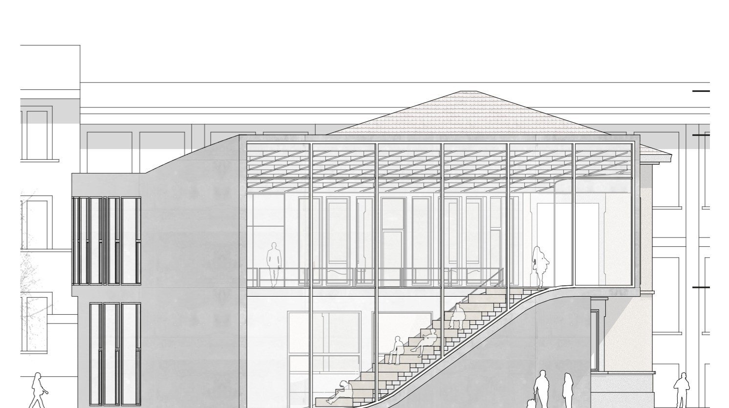
WEST ELEVATION
