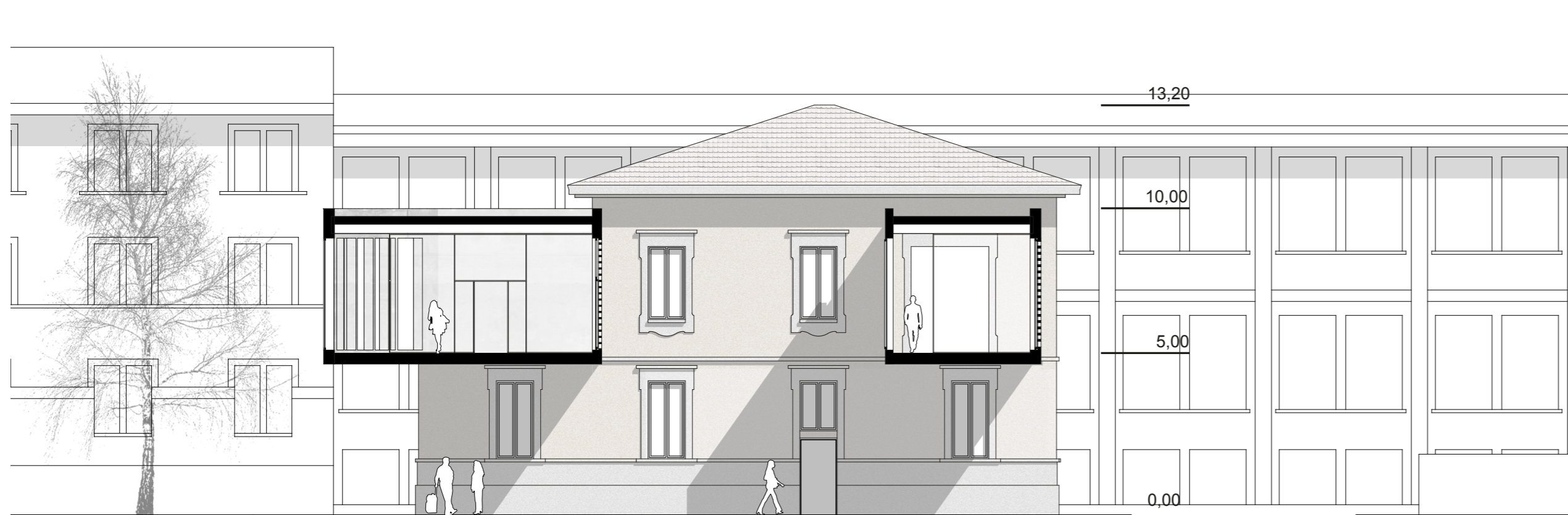
SECTION B-B
