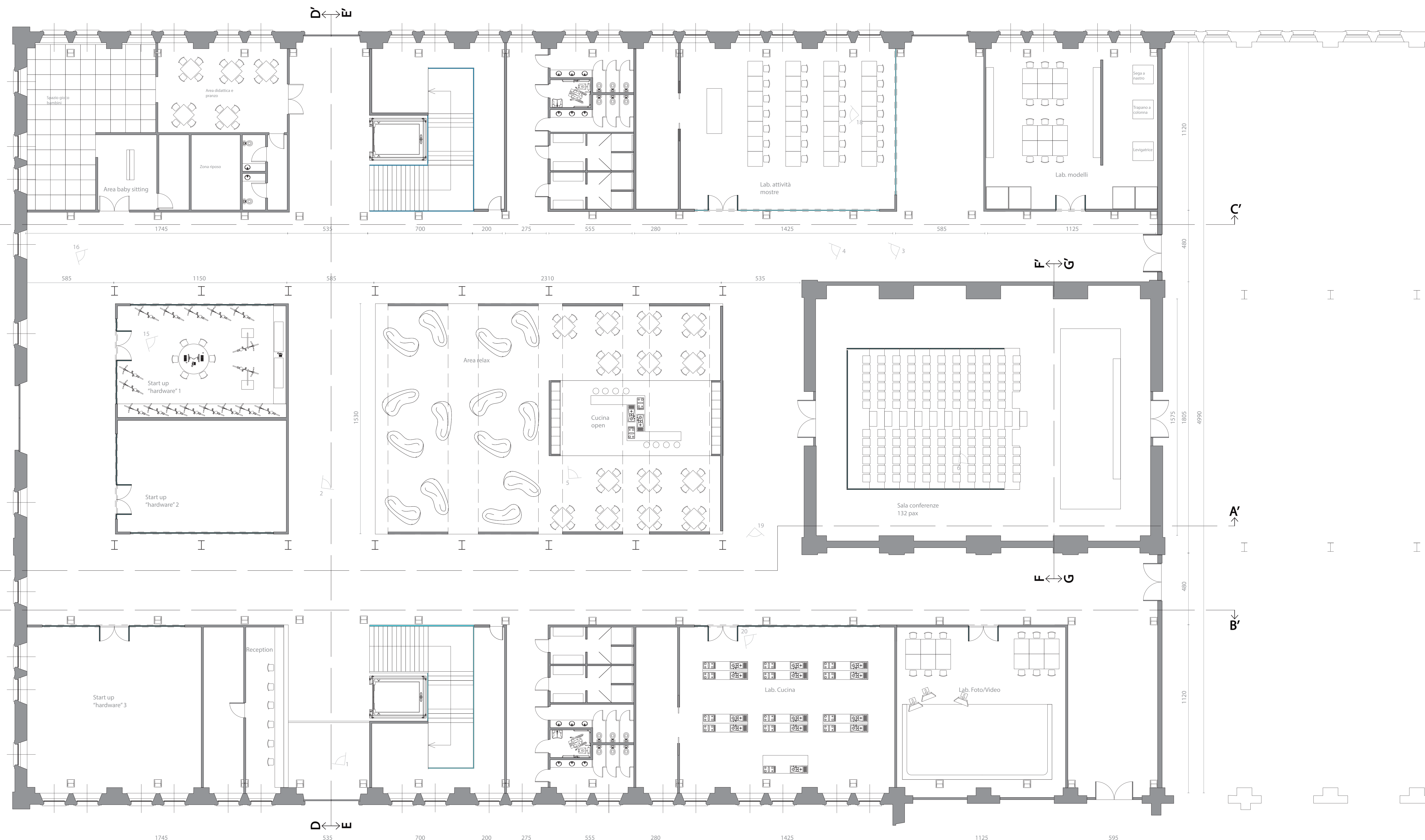
Pianta Piano 0 Scala 1:100 Quote in cm
