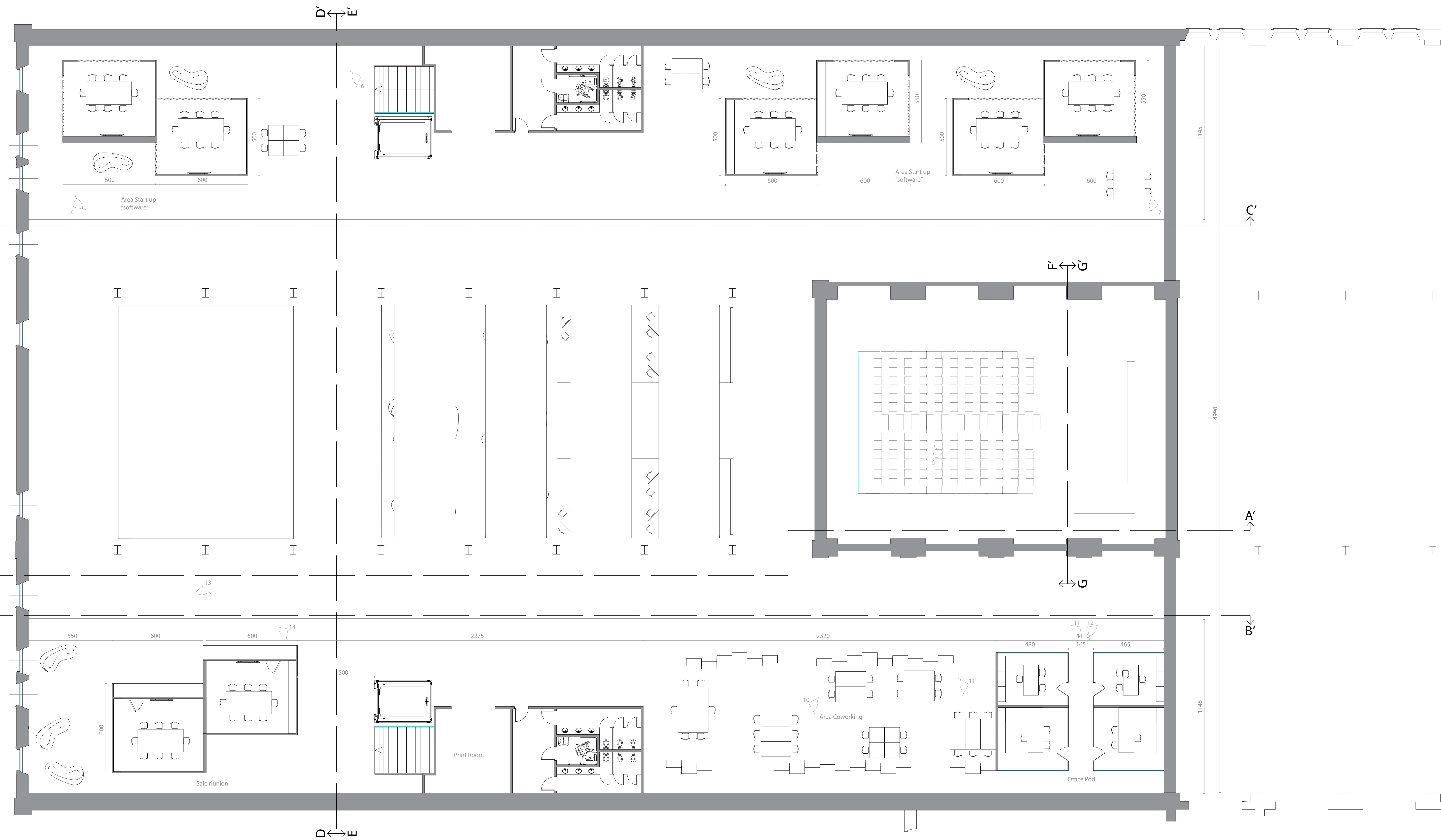
Pianta Piano +1 Scala 1:100 Quote in cm
