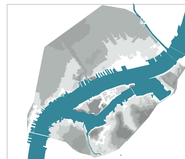
OROGRAPHIC CONFORMATION
