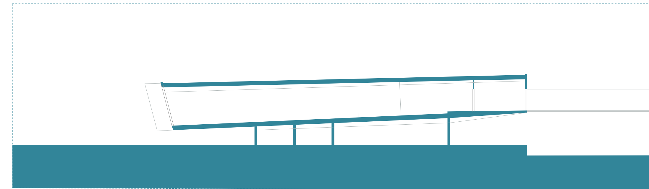
LONGITUDINAL SECTION OF THE AUDITORIUM
