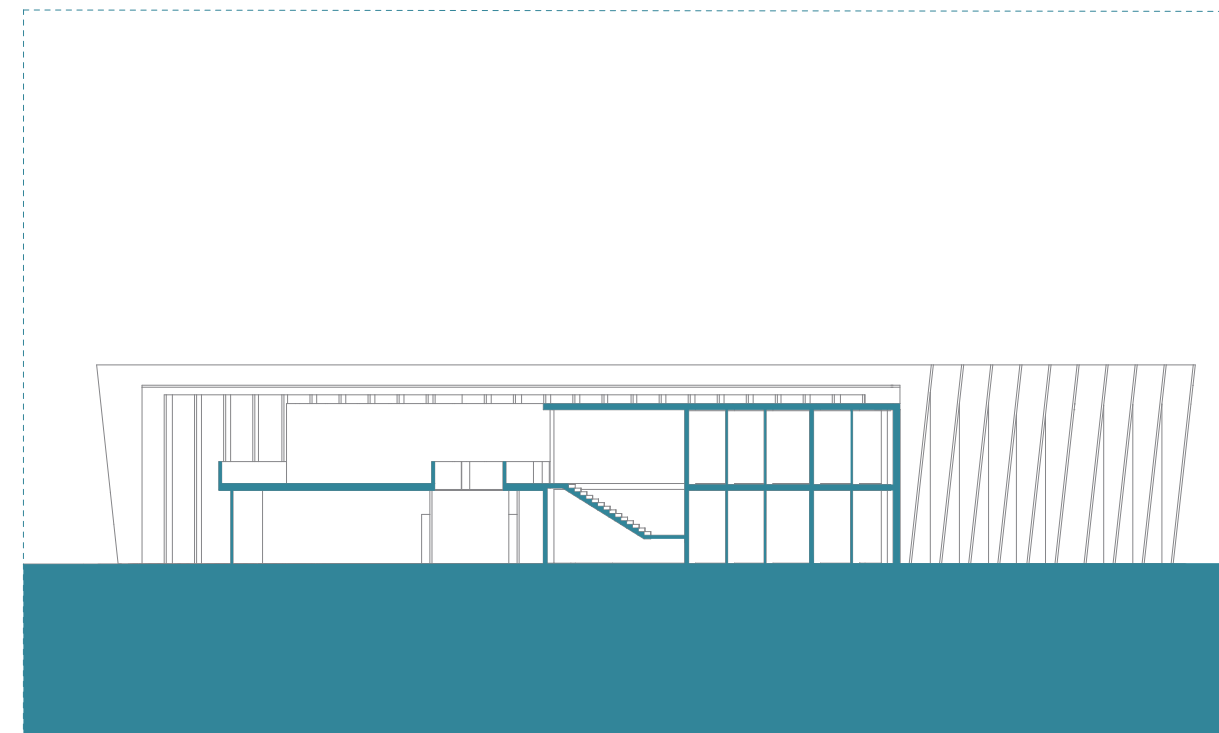
CROSS SECTION OF SERVICE BLOCK
