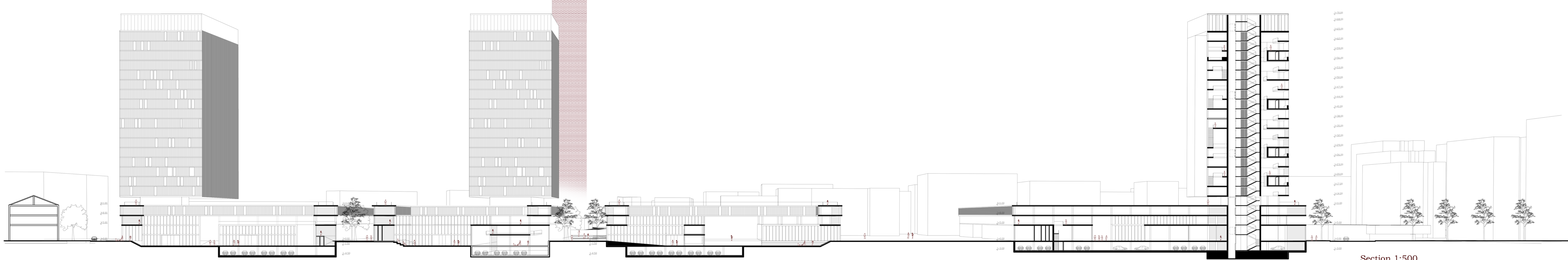
Section 1:500
