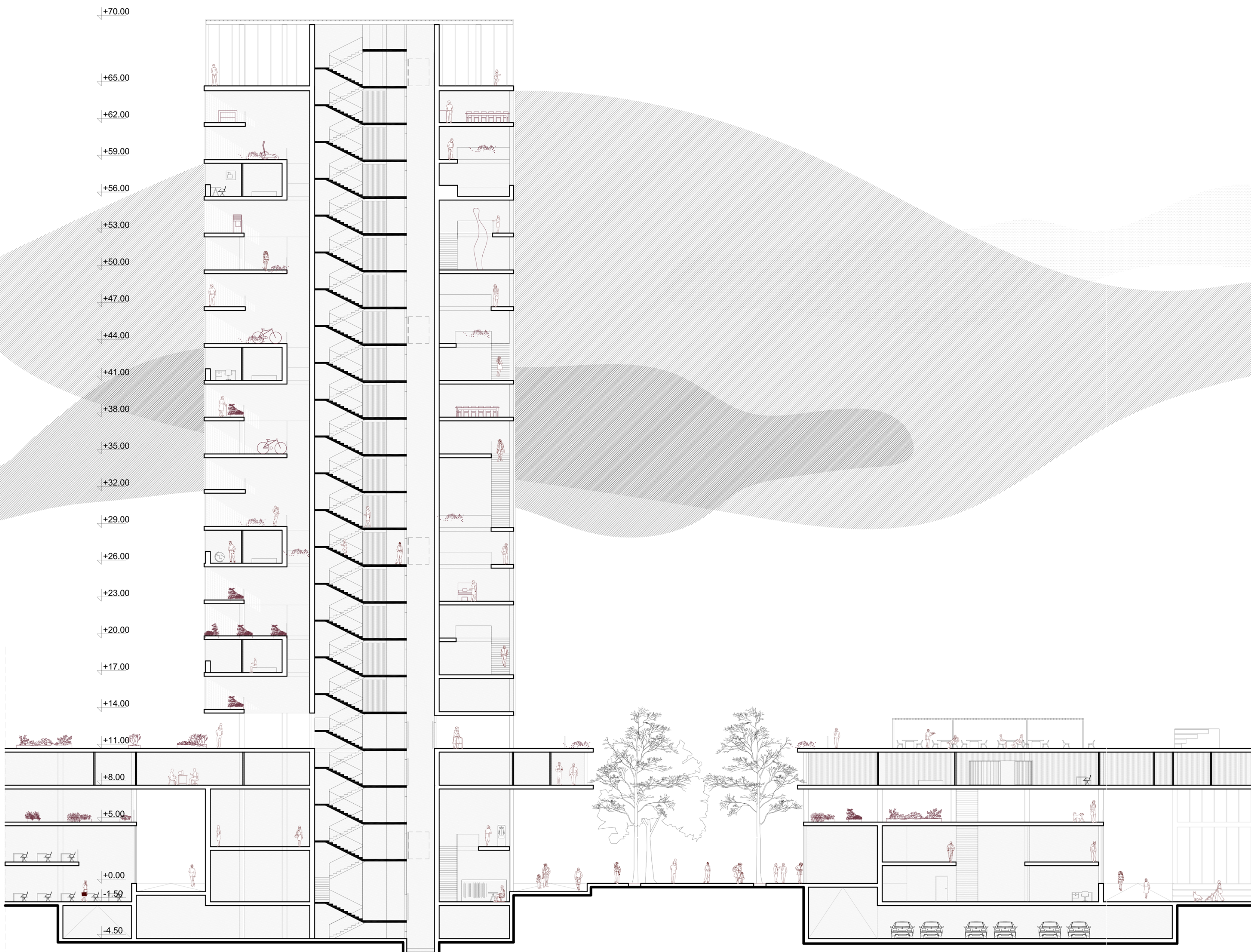
Section 1:200
