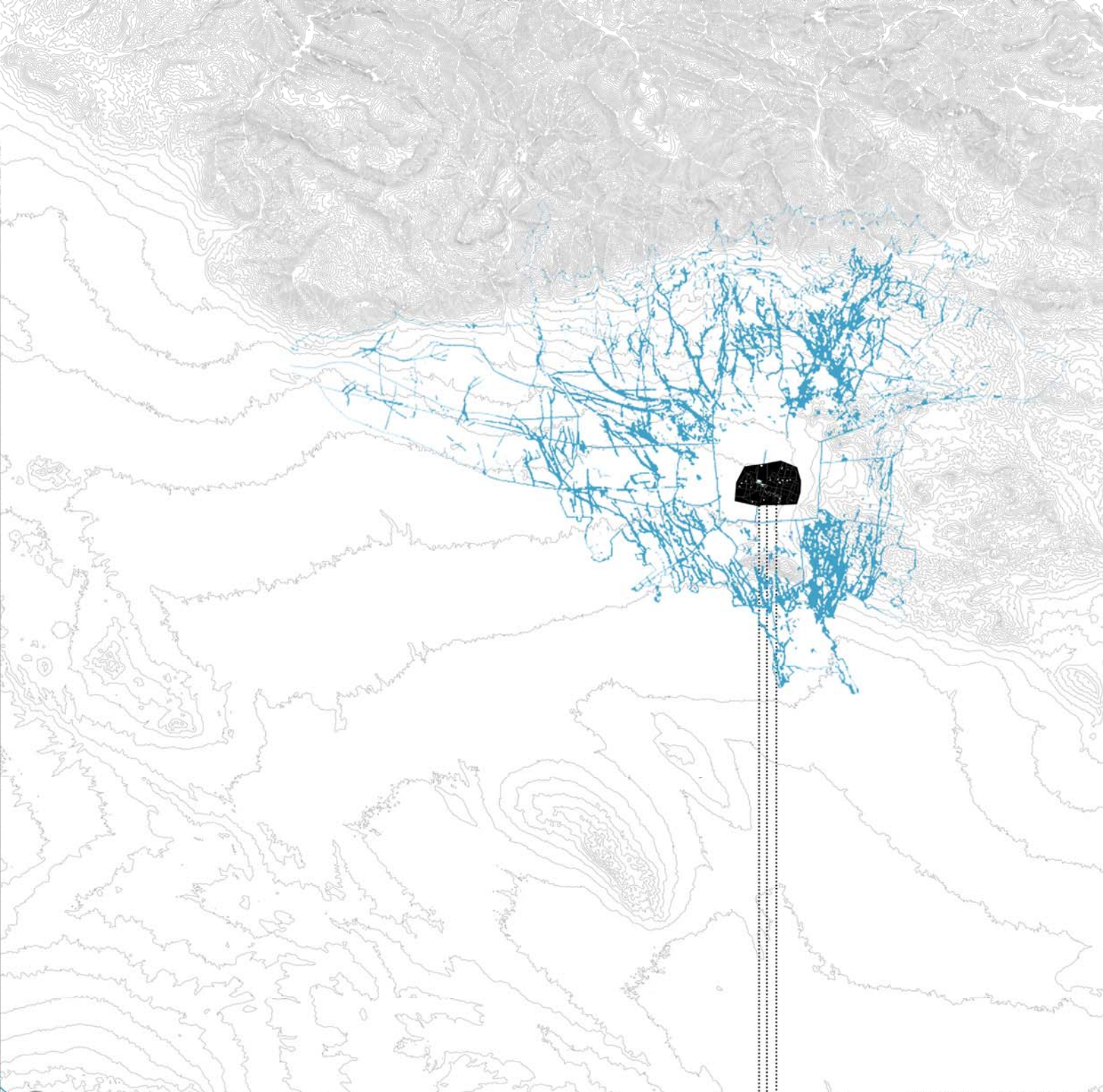
THE LOCATION OF THE FIRST CITY OF TEHRAN ACCORDING TO ITS UNDERGROUND WATER CANALS (QANAT)
