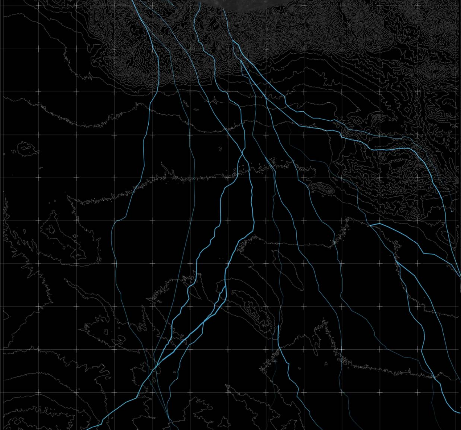
ROOTS OF TEHRAN UNDERGROUND WATER CANALS
