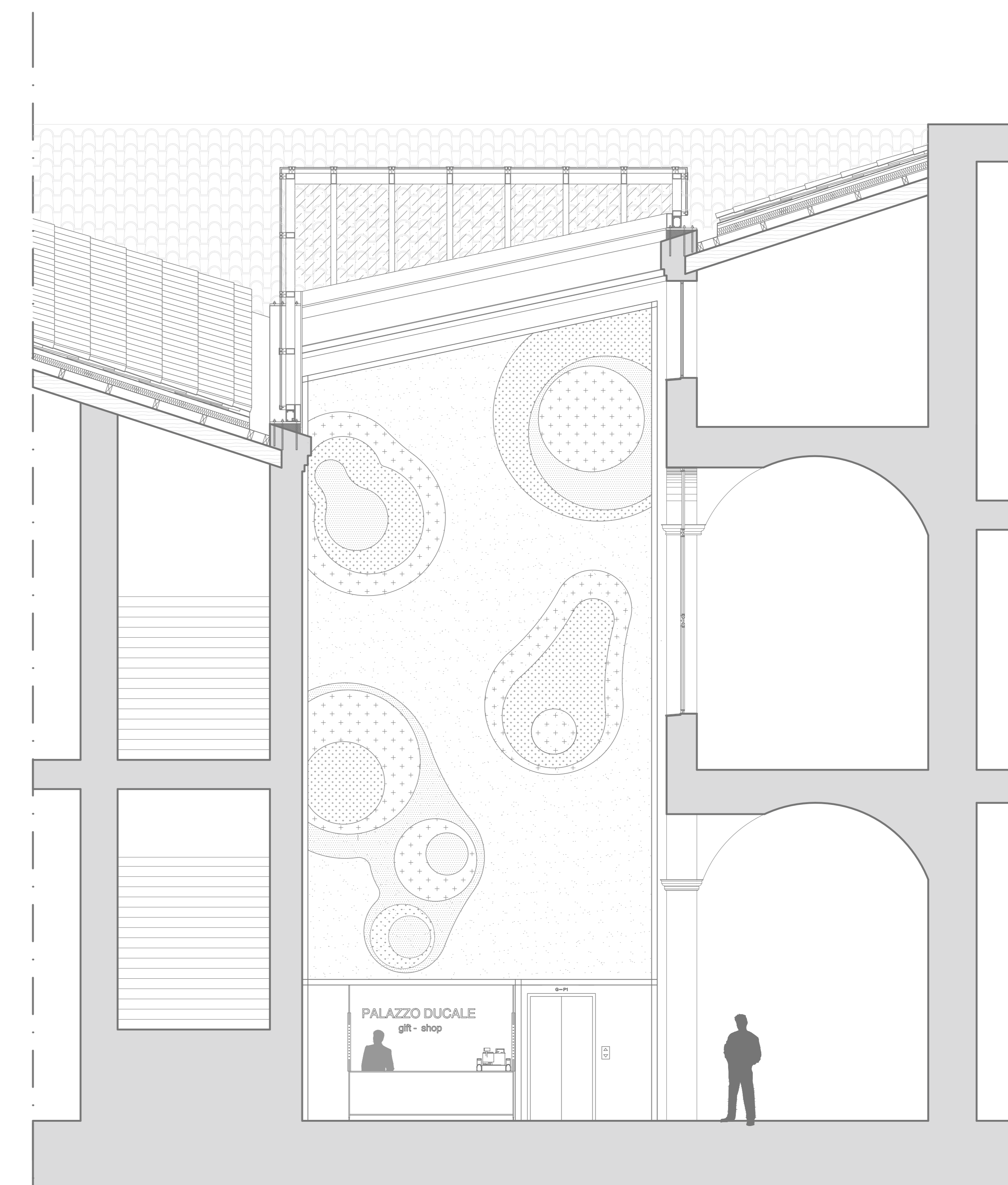
SECTION B-B SCALE 1:50
