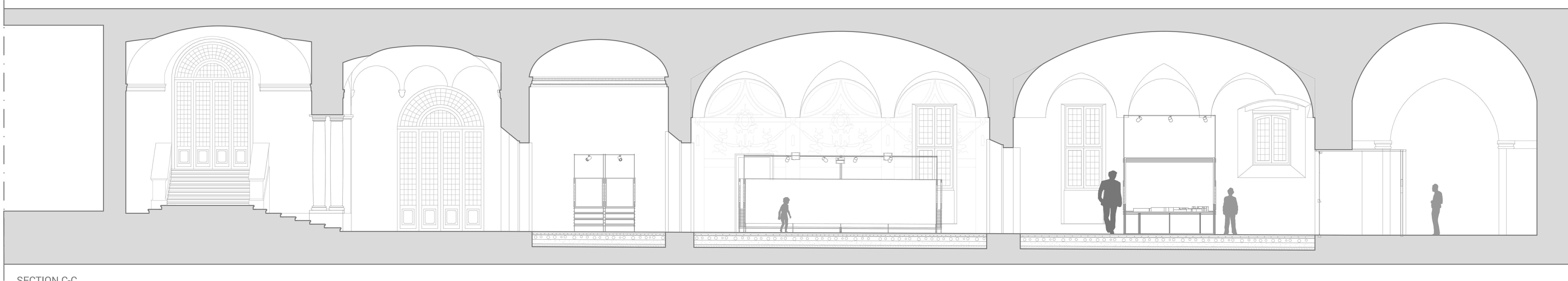
SECTION C-C SCALE 1:50
