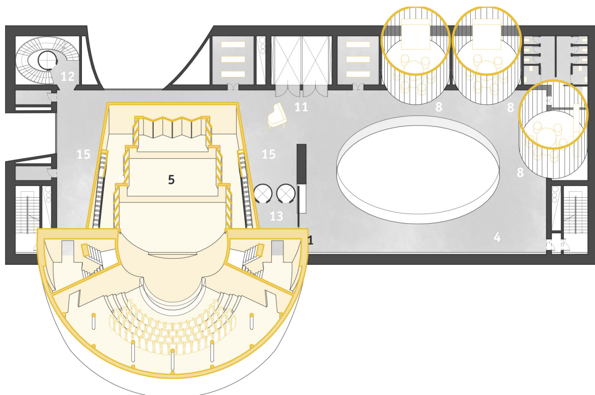
Pianta a quota +13,5m piano palco
