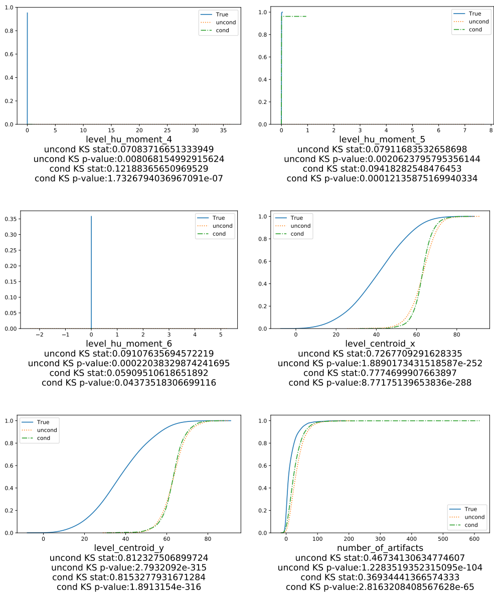
Figure B.3: Experiments 1 and 2: Cumulative distribution functions for true data, unconditional network and conditional network for each non-input feature.
