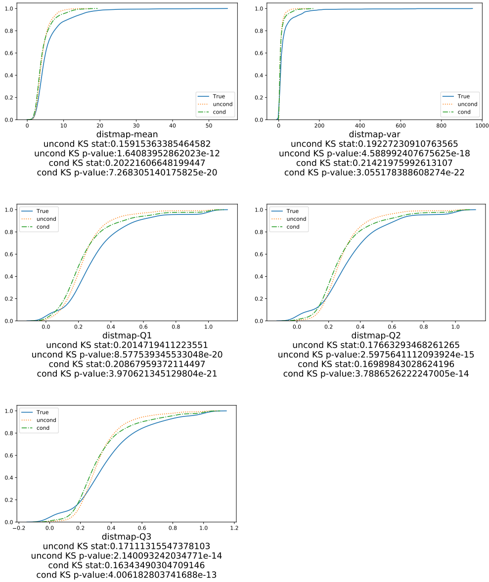
Figure B.11: Experiments 1 and 2: Cumulative distribution functions for true data, unconditional network and conditional network for each non-input feature.
