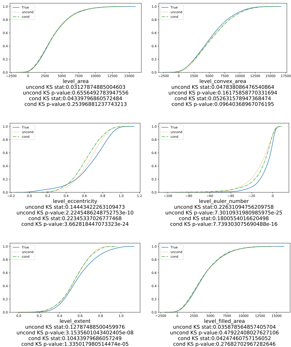
Figure B.1: Experiments 1 and 2: Cumulative distribution functions for true data, unconditional network and conditional network for each non-input feature.
