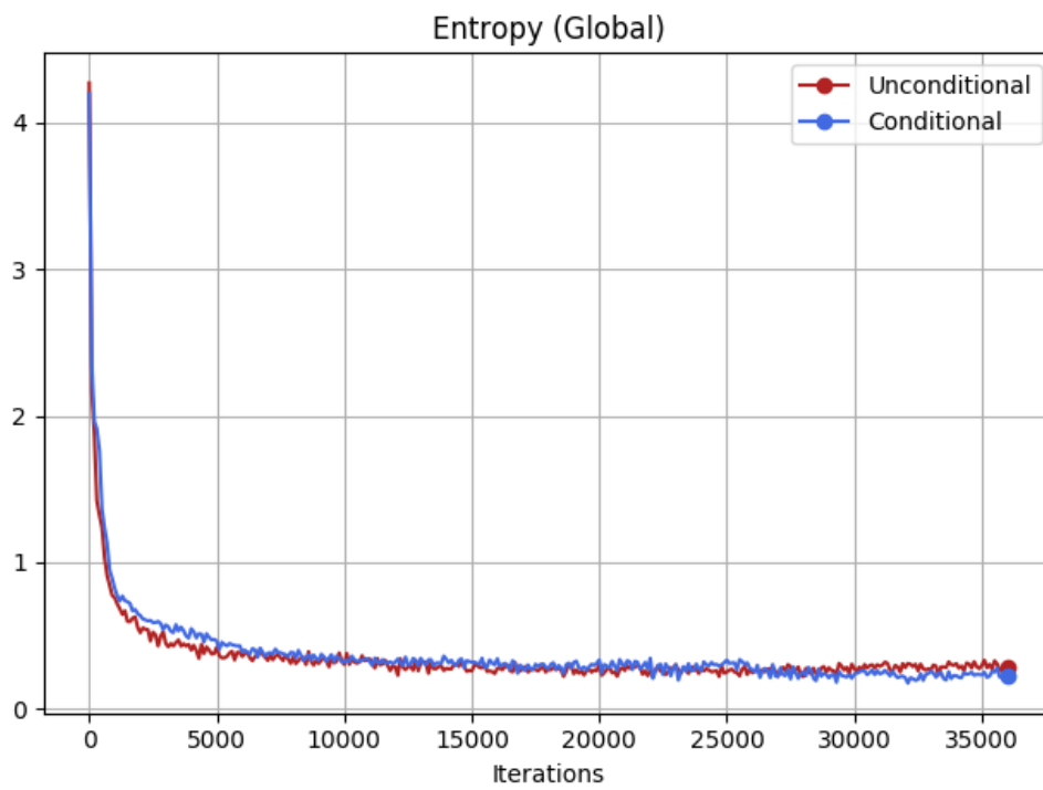
Figure 6.3: Sample Evaluation Metrics: Mean Entropy difference over all the maps (floormap, wallmap, thingsmap, heightmap). Unconditional (Red) and Conditional (Blue) networks generate samples having similar mean entropy.
