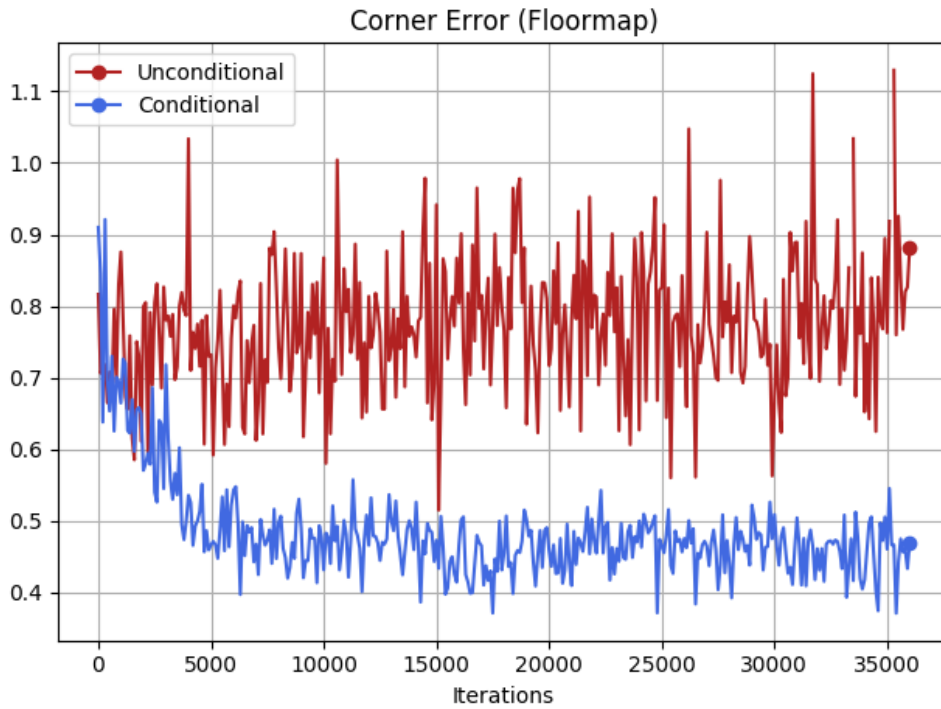
Figure 6.13: Sample Evaluation Metrics: Mean Corner Error over the FloorMap. Conditional (Blue) networks generate samples having a floor corner count closer to true levels than the Unconditional network (Red).
