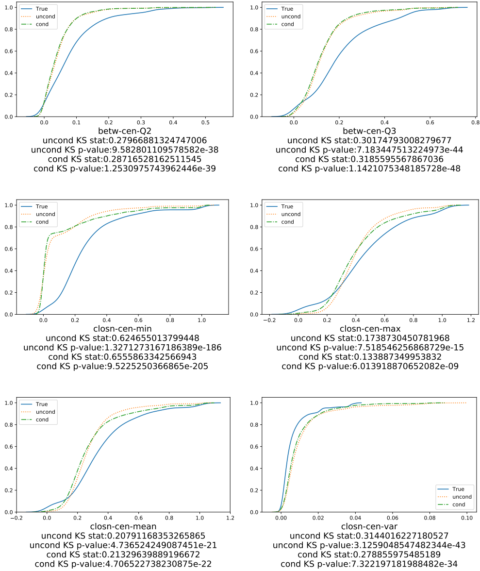
Figure B.9: Experiments 1 and 2: Cumulative distribution functions for true data, unconditional network and conditional network for each non-input feature.
