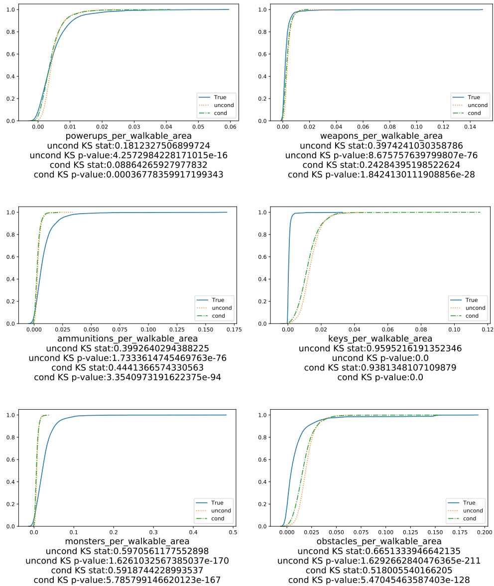
Figure B.6: Experiments 1 and 2: Cumulative distribution functions for true data, unconditional network and conditional network for each non-input feature.
