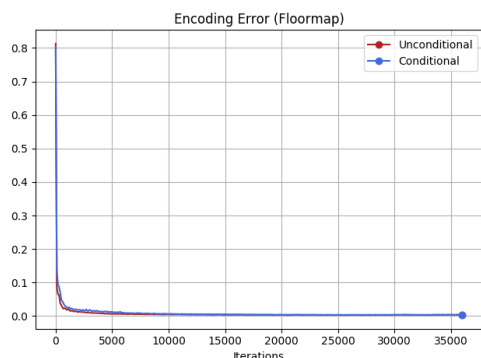
Figure 6.9: Sample Evaluation Metrics: Encoding Error calculated on FloorMap. Both Unconditional (Red) and Conditional (Blue) networks learn the colour scheme for representing the floors.
