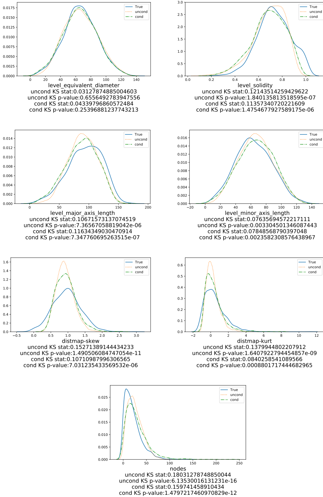
Figure 6.16: Experiments 1 and 2: Estimated probability density functions for true data, unconditional network and conditional network for each input feature.
