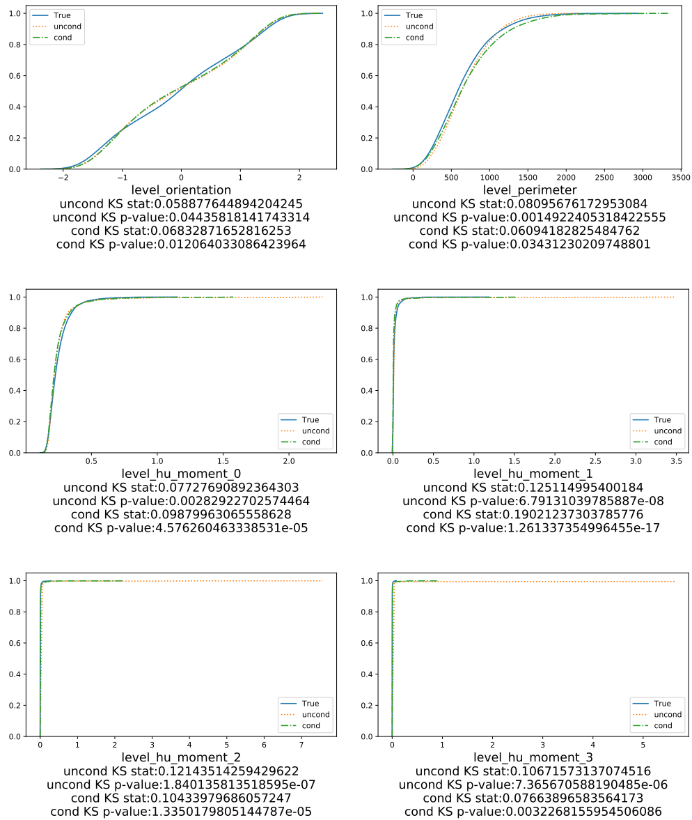
Figure B.2: Experiments 1 and 2: Cumulative distribution functions for true data, unconditional network and conditional network for each non-input feature.
