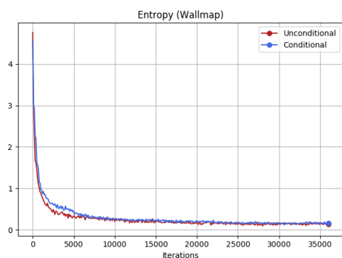
Figure 6.6: Sample Evaluation Metrics: Entropy MAE calculated on WallMap. Unconditional (Red) and Conditional (Blue) networks generate samples having similar WallMap entropy.
