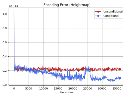
Figure 6.10: Sample Evaluation Metrics: Encoding Error calculated on HeightMap. Conditional (Blue) network is slightly more precise in representing the colour coding for the floor height than the Unconditional network (Red).
