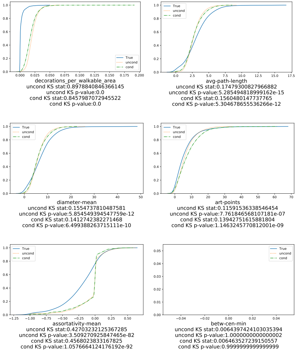
Figure B.7: Experiments 1 and 2: Cumulative distribution functions for true data, unconditional network and conditional network for each non-input feature.
