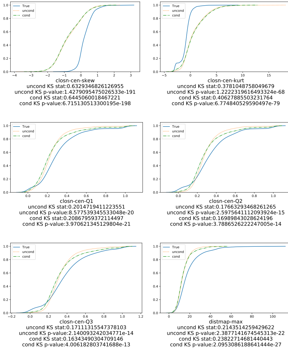
Figure B.10: Experiments 1 and 2: Cumulative distribution functions for true data, unconditional network and conditional network for each non-input feature.
