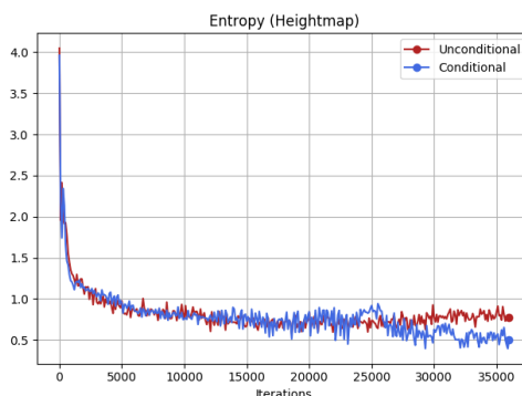
Figure 6.5: Sample Evaluation Metrics: Entropy MAE calculated on HeightMap. Conditional (Blue) network generate samples having slightly better HeightMap entropy than the Unconditional network (Red).
