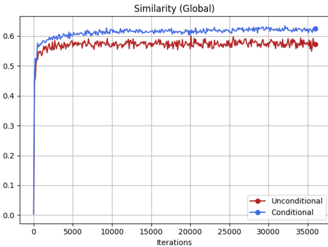
Figure 6.8: Sample Evaluation Metrics: Mean Structural Similarity over the samples. Conditional (Blue) networks generate samples being more similar to true ones than the Unconditional network (Red).
