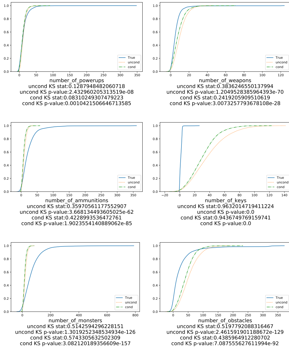
Figure B.4: Experiments 1 and 2: Cumulative distribution functions for true data, unconditional network and conditional network for each non-input feature.
