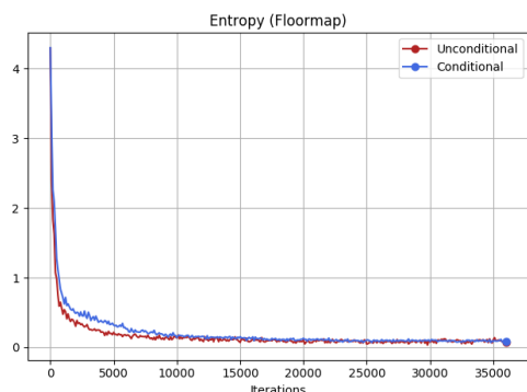
Figure 6.4: Sample Evaluation Metrics: Entropy MAE calculated on FloorMap. Unconditional (Red) and Conditional (Blue) networks generate samples having similar Floormap entropy.
