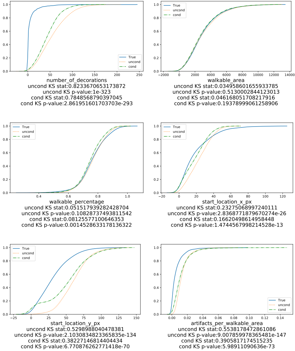
Figure B.5: Experiments 1 and 2: Cumulative distribution functions for true data, unconditional network and conditional network for each non-input feature.
