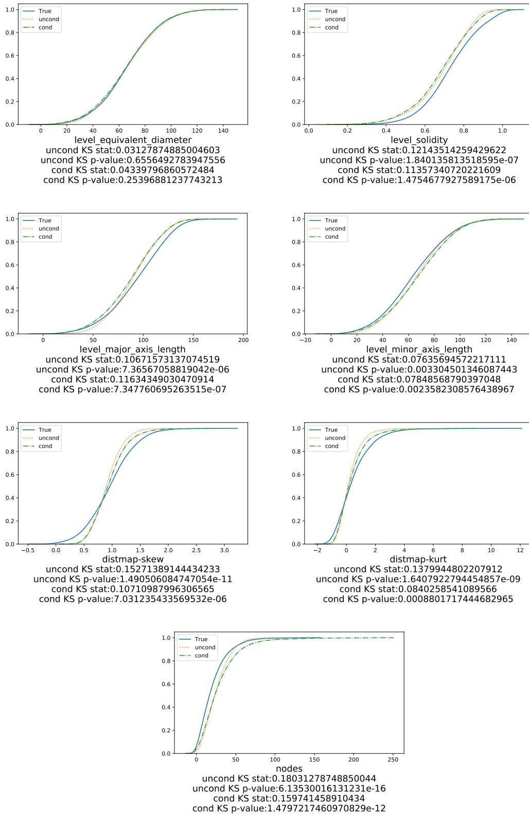
Figure 6.15: Experiments 1 and 2: Cumulative distribution functions for true data, unconditional network and conditional network for each input feature.
