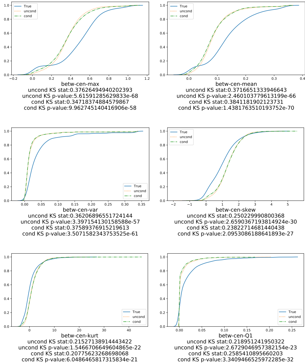
Figure B.8: Experiments 1 and 2: Cumulative distribution functions for true data, unconditional network and conditional network for each non-input feature.
