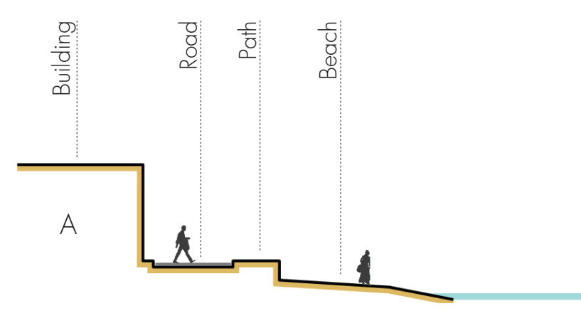
Schematic Section of Beaches 1, 2, 3
