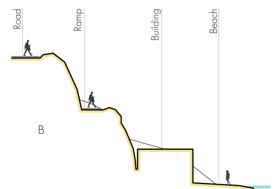
Schematic Section of Beaches 4, 5, 14, 16
