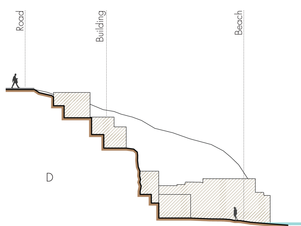
Schematic Section of Beach 6, 7
