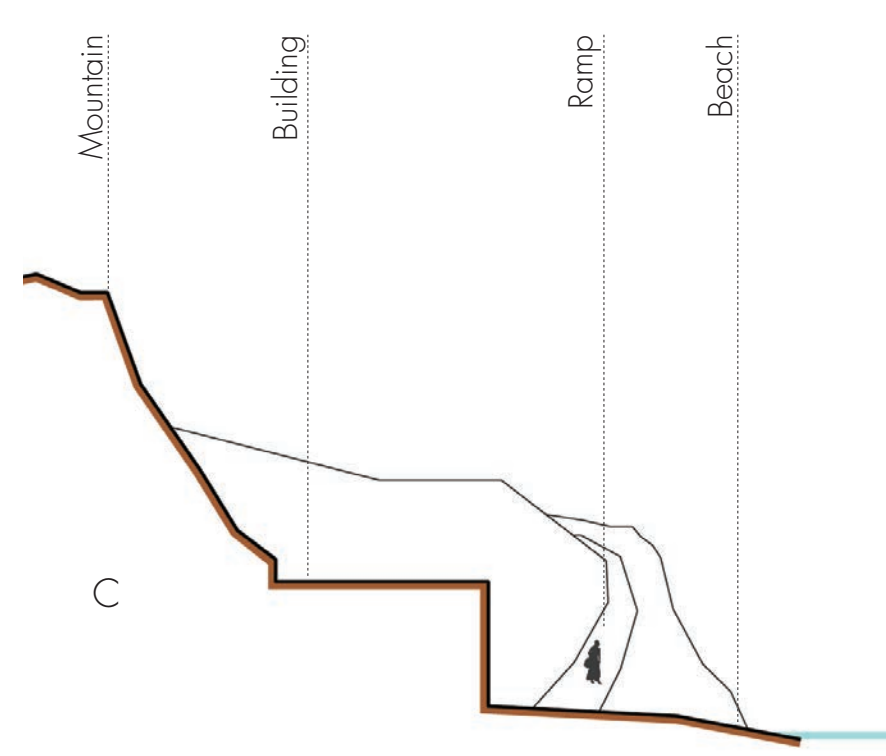
Schematic Section of Beach 8
