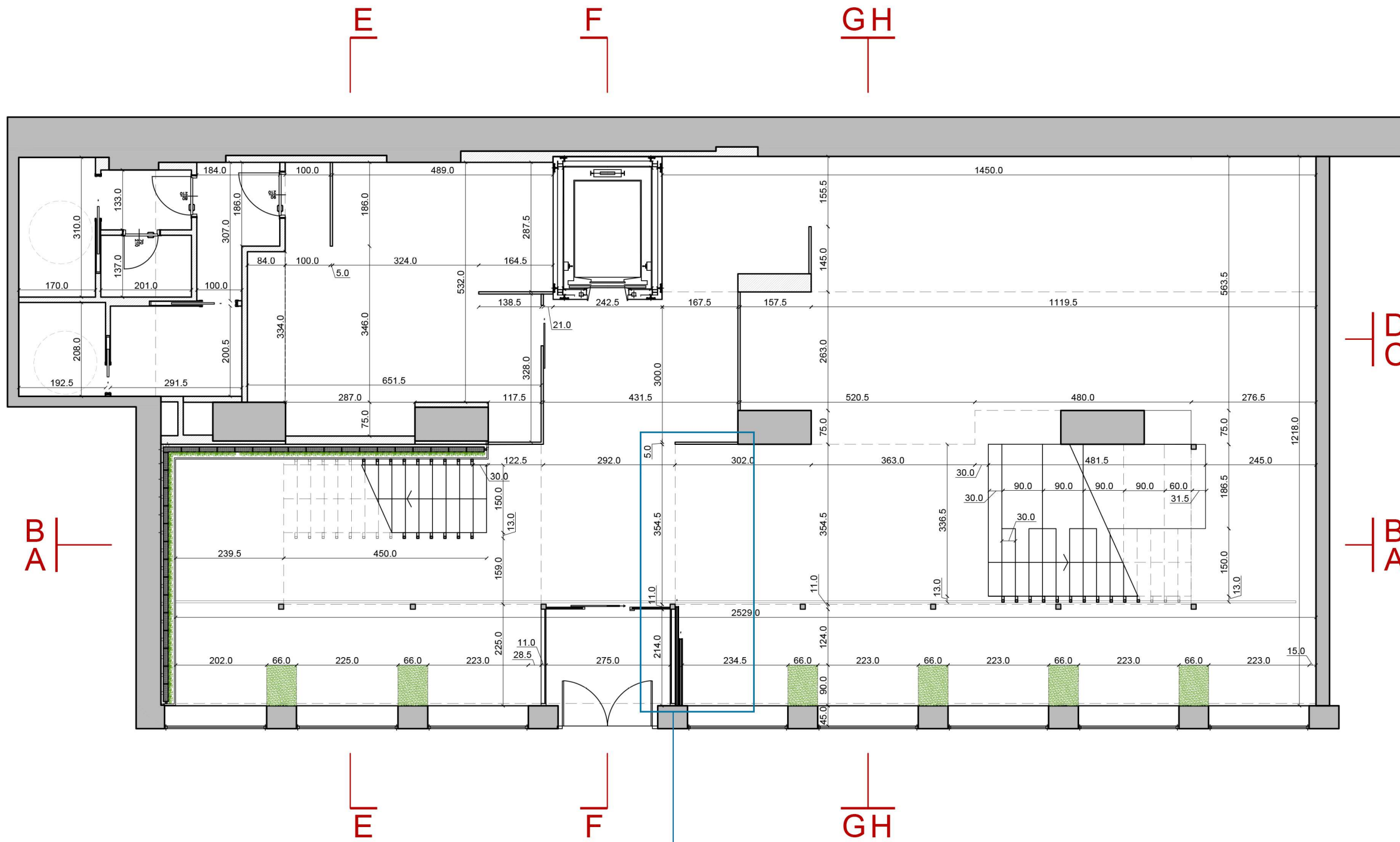
DETAIL 1: Moveable partition for Cultural Events
