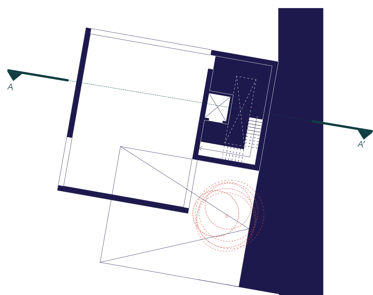
-0.75m Plan 1:200
