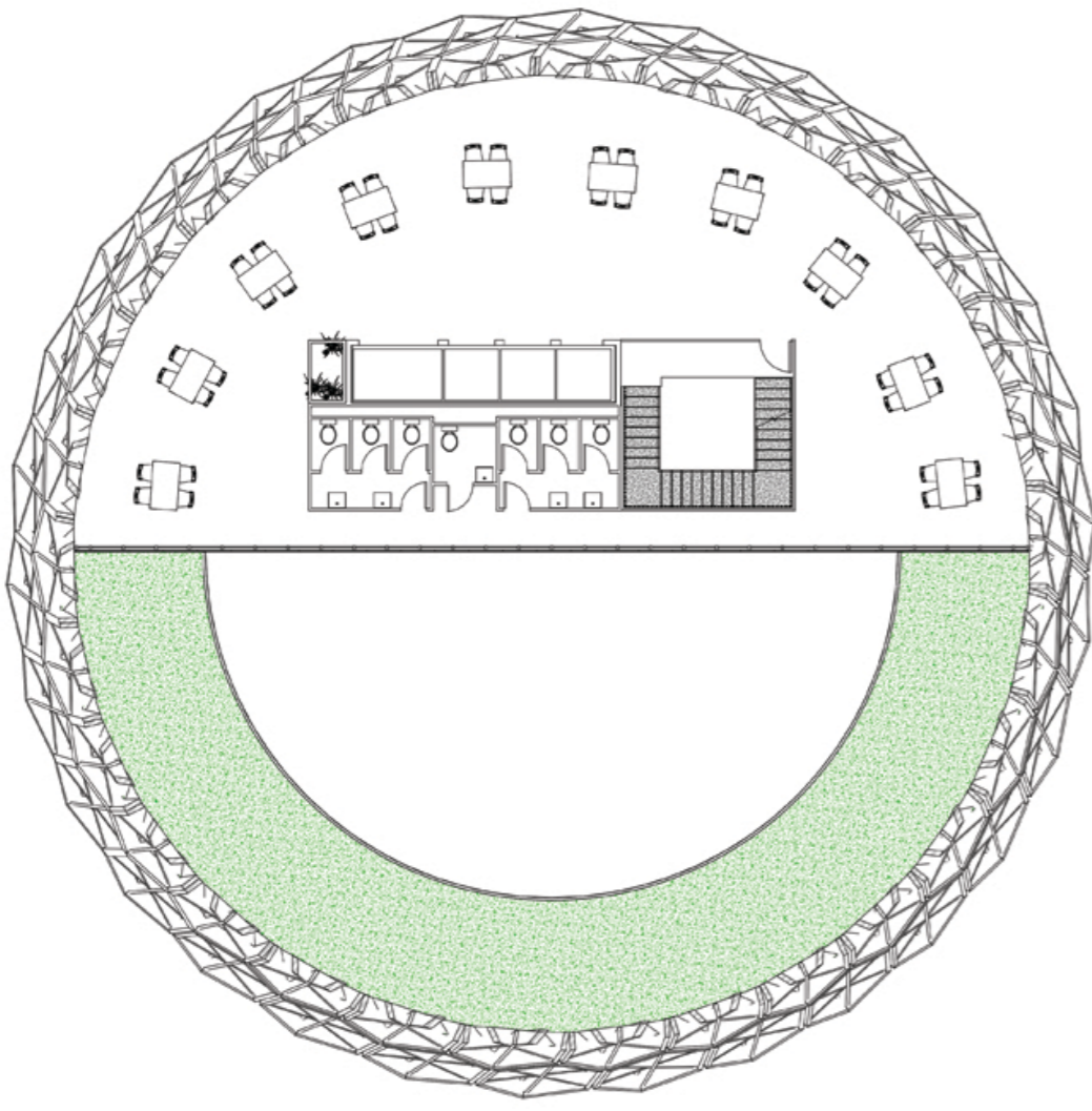
8th FLOOR PLAN Sc : 1/200
