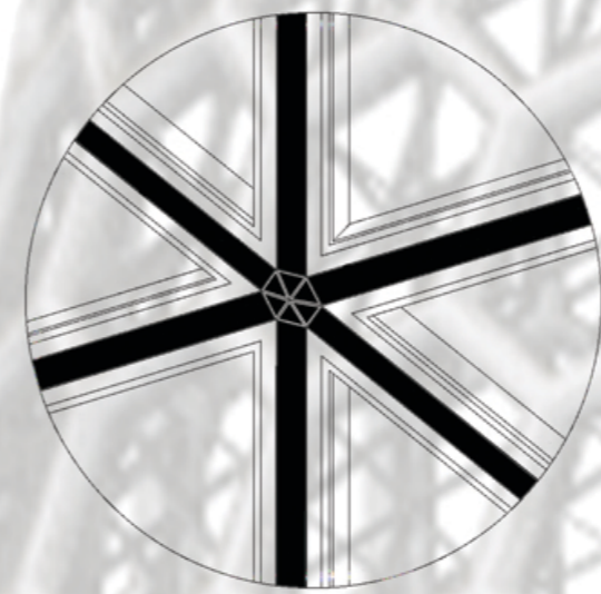
T Star Hub Middle 6 Branches 2D,3D Connections
