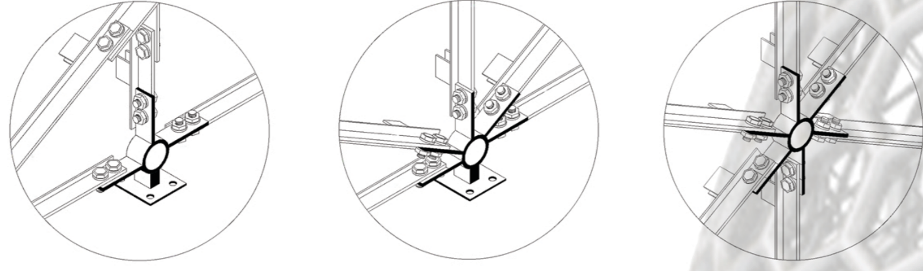
T Star Hub Ground 3 Branches 2D,3D Connections
