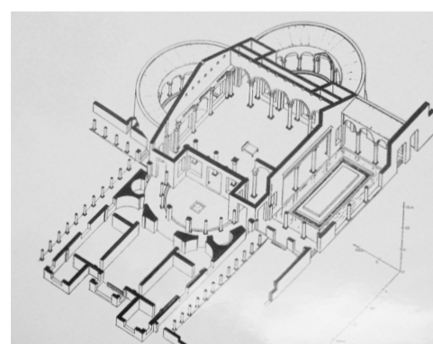
1 Arcaded Triclinium (W. MacDonald and J. Pinto)
