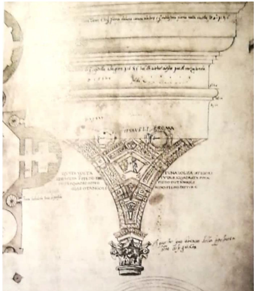
Drawing of the stucco ceiling of the Large Baths by Giuliano da Sangallo.
