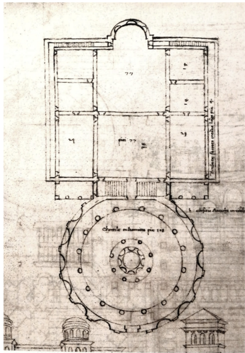
Plan of the Maritime Theatre and Greek Library. 'Clean copy' by Francesco di Giorgio Martini and his assistant.
