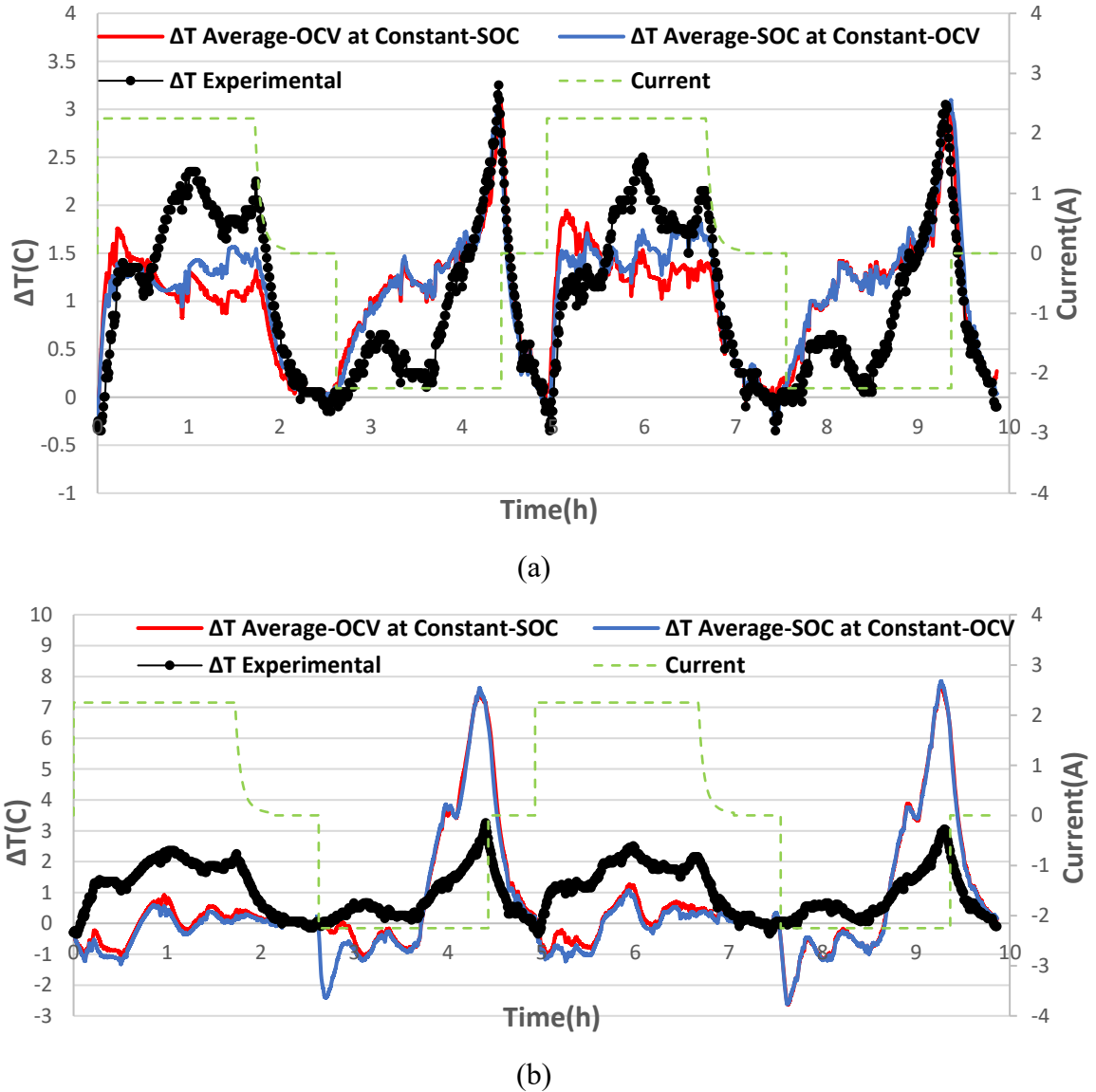
Figure 33 Illustration of the Simulated and Experimental Cell–Ambient Temperature Difference ( \Delta T ) with the Applied Current Profile at 0.5C-Rate: (a) Excluding the EHC and (b) Including the EHC.
