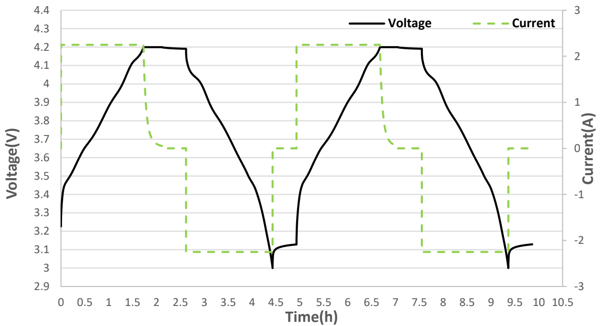
Figure 32 Experimental Voltage and Current Profiles at 0.5C-Rate.
