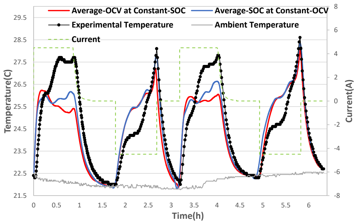
Figure A2 Experimental and Model-predicted Temperature Evolution During Cyclic Charge-discharge at 1C.
