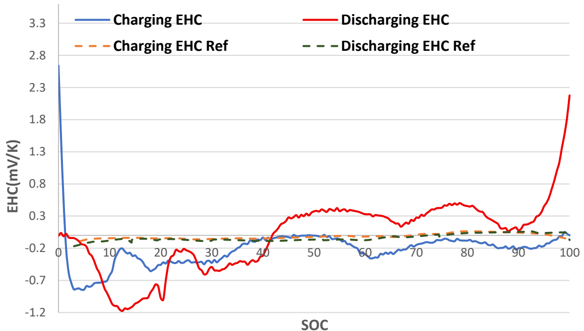
Figure 31 Charging vs. discharging entropic heat coefficient (EHC), including experimentally measured data and reference EHC from (Friedrich et al., 2022).
