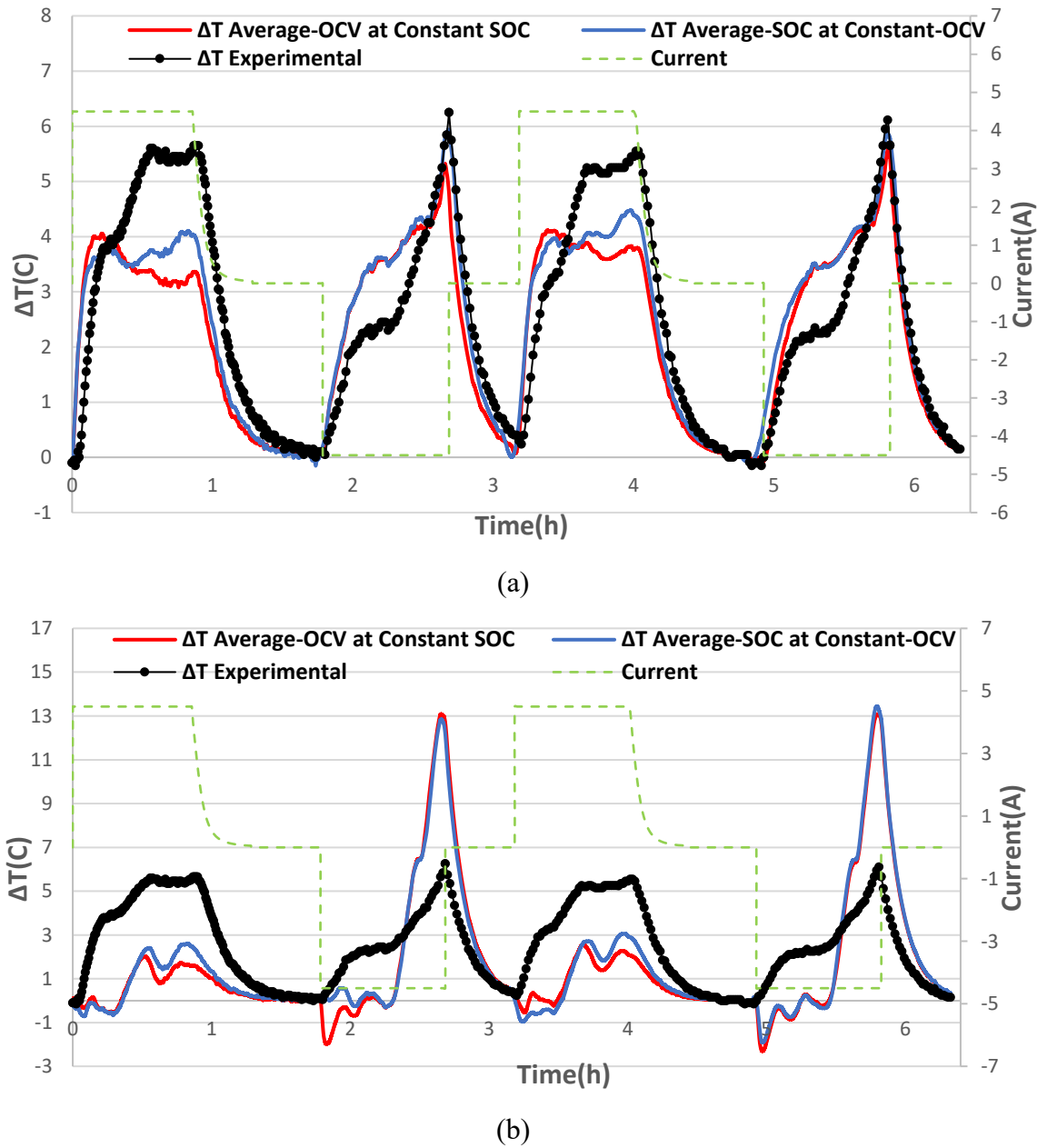
Figure 35 Illustration of the Simulated and Experimental Cell–Ambient Temperature Difference ( \Delta T ) with the Applied Current Profile at 1C-Rate: (a) Excluding the EHC and (b) Including the EHC.
