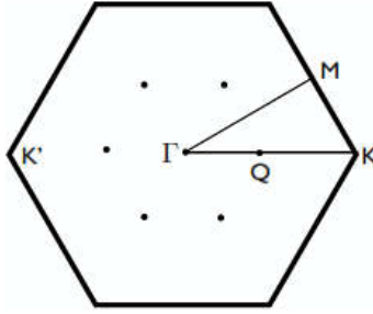
Figure 1.8. Two-dimensional Brillouin zone (BZ) of MX_2 . The high symmetry points \Gamma = (0,0) , K = 4\pi/3a(1,0) and M = 4\pi/3a(0,\sqrt{3}/2) are shown. The Q points (which are not high symmetry points) indicate the position of the edges of the conduction band in multi-layer samples.
