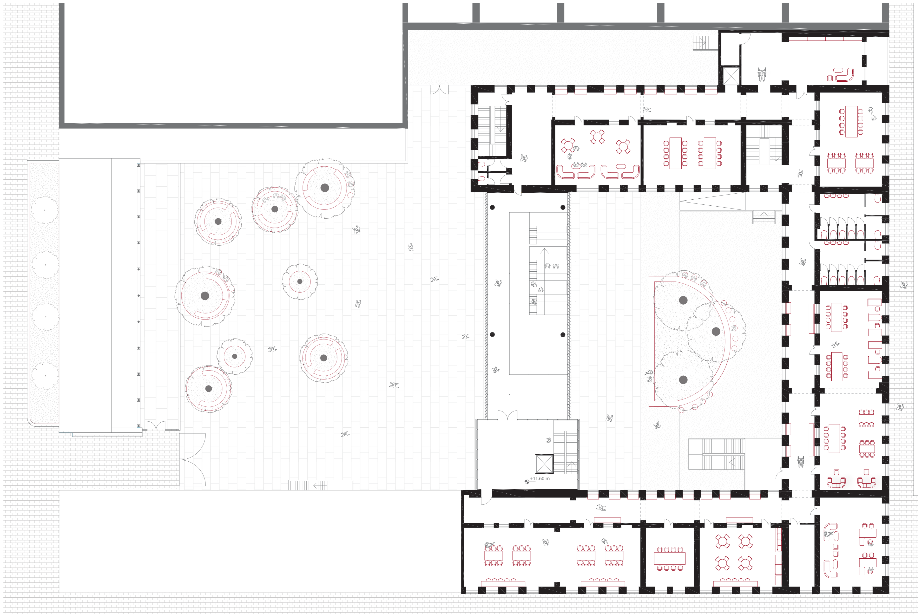
Second Floor 1:200
