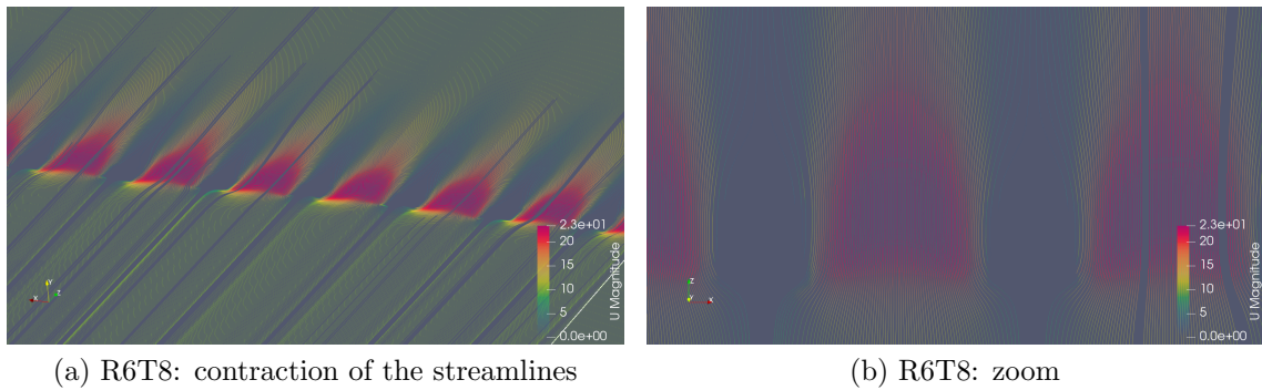
Figure 5: Velocity streamlines
