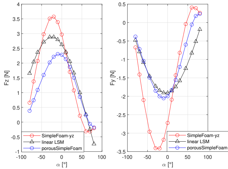
Figure 42: Stretched Screen: SimpleFoam, LSM and PorousSimpleFoam comparison - zy plane
