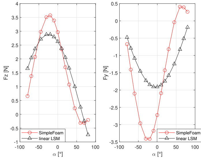
Figure 41: Stretched Screen: SimpleFoam and LSM - zy plane
