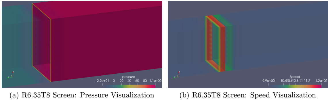
Figure 43: R6.35T8 screen: Channel Flow Visualizations
