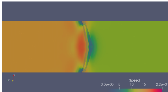
(a) Stretched Screen: Explicit Speed Visualization
